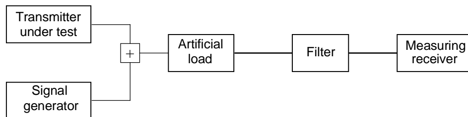
Figure 2: Measuring arrangement
