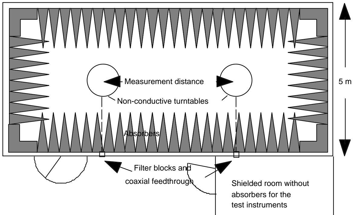
Ground plan
