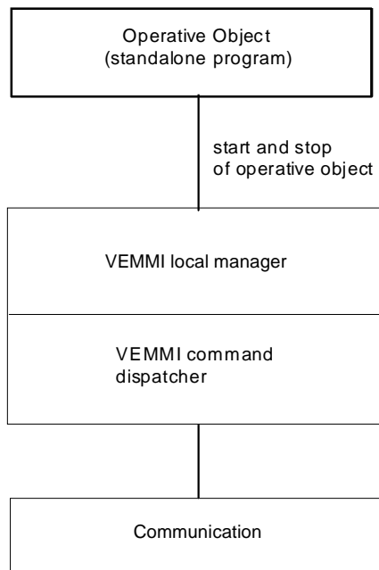
Figure 41: Standalone programs
