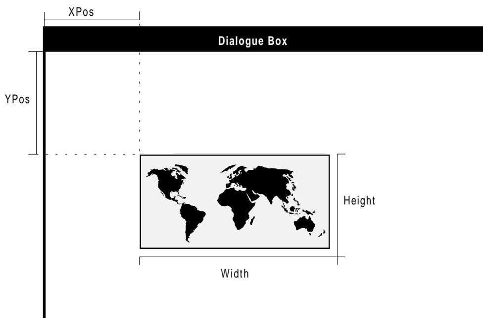
Figure 30a: Graphic output area featuring a bitmap and surrounded by a frame
