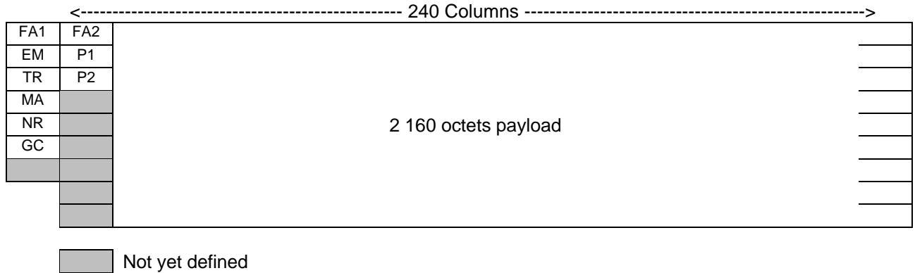
Figure C.1: Frame structure at 139 264 kbit/s
