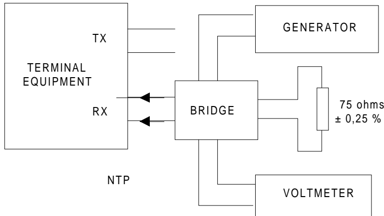
Figure A.5: Return loss at input port
