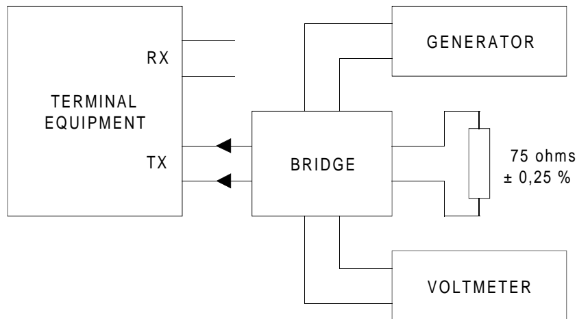
Figure A.6: Return loss at output port
