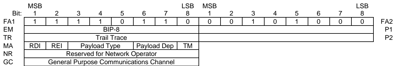
Figure C.2: Path overhead at 139 264 kbit/s
