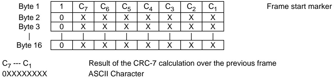
Figure C.3: 16-byte frame
