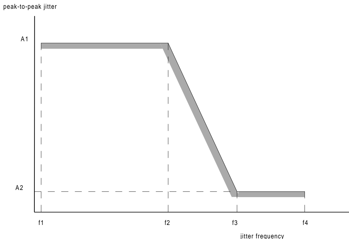
Figure 4: Input jitter tolerance
