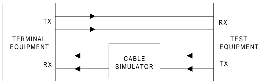
Figure A.4: Input coding and loss tolerance
