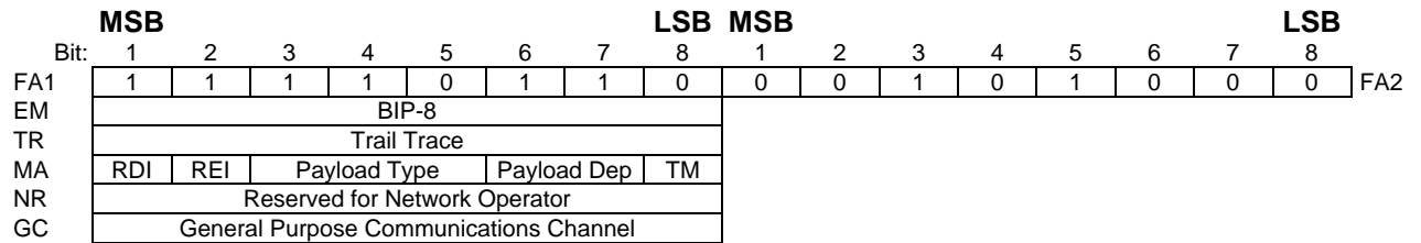
Figure C.2: Path overhead at 34 368 kbit/s
