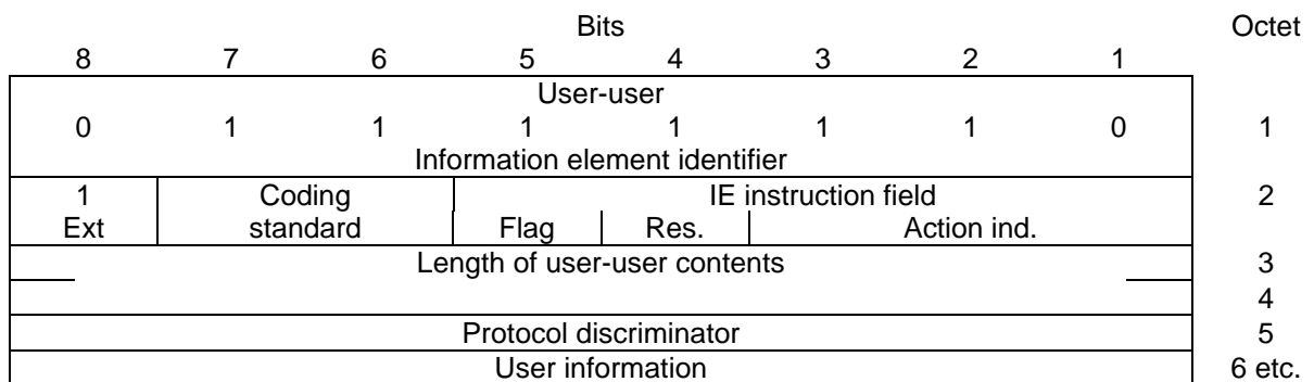
Figure 1-1: User-user information element
