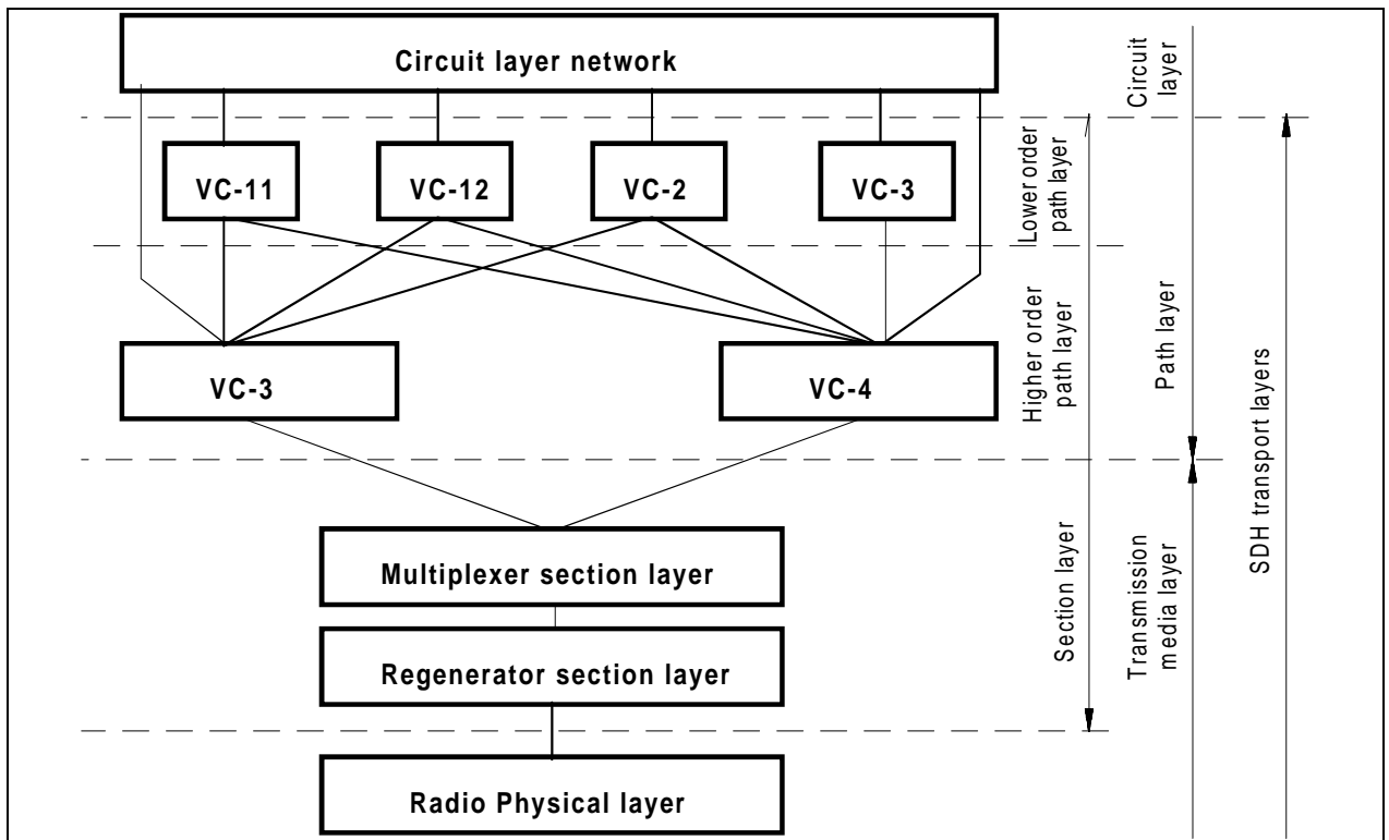
Figure C.1: SDH - based transport network layered model
