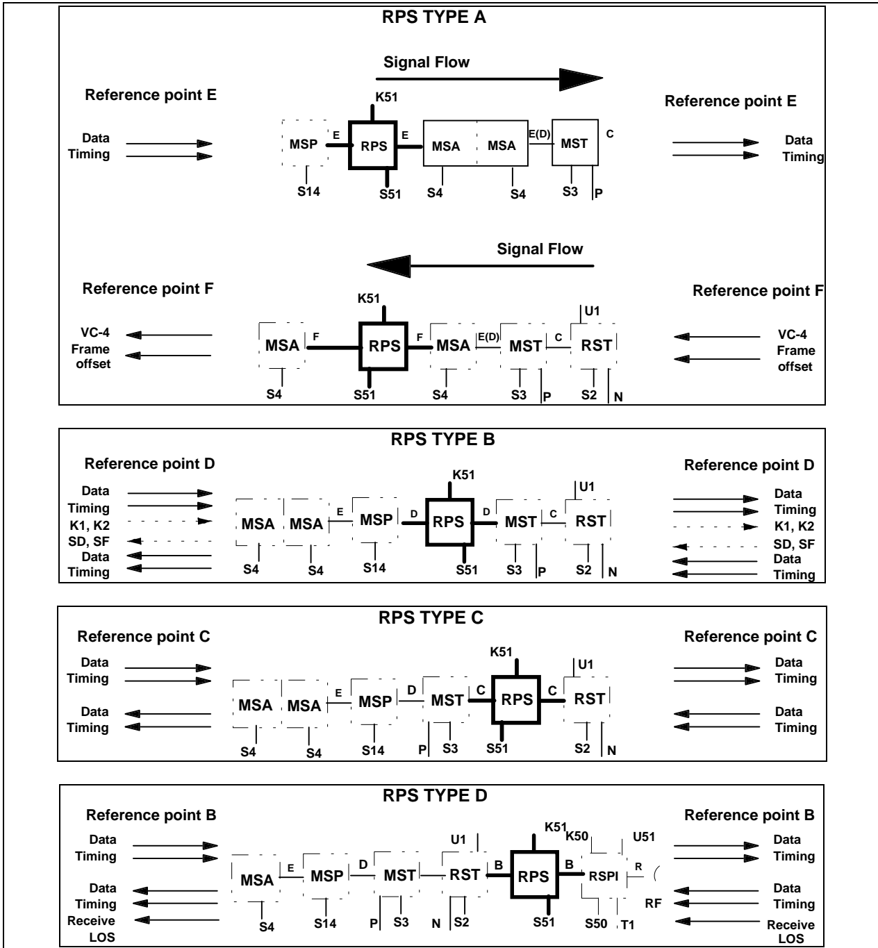
Figure A.2: Possible reference points of the RPS functional block
