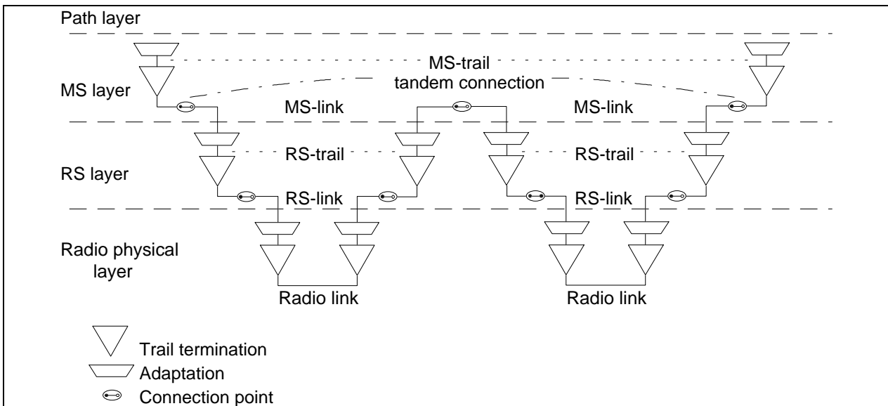
Figure C.3: ITU-T Recommendation G.783 [7] functional blocks and the corresponding managed object classes example
