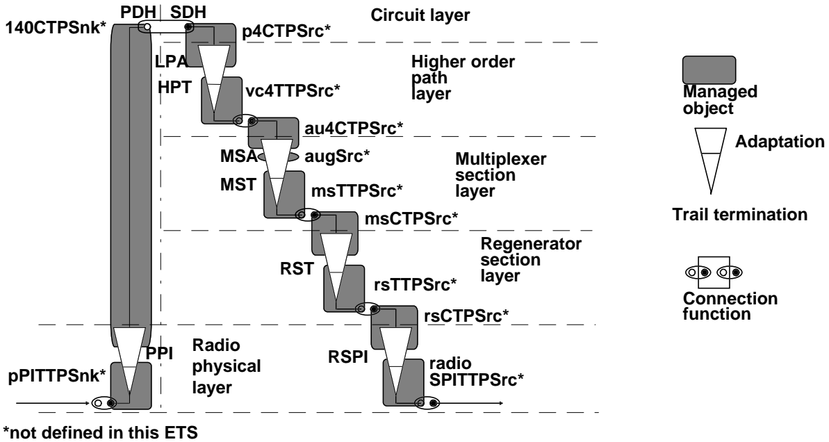
Figure C.2: EXAMPLE: 140 Mbit/s signals multiplexed to STM-1 signal
