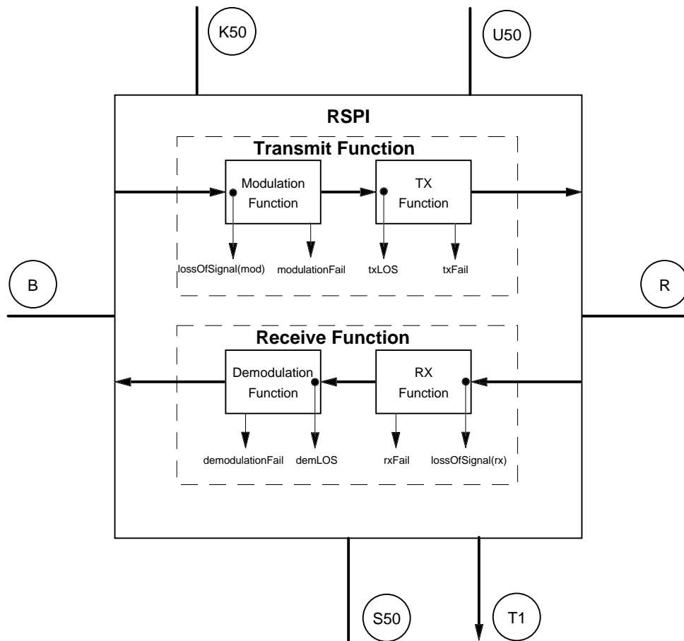
Figure 3: RSPI functional block(detail)
