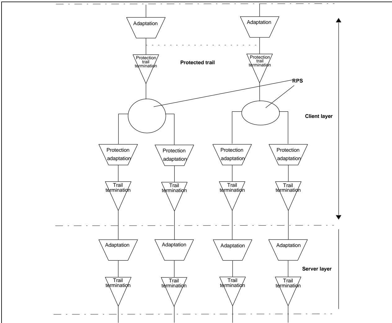
Figure C.5: Trail protection scheme
