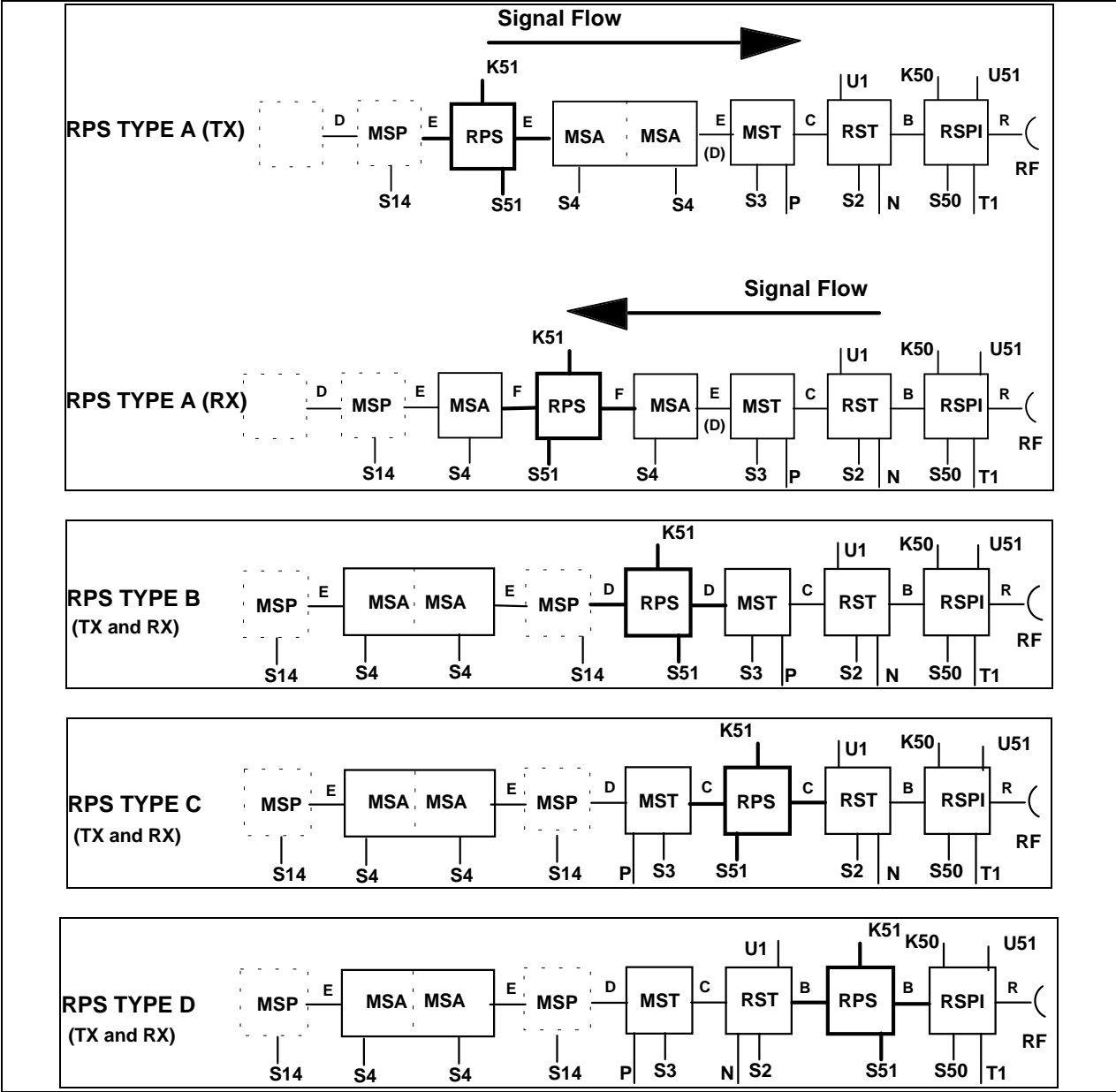
Figure A.1: Possible logical allocation of the RPS functional block
