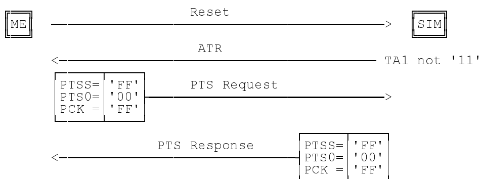
Figure 1: PTS procedure
