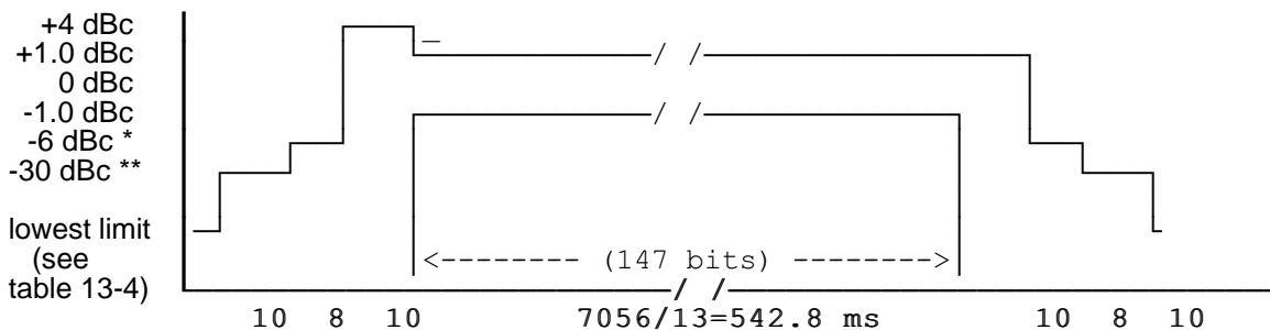
Figure 13-1: Power / time template for normal bursts
