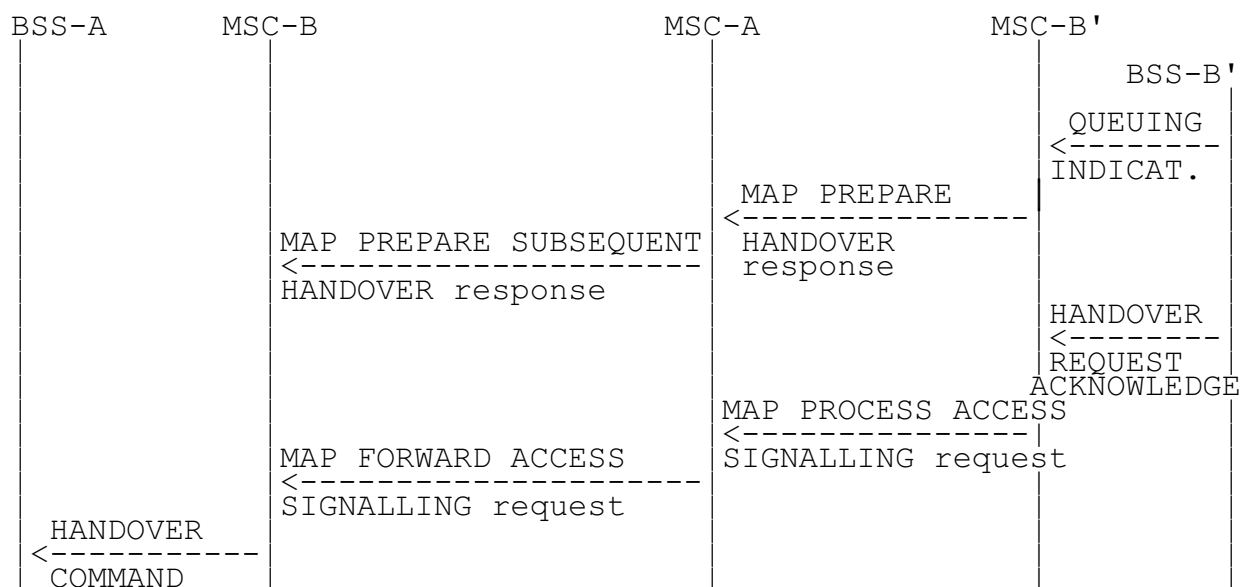
Figure 17: Signalling for Subsequent Inter-MSC Handover to third MSC (MSC-B') execution (Positive outcome)
