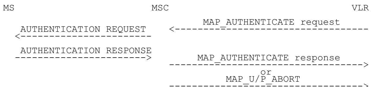
Figure 2: Authentication operation
