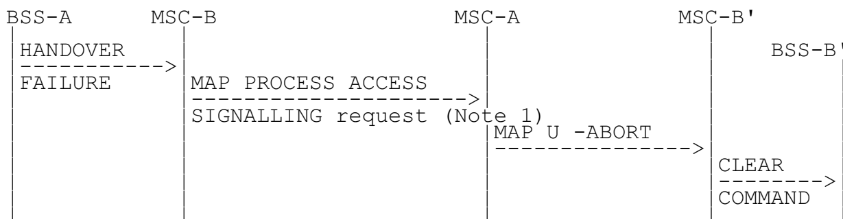
Figure 20: Signalling for Subsequent Inter-MSC Handover to third MSC (MSC-B') completion (Unsuccessful completion of the procedure)
