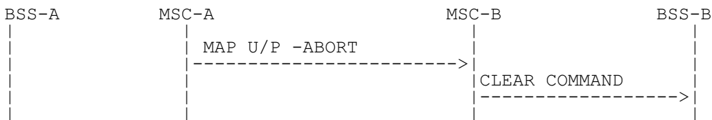
Figure 10: Signalling for Basic Inter-MSC Handover completion (Negative outcome)
