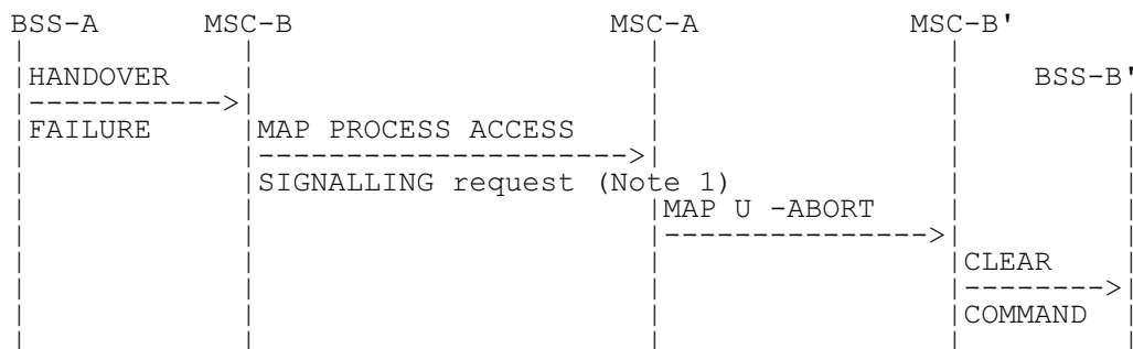
Figure 20: Signalling for Subsequent Inter-MSC Handover to third MSC (MSC-B') completion (Unsuccessful completion of the procedure)
