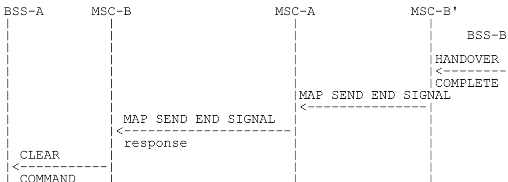
Figure 19: Signalling for Subsequent Inter-MSC Handover to third MSC (MSC-B') completion (Successful completion of the procedure)
