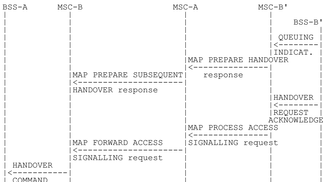
Figure 17: Signalling for Subsequent Inter-MSC Handover to third MSC (MSC-B') execution (Positive outcome)
