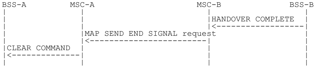
Figure 8: Signalling for Basic Inter-MSC Handover completion
