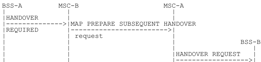
Figure 11: Signalling for Subsequent Inter-MSC Handover back to MSC-A initiation
