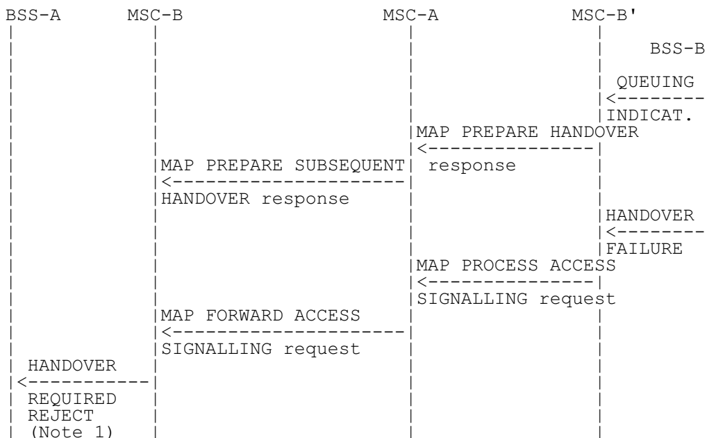
Figure 18: Signalling for Subsequent Inter-MSC Handover to third MSC (MSC-B') execution (Negative outcome)
