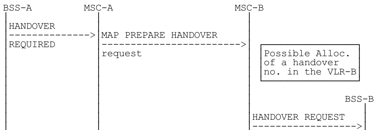
Figure 5a: Signalling for Basic Inter-MSC Handover initiation (no trace related messages transferred)
