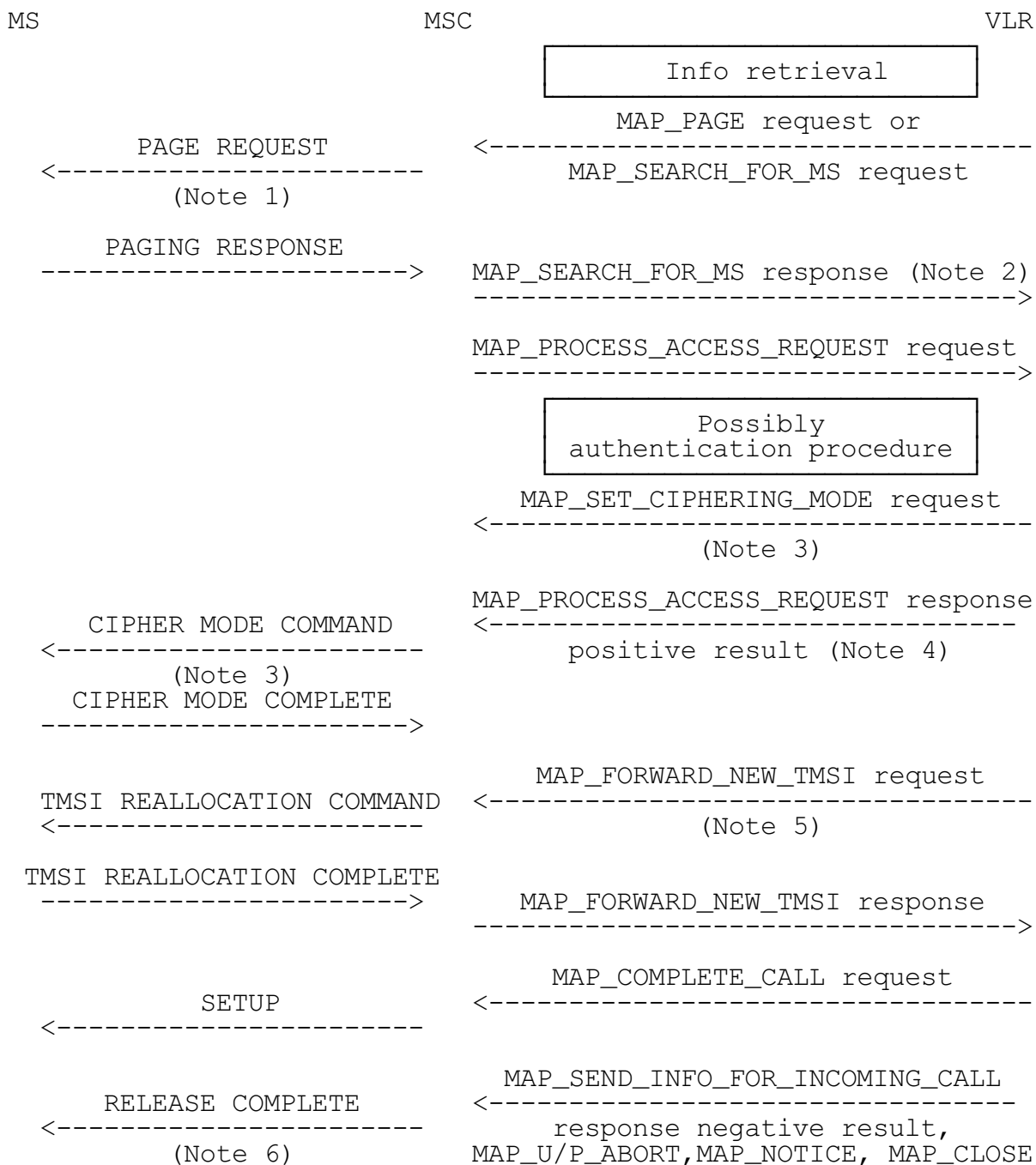
Figure 4: Incoming call set-up
