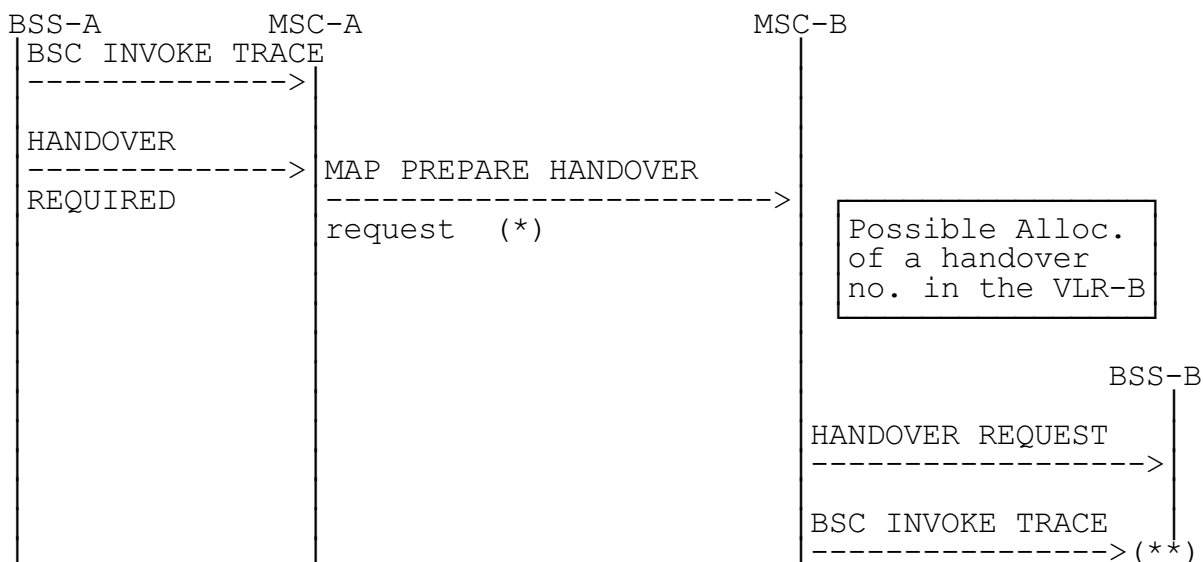
Figure 5b: Signalling for Basic Inter-MSC Handover initiation (BSC invoke trace message transferred)
