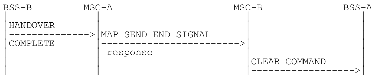
Figure 14: Signalling for Subsequent Inter-MSC Handover back to MSC-A completion (Successful completion of the procedure)
