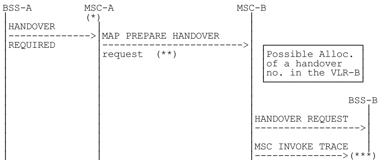
Figure 5c: Signalling for Basic Inter-MSC Handover initiation (MSC invoke trace message transferred)
