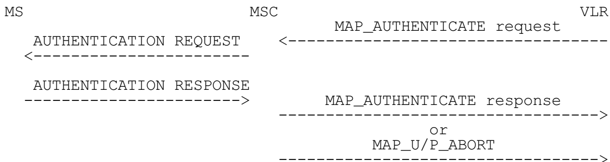
Figure 2: Authentication operation
