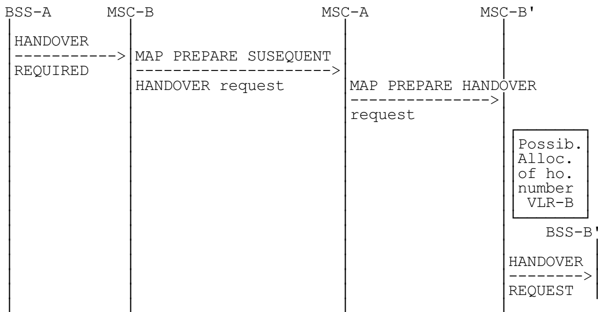
Figure 16: Signalling for Subsequent Inter-MSC Handover to third MSC (MSC-B') initiation
