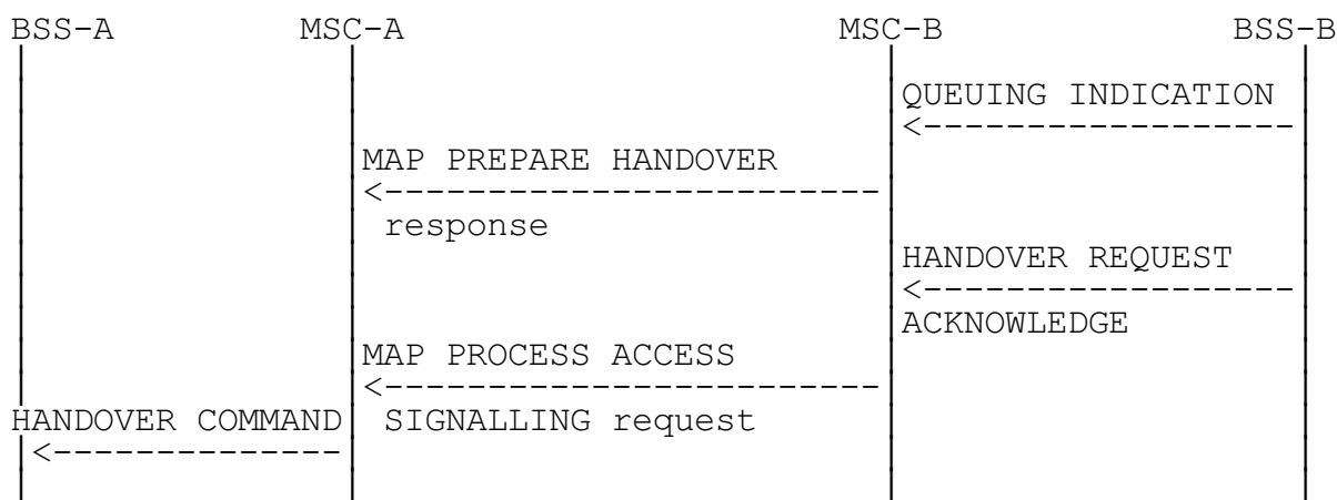
Figure 6: Signalling for Basic Inter-MSC Handover execution (Positive outcomes)
