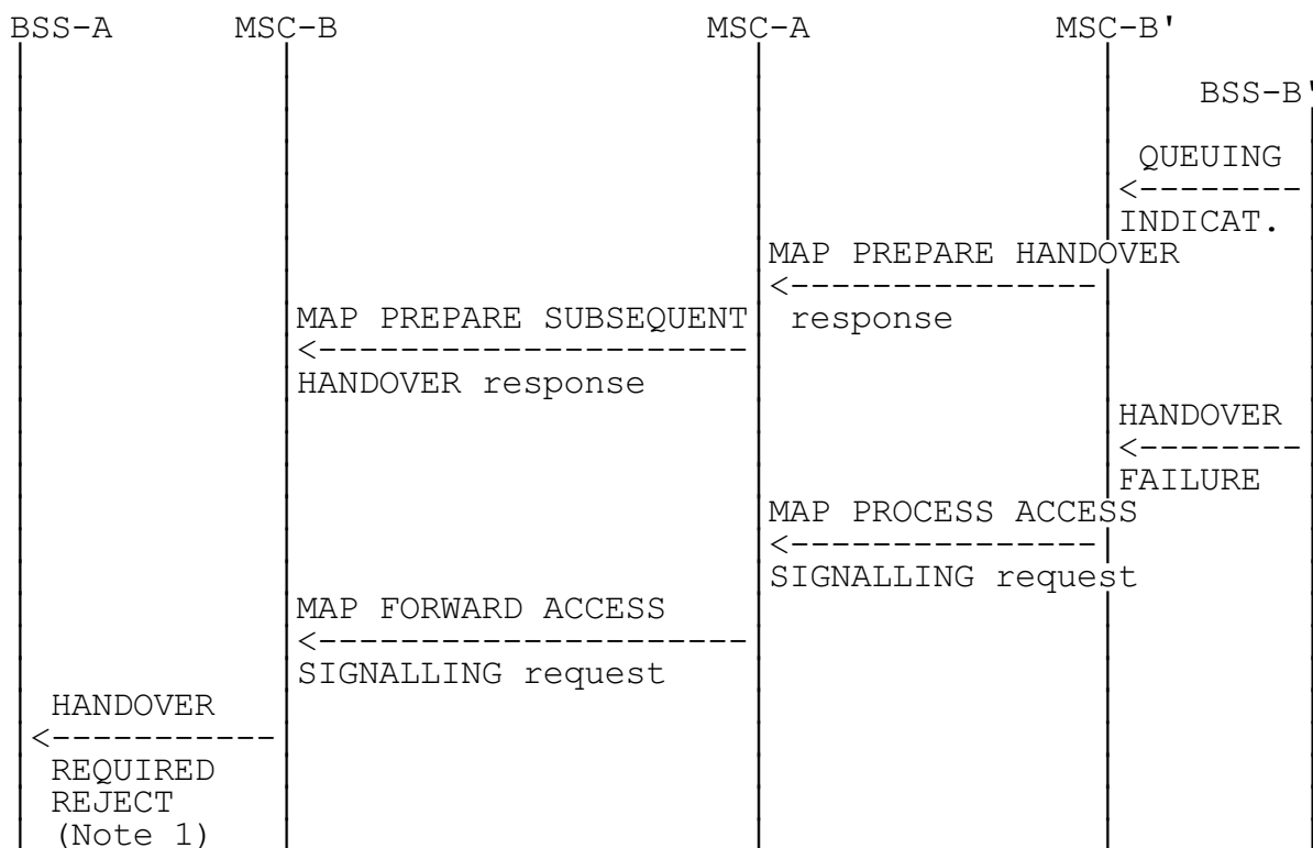
Figure 18: Signalling for Subsequent Inter-MSC Handover to third MSC (MSC-B') execution (Negative outcome)
