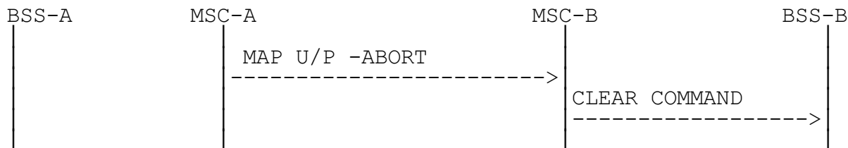
Figure 10: Signalling for Basic Inter-MSC Handover completion (Negative outcome)
