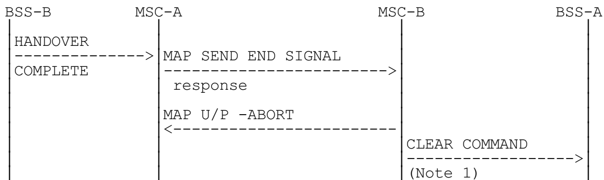
Figure 15: Signalling for Subsequent Inter-MSC Handover back to MSC-A completion (Unsuccessful completion of the procedure)
