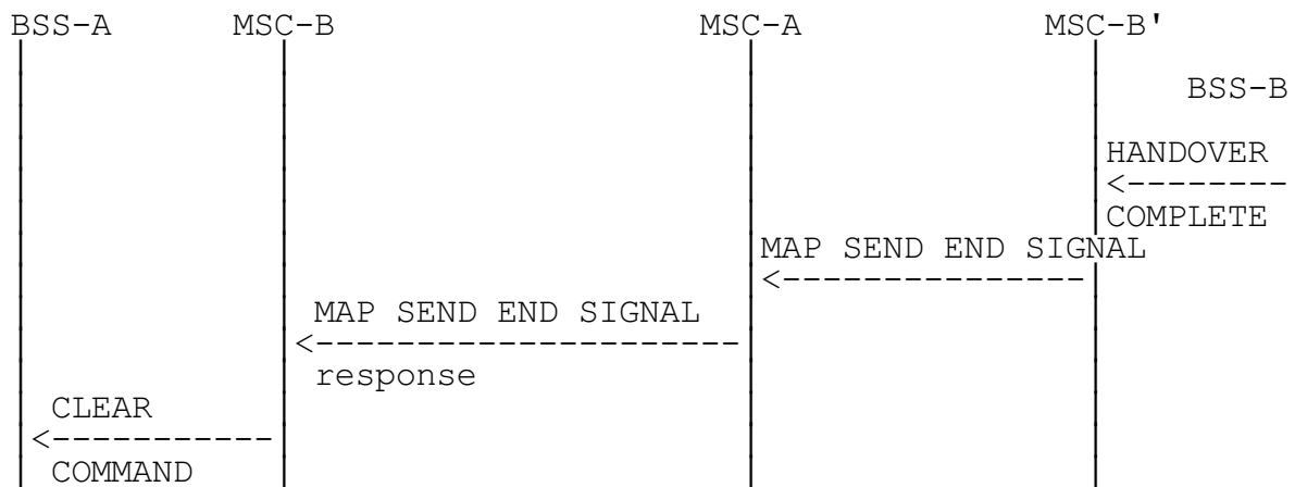
Figure 19: Signalling for Subsequent Inter-MSC Handover to third MSC (MSC-B') completion (Successful completion of the procedure)
