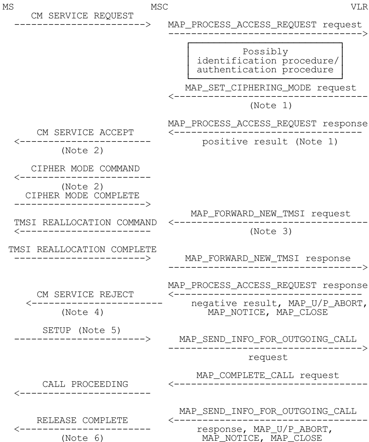
Figure 3: Part of outgoing call set-up sequence
