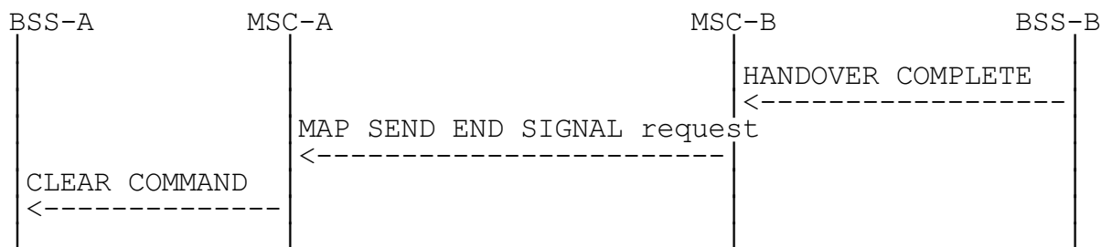
Figure 8: Signalling for Basic Inter-MSC Handover completion
