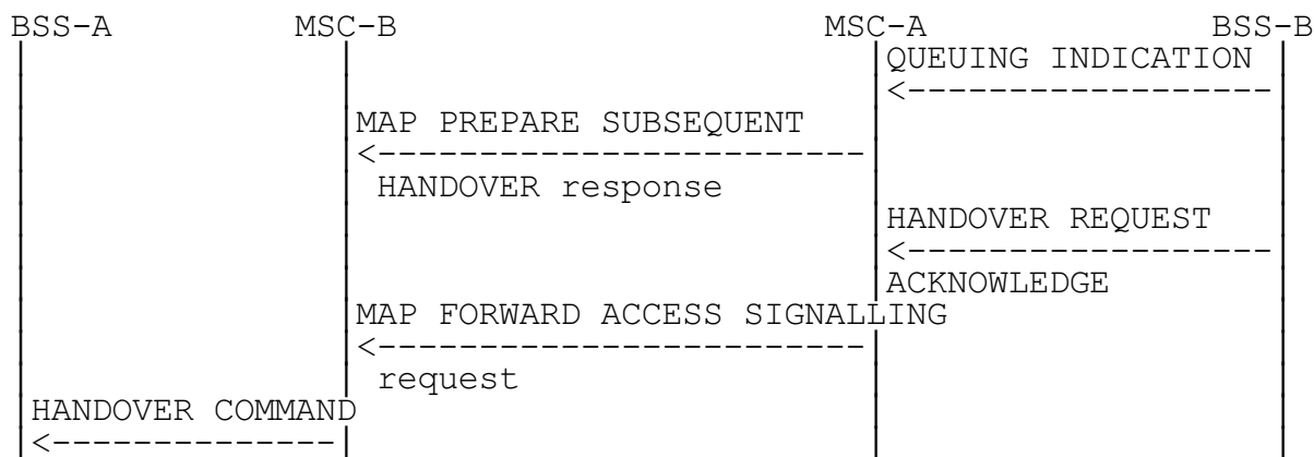
Figure 12: Signalling for Subsequent Inter-MSc Handover back to MSC-A execution (Positive outcome)
