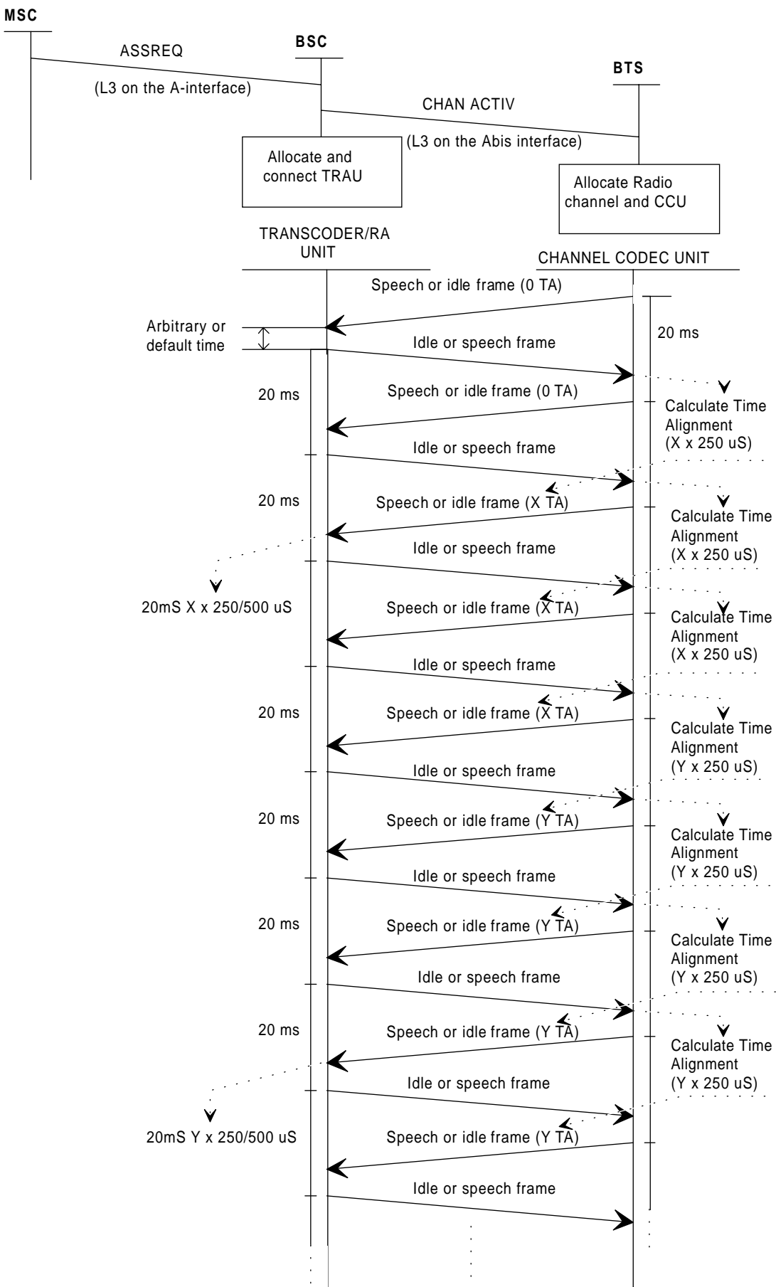
Figure GSM 08.60/4.1:Initial Time Alignment procedure
