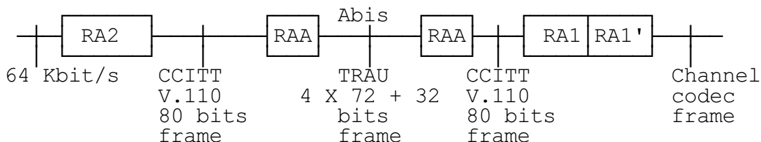
Figure TS GSM 08.60/4.3: Rate adaption when 16 kbit/s traffic channels are used.
