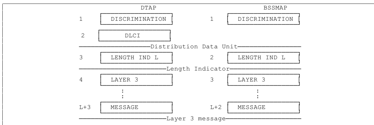
Figure 3/08.06 Structure of the User Data Field
