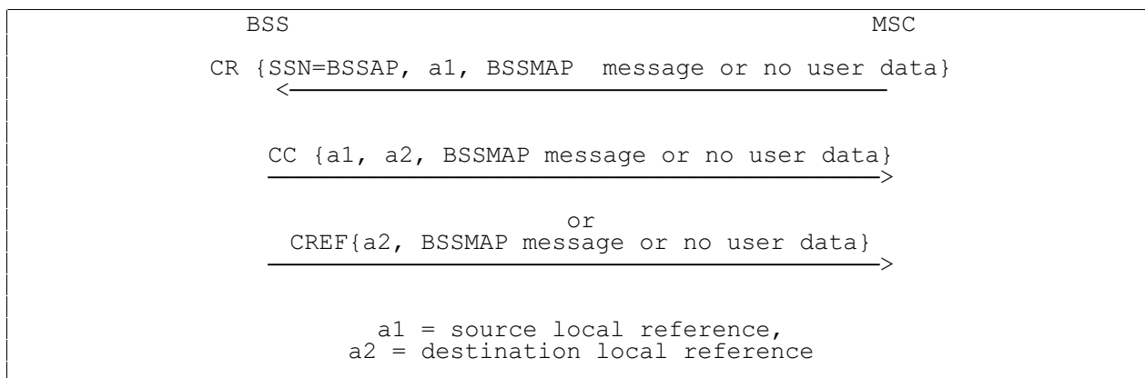
Figure 2/08.06 Set-up of SCCP connections on a new BSS/MSC (handover) interface
