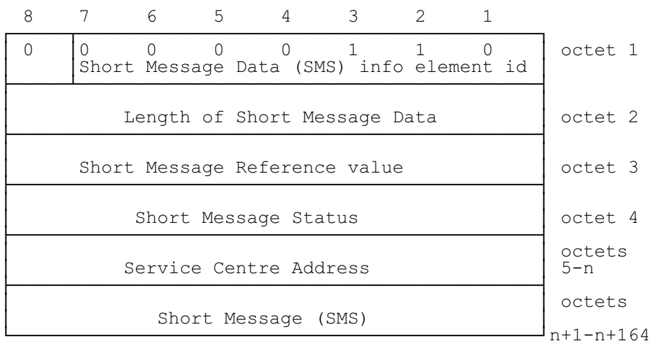
Figure 2.5.8/GSM 07.05: Short Message Data (SMS) information element
