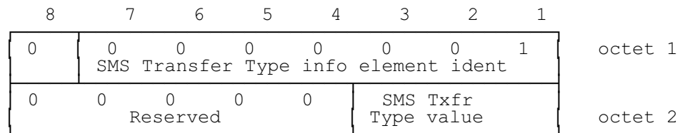
Figure 2.5.3/GSM 07.05: SMS Transfer Type information element
