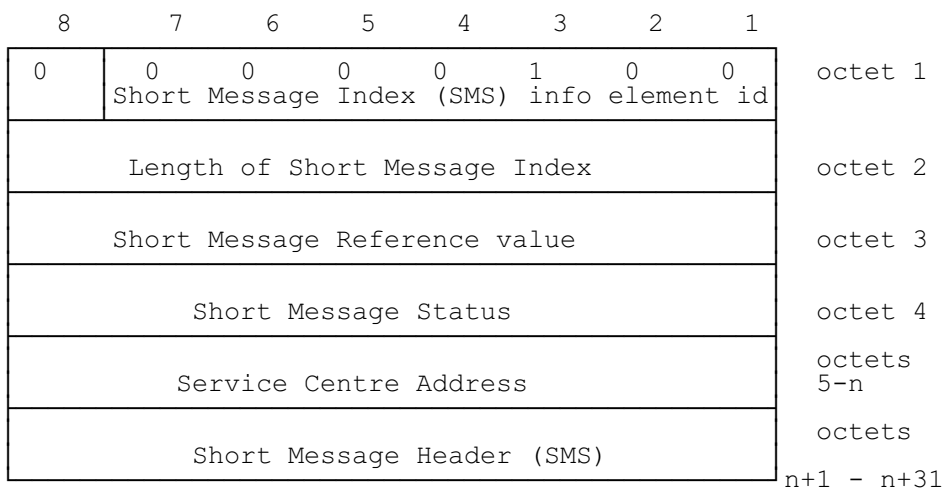
Figure 2.5.6/GSM 07.05: Short Message Index (SMS) information element
