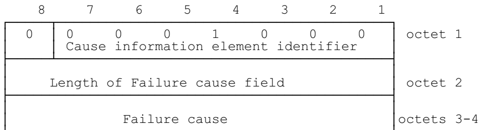
Figure 2.5.16/GSM 07.05: TP-Failure Cause information element
