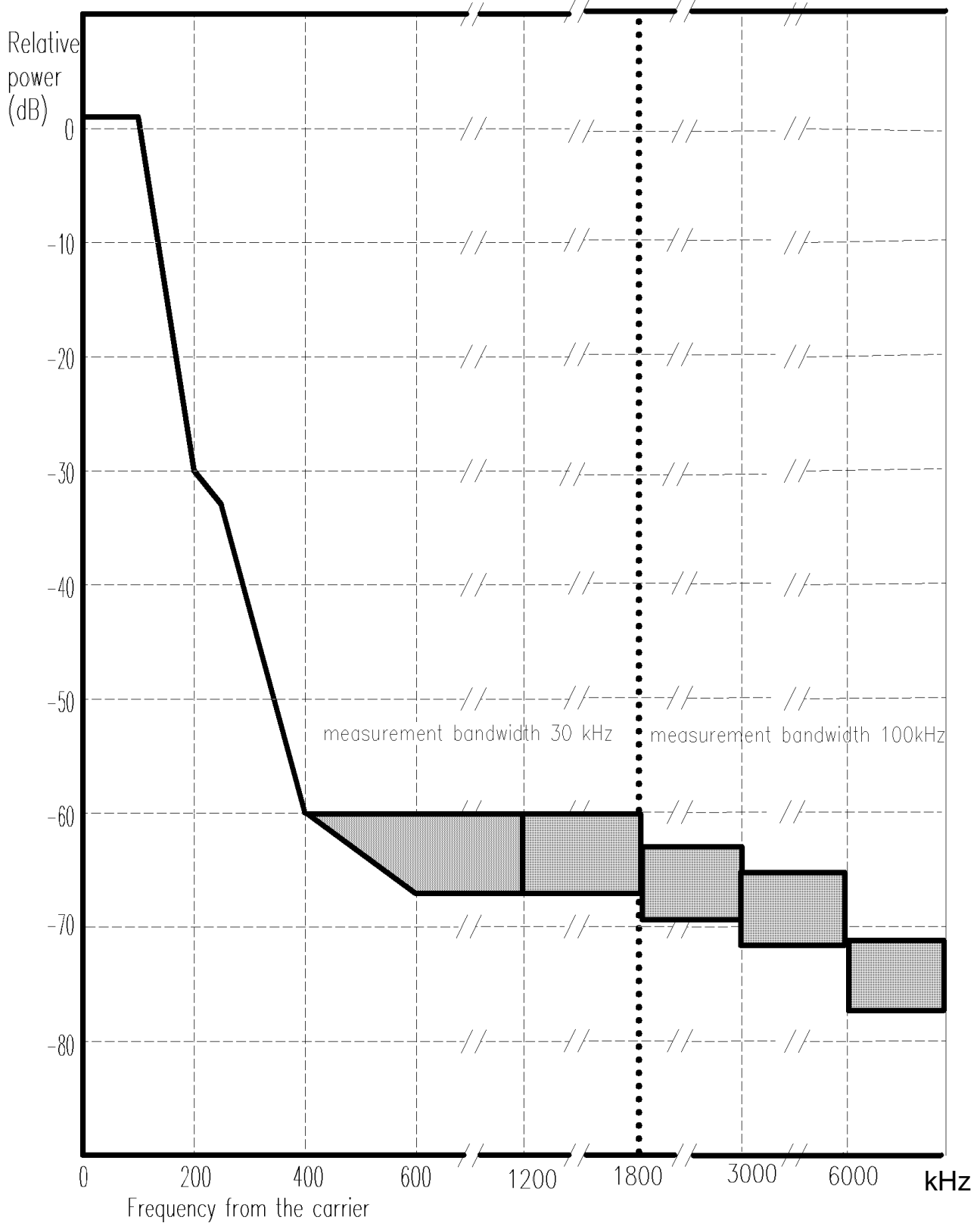
Figure A.1: GSM 900 MS spectrum due to modulation
