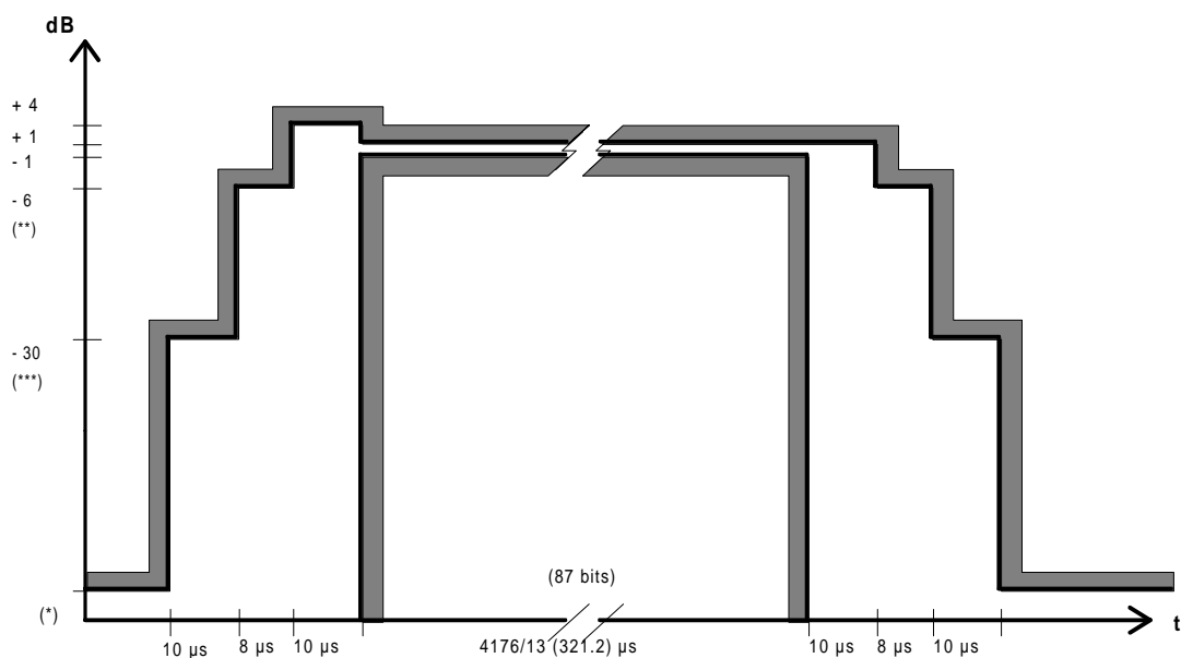
Time mask for access burst (AB)
