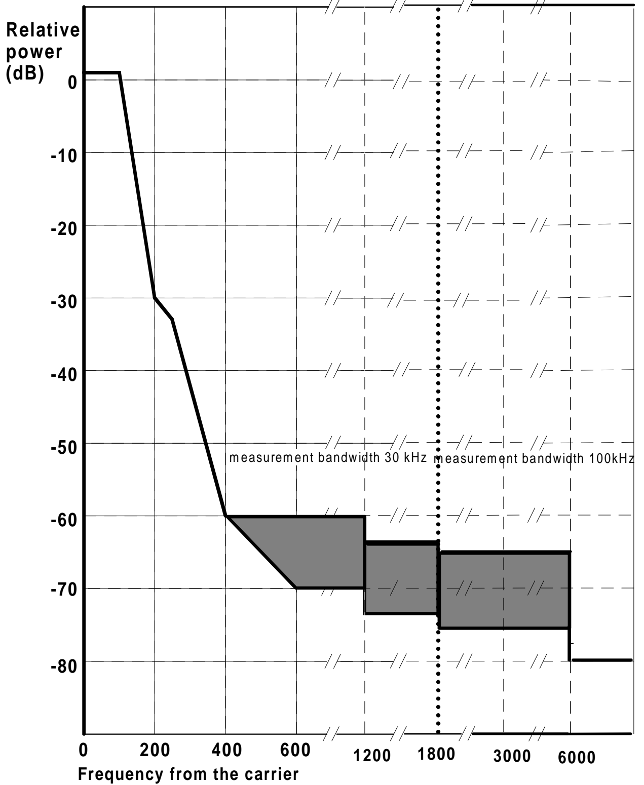
Figure A.2: GSM 900 BTS spectrum due to modulation
