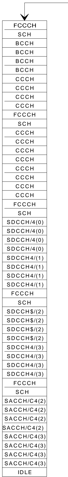
Figure 8: Example of TDMA frame mapping for control channels
