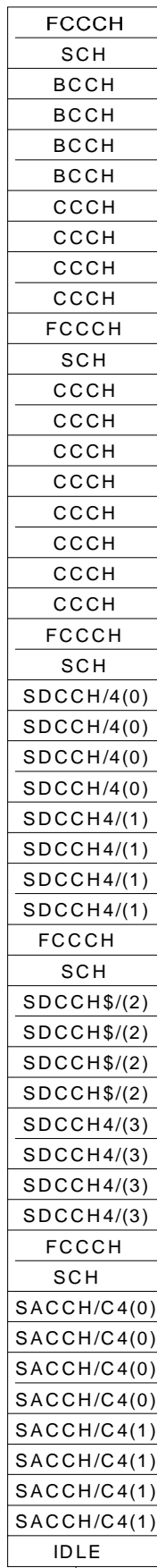
Figure 8: Example of TDMA frame mapping for control channels
