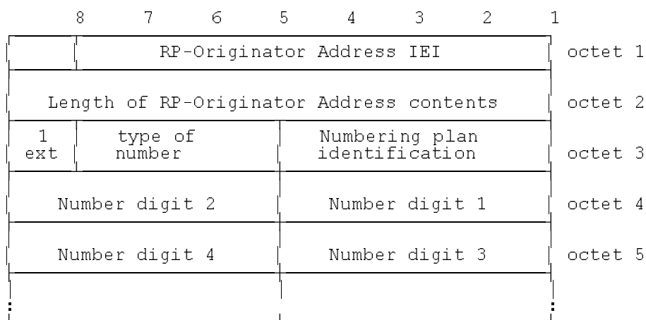
Figure 8.5/GSM 04.11: RP-Originator Address information element
