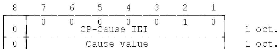
Figure 8.3/GSM 04.11: CP-Cause element layout.
