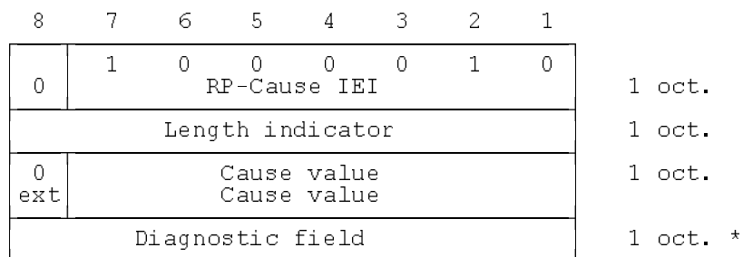
Figure 8.8/GSM 04.11: RP-Cause element layout.
