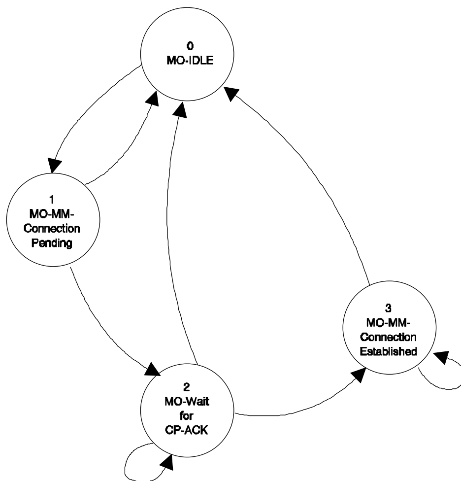
MO-SMC-entity on MS-side State transition diagram
