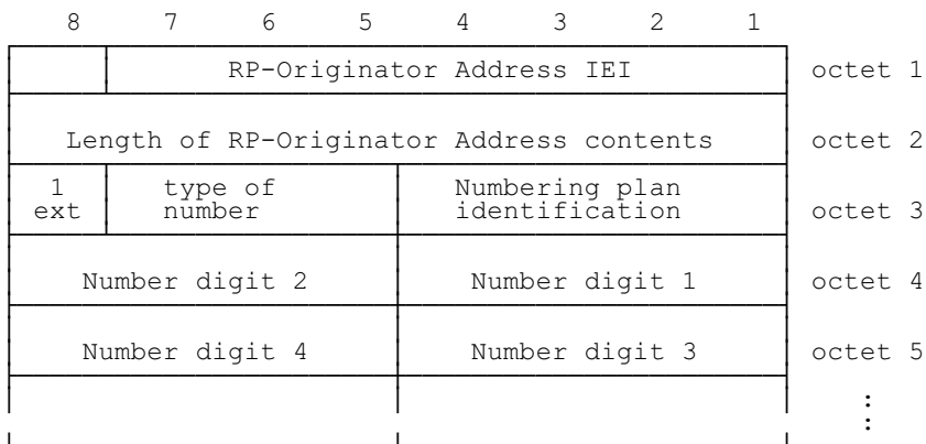
Figure 8.5/GSM 04.11: RP-Originator Address information element
