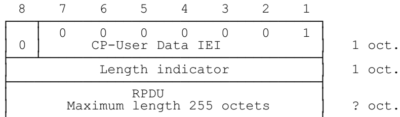
Figure 8.2/GSM 04.11: CP-User data element layout.
