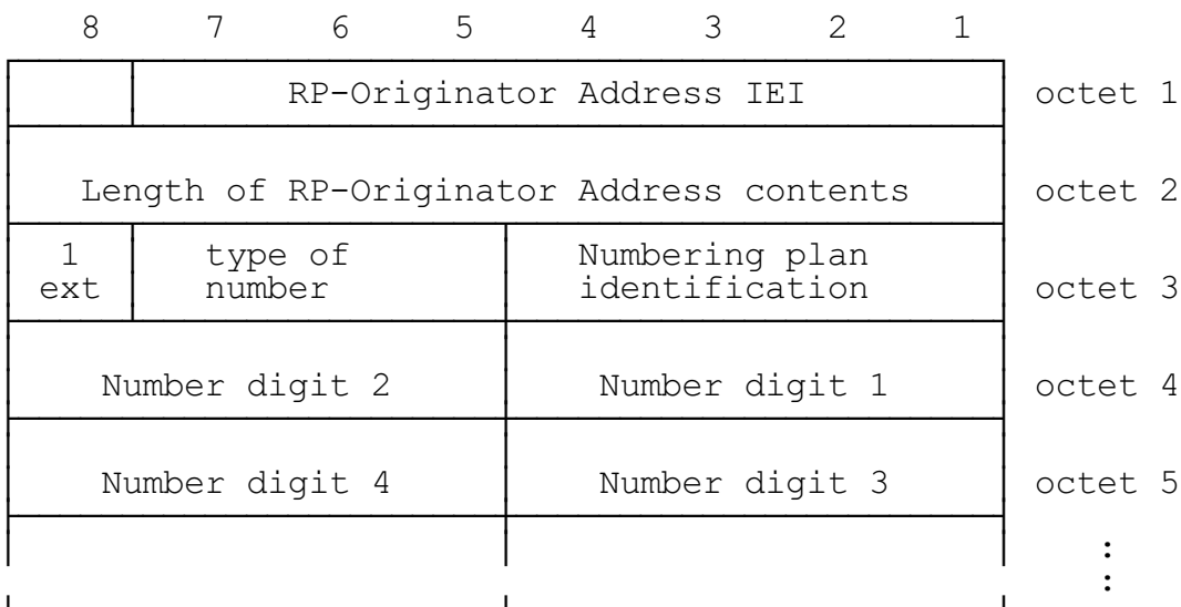
Figure 8.5/GSM 04.11: RP-Originator Address information element
