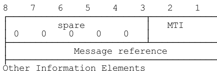
Figure 8.4/GSM 04.11.
