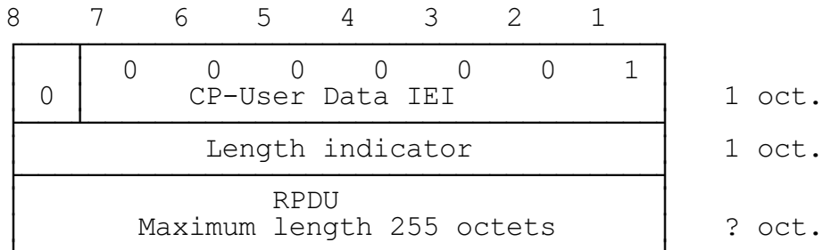
Figure 8.2/GSM 04.11: CP-User data element layout.
