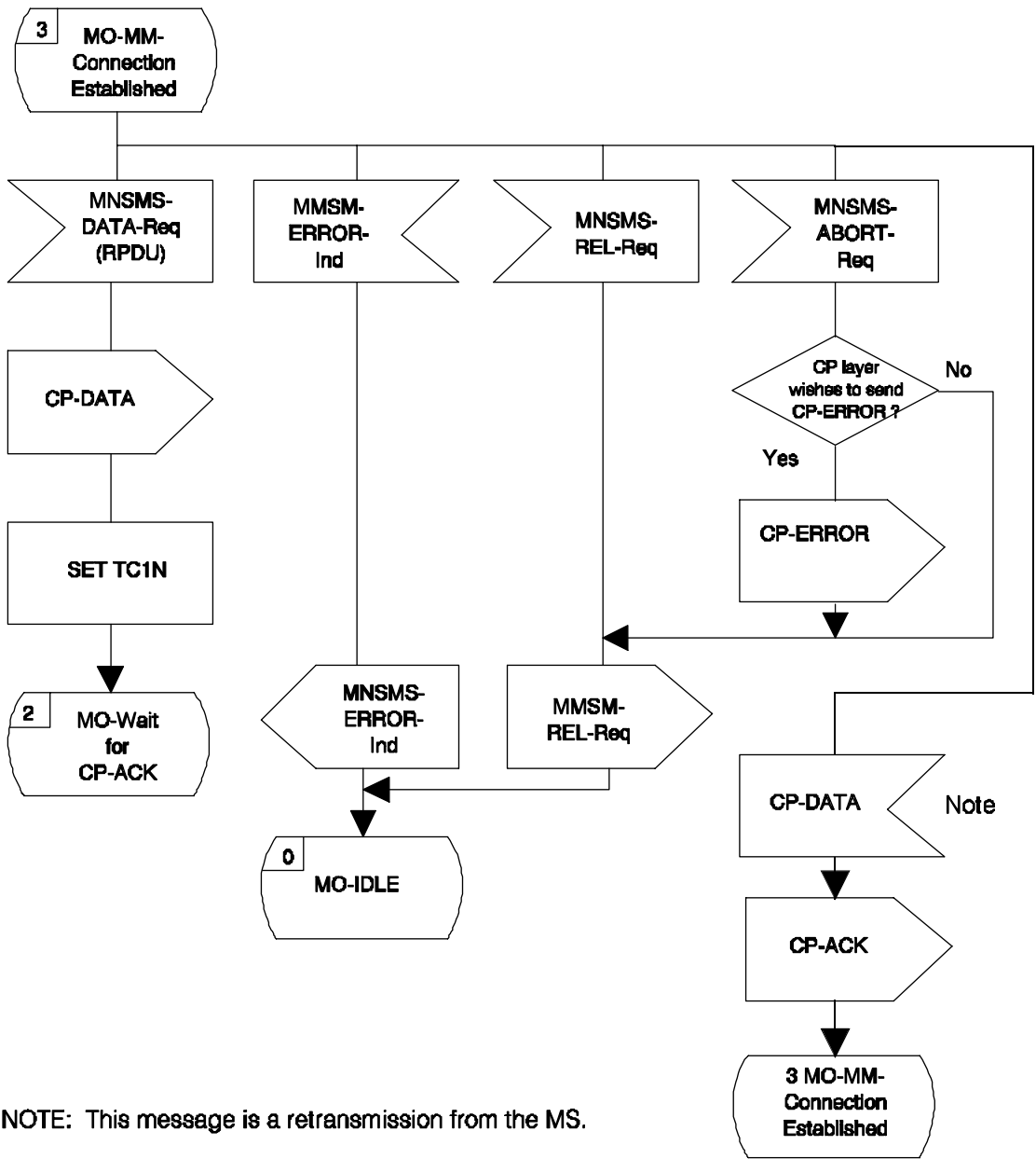
MO-SMC-entity on Network side SDL-9
