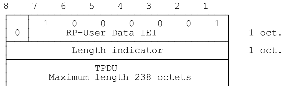
Figure 8.7/GSM 04.11: RP-User data element layout.
