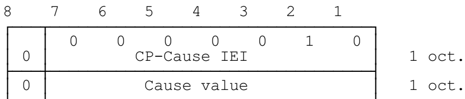
Figure 8.3/GSM 04.11: CP-Cause element layout.
