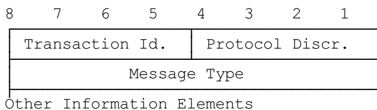
Figure 8.1/GSM 04.11.
