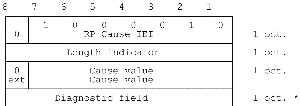
Figure 8.8/GSM 04.11: RP-Cause element layout.
