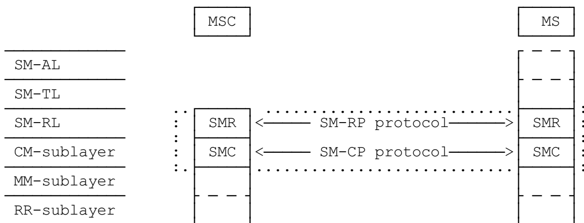
Figure 2.1/GSM 04.11: Protocol hierarchy
