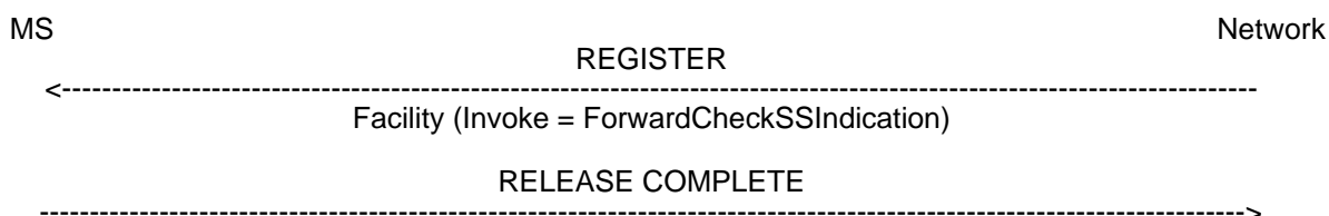
Figure 6.1: ForwardCheckSSIndication sent on new transaction
