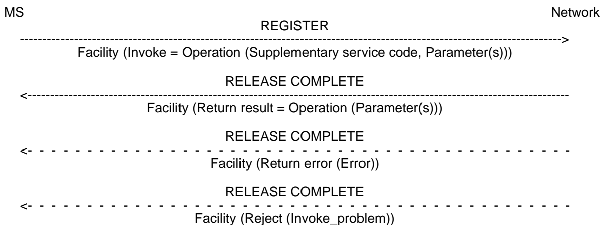
Figure 3.1: Mobile station initiated supplementary service transaction
