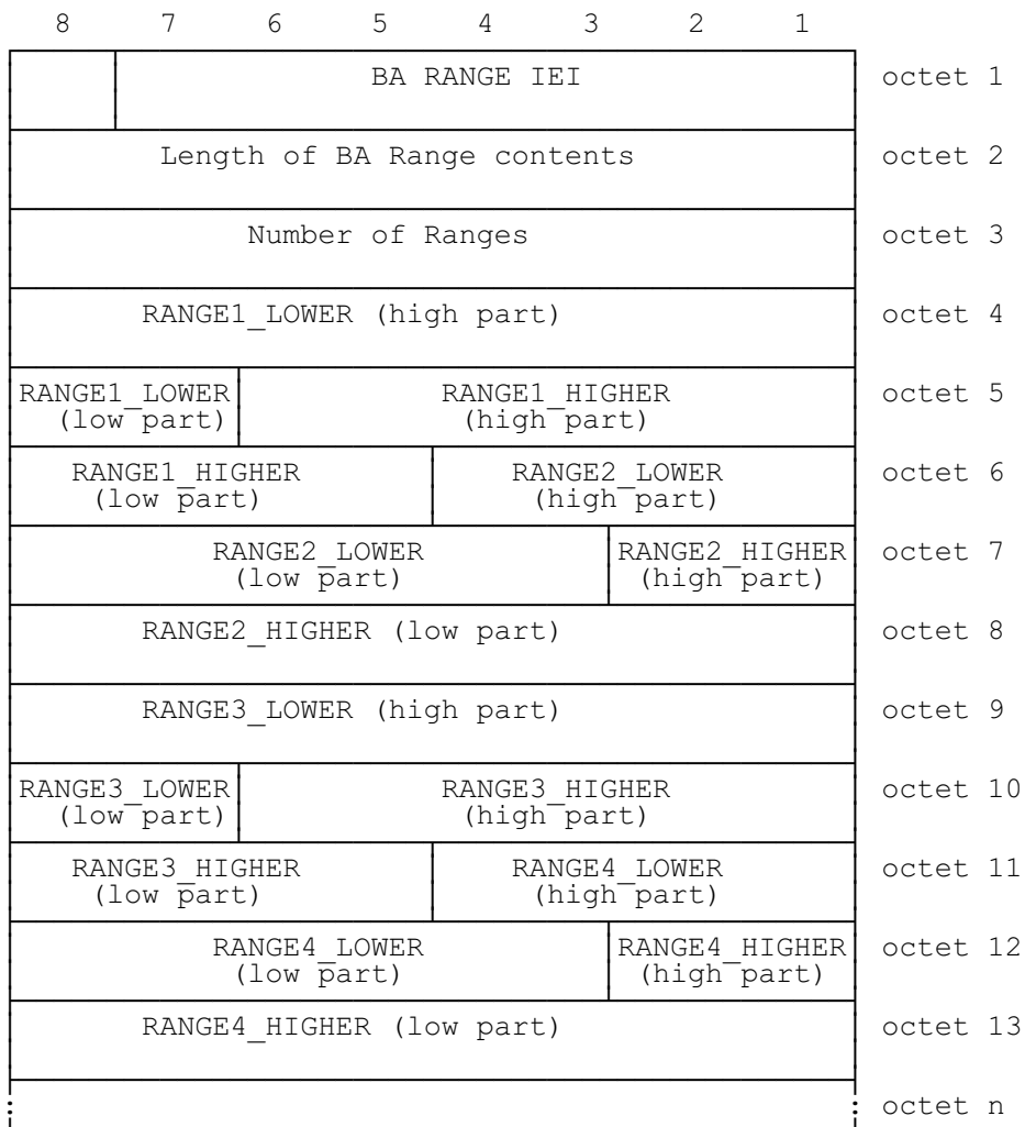
FIGURE 10.8a/GSM 04.08 BA RANGE information element
