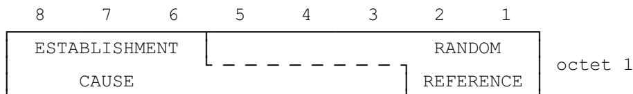
FIGURE 9.1/GSM 04.08 CHANNEL REQUEST message content
