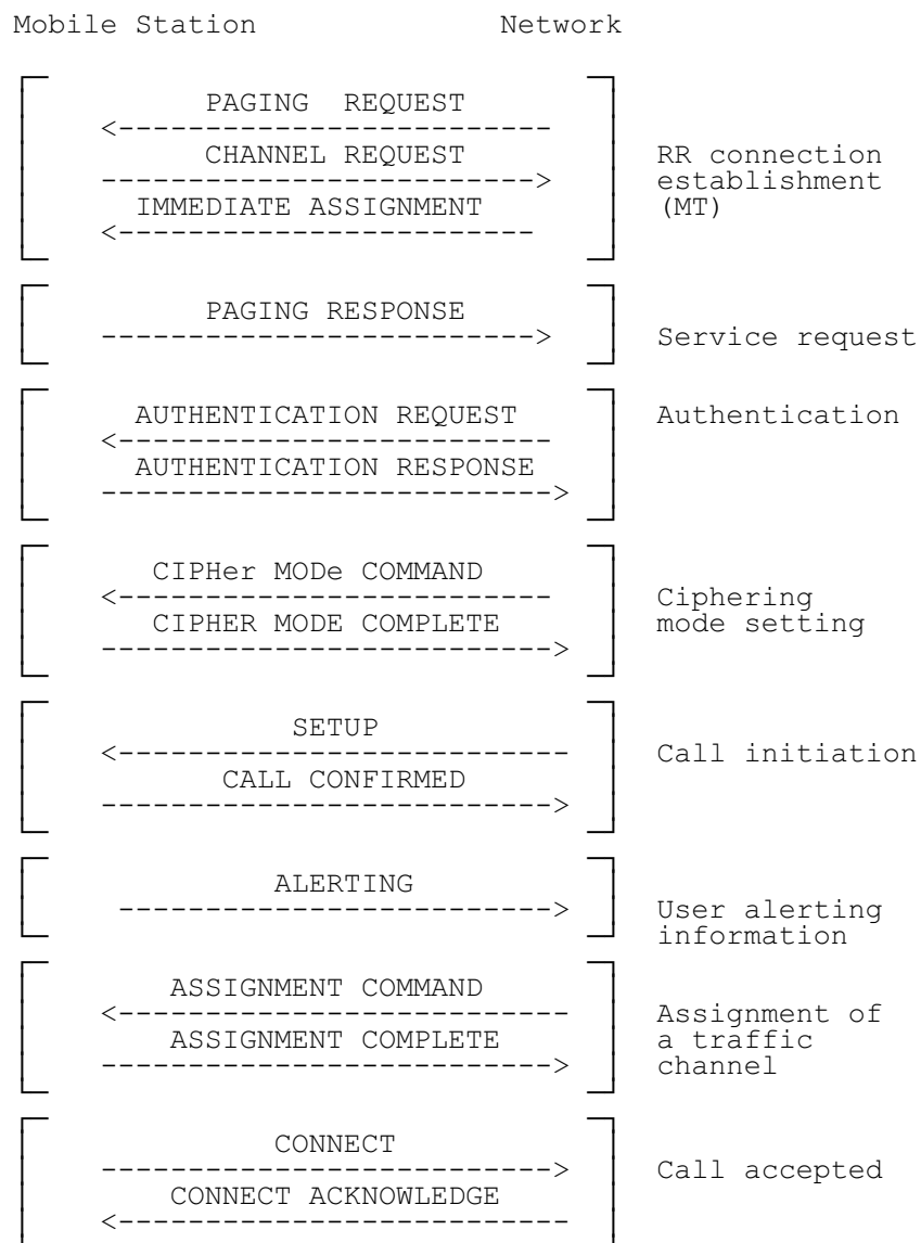
Figure 7.11b/GSM 04.08 - Mobile terminating call establishment with OACSU (late assignment)
