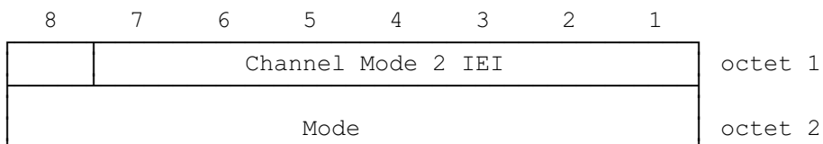
FIGURE 10.21/GSM 04.08 Channel Mode 2 information element
