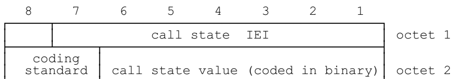
FIGURE 10.72/GSM 04.08 Call state information element
