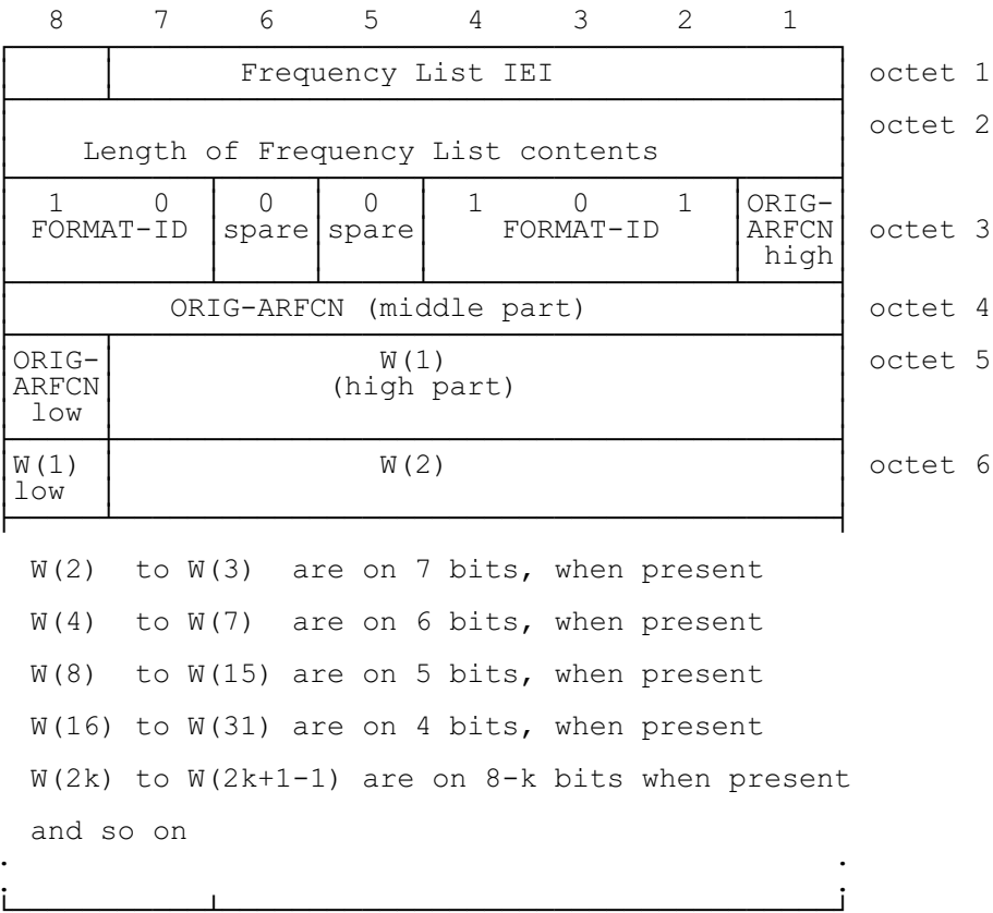
FIGURE 10.30/GSM 04.08 Frequency List information element (Range 256 format)
