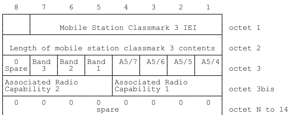
FIGURE 10.8/GSM 04.08 Mobile Station Classmark 3 information element
