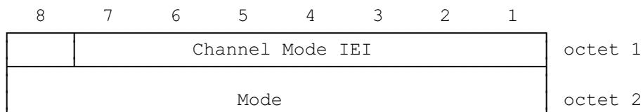
FIGURE 10.20/GSM 04.08 Channel Mode information element
