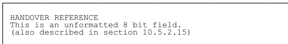
FIGURE 9.2/GSM 04.08 HANDOVER ACCESS message content
