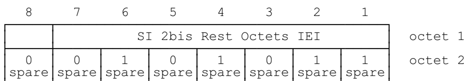
FIGURE 10.51/GSM 04.08 SI 2bis Rest Octets information element
