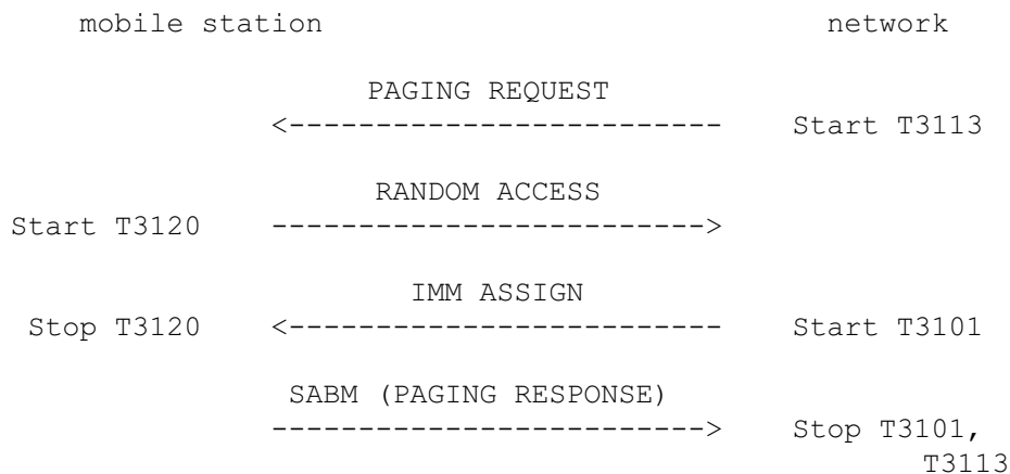
Figure 3.2/GSM 04.08 Paging sequence
