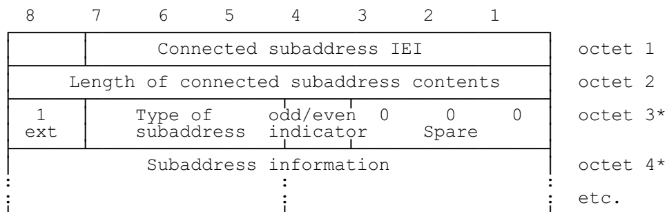
Figure 10.81/GSM 04.08
