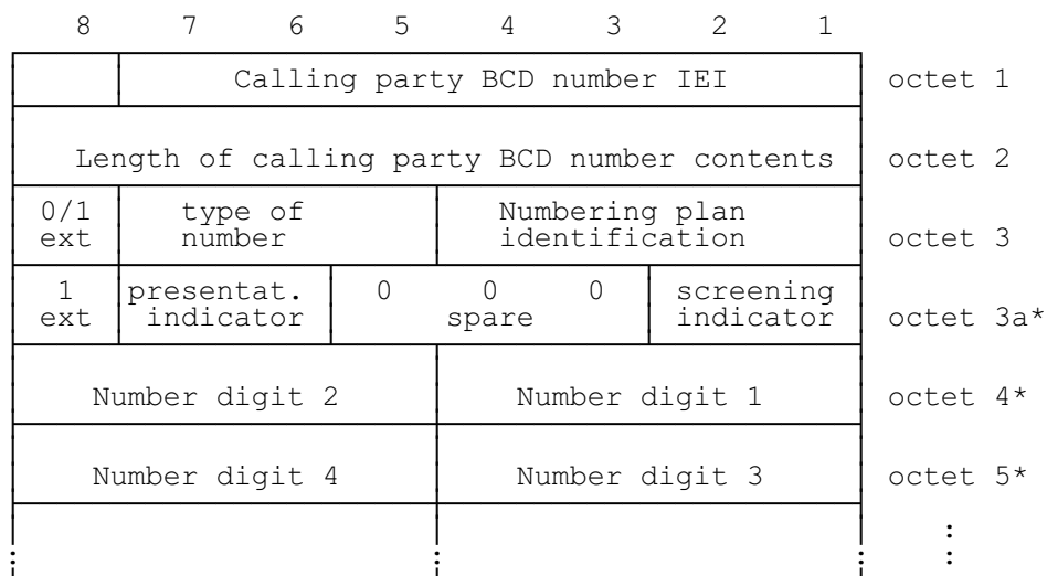
FIGURE 10.75/GSM 04.08 Calling party BCD number information element
