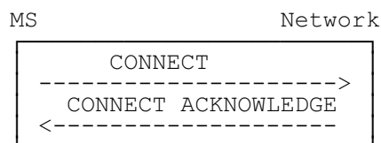
Figure 5.7/GSM 04.08
