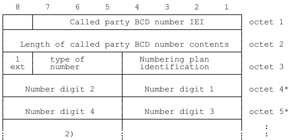
FIGURE 10.73/GSM 04.08 Called party BCD number information element
