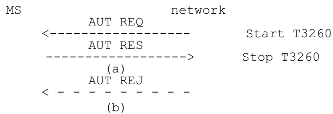
Figure 4.2/GSM 04.08 Authentication sequence: (a) authentication; (b) authentication rejection.
