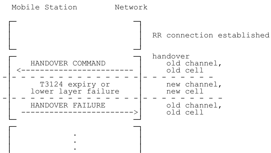
Figure 7.16/GSM 04.08
