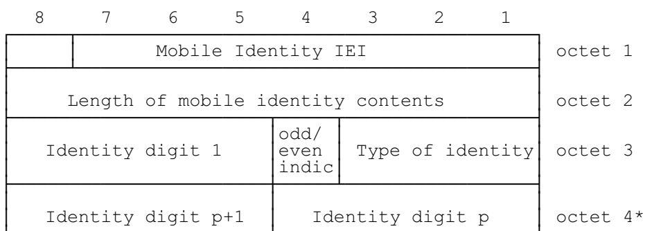
FIGURE 10.5/GSM 04.08 Mobile Identity information element
