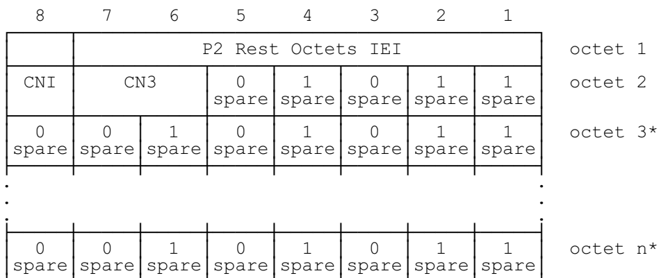
FIGURE 10.42/GSM 04.08 P2 Rest Octets information element
