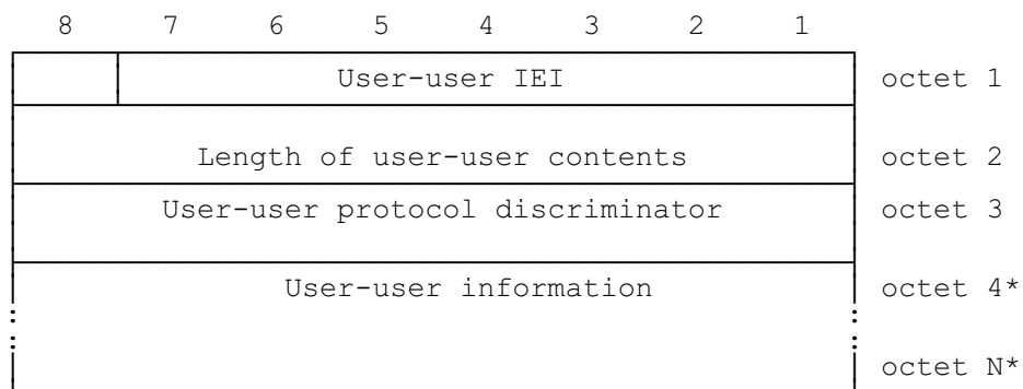
FIGURE 10.92/GSM 04.08 User-user information element
