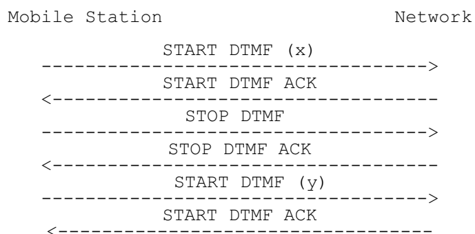
· · · Figure 5.9/GSM 04.08 Multiple DTMF transmission
