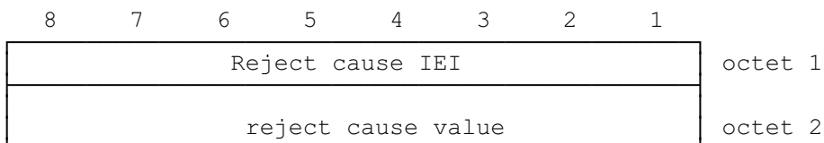
Figure 10.66/GSM 04.08: Reject Cause information element
