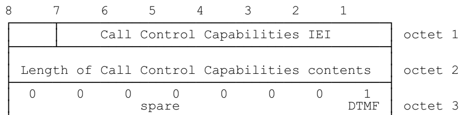
Figure 10.71a/GSM 04.08: Call Control Capabilities information element
