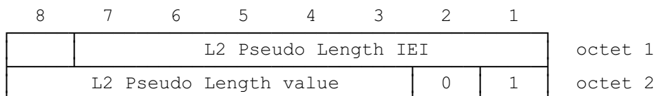
Figure 10.37/GSM 04.08: L2 Pseudo Length information element
