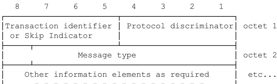
FIGURE 10.1/GSM 04.08 General message organization example
