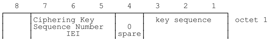
FIGURE 10.3/GSM 04.08 Cipherring Key Sequence Number information element
