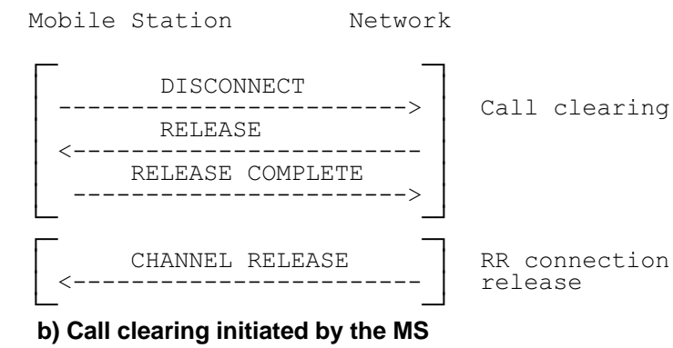
Figure 7.12/GSM 04.08 Call clearing
