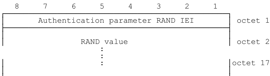
Figure 10.61a/GSM 04.08 Authentication Parameter RAND information element
