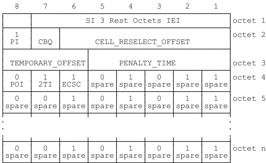
Figure 10.52i/GSM 04.08 SI 3 Rest Octets information element for PI=H & POI=L & 2TI=H & ECSC=L
