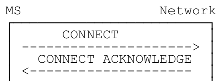
Figure 5.7/GSM 04.08
