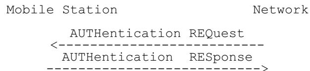
Figure 7.5/GSM 04.08 Authentication
