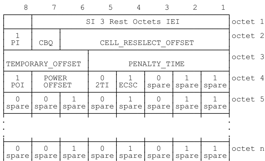
Figure 10.52d/GSM 04.08
