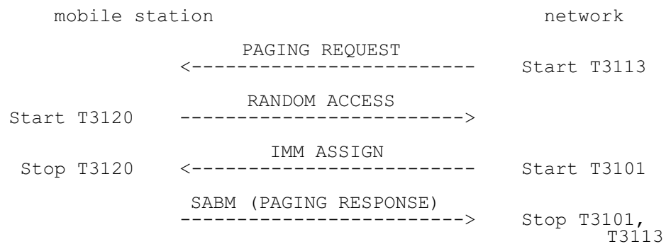
Figure 3.2/GSM 04.08 Paging sequence
