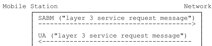
Figure 3.1/GSM 04.08 Service request and contention resolution
