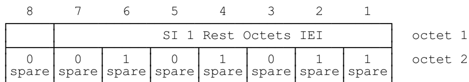
Figure 10.50/GSM 04.08 SI 1 Rest Octets information element
