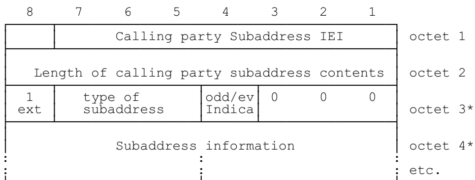
Figure 10.76/GSM 04.08 Calling party subaddress
