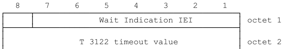
Figure 10.60/GSM 04.08 Wait Indication information element
