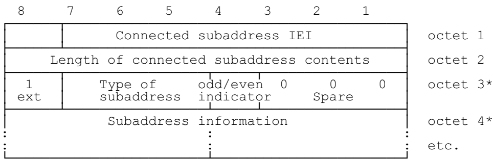
Figure 10.81/GSM 04.08
