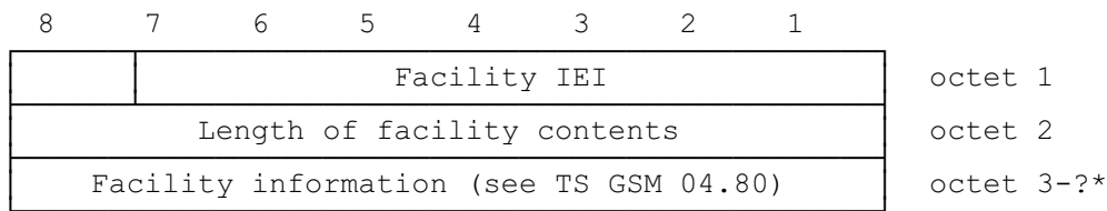
Figure 10.82/GSM 04.08
