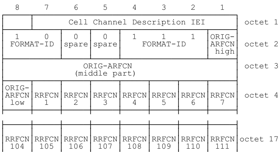
Figure 10.15/GSM 04.08
