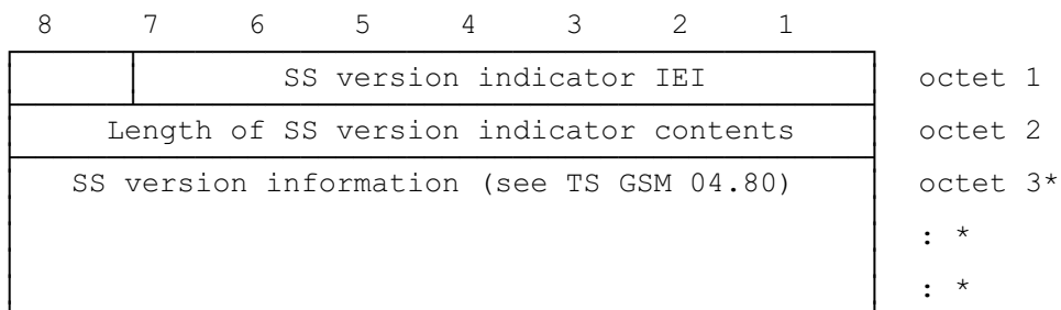
Figure 10.91/GSM 04.08
