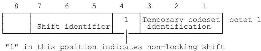
Figure 10.69/GSM 04.08 Non-locking shift element
