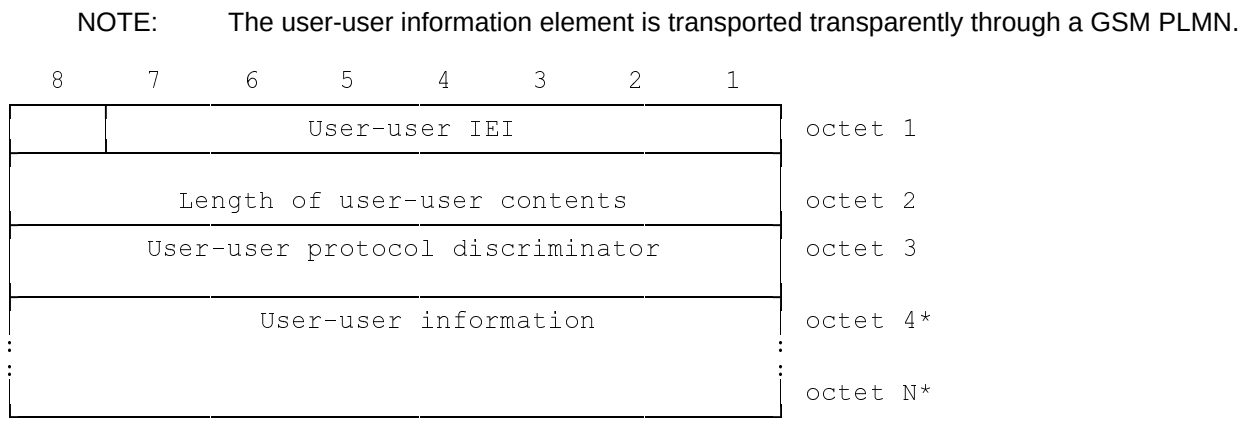
Figure 10.92/GSM 04.08 User-user information element
