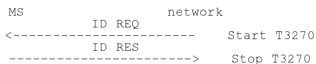
Figure 4.3/GSM 04.08 Identification sequence
