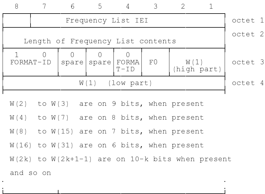
Figure 10.28/GSM 04.08 Frequency List information element (Range 1024 format)
