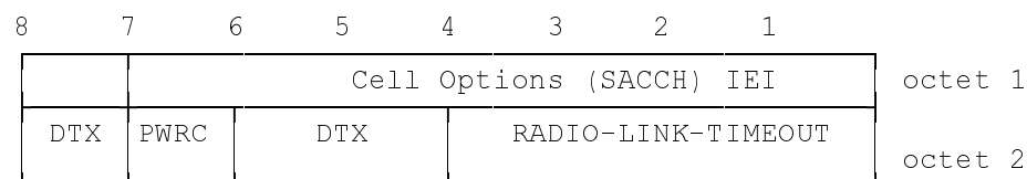
Figure 10.17a/GSM 04.08 Cell Options (SACCH) information element
