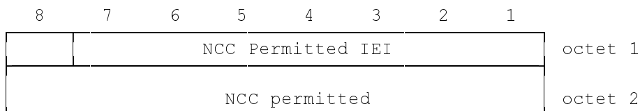
Figure 10.45/GSM 04.08 NCC Permitted information element
