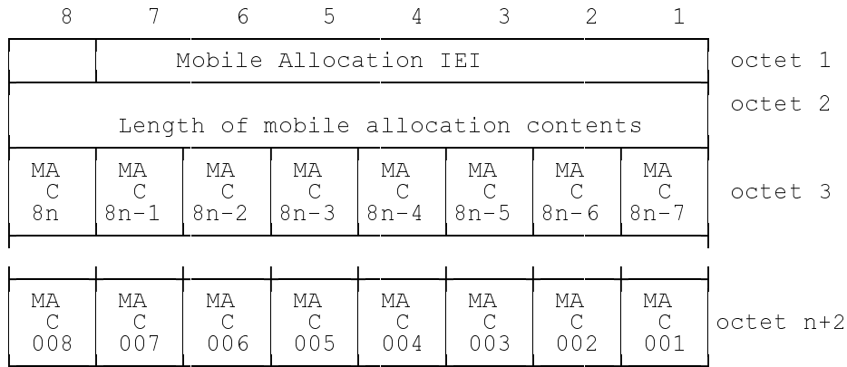
Figure 10.39/GSM 04.08 Mobile Allocation information element.
