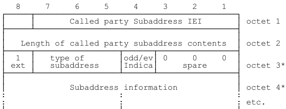
Figure 10.74/GSM 04.08: Called party subaddress
