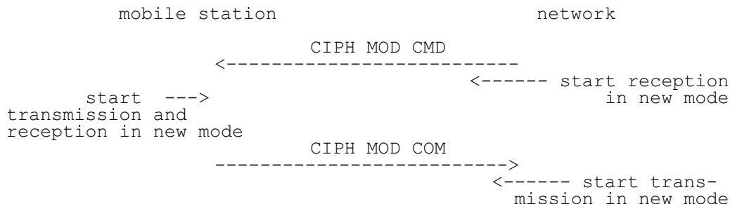
Figure 3.3/GSM 04.08: Cipherring mode setting sequence
