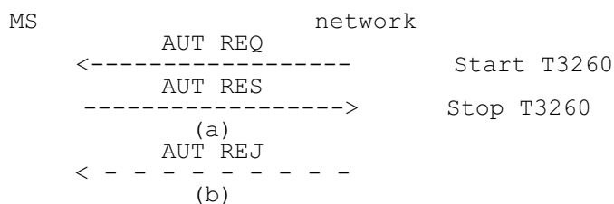
Figure 4.2/GSM 04.08: Authentication sequence: (a) authentication;(b) authentication rejection.
