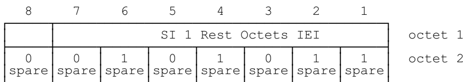
Figure 10.50/GSM 04.08: SI 1 Rest Octets information element
