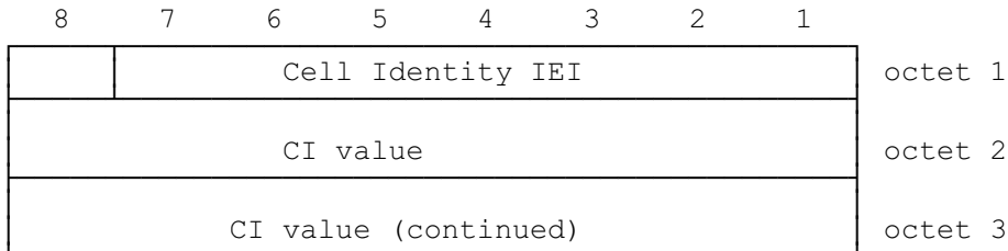
Figure 10.2/GSM 04.08: Cell Identity information element
