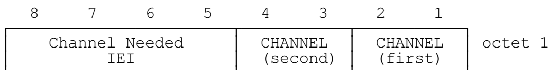
FIGURE 10.22/GSM 04.08 Channel Needed information element
