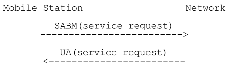
Figure 7.4/GSM 04.08 Service request and contention resolution
