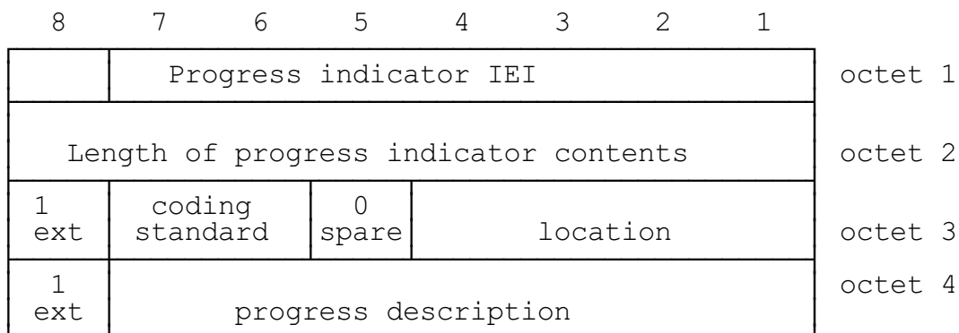
FIGURE 10.88/GSM 04.08 Progress indicator information element
