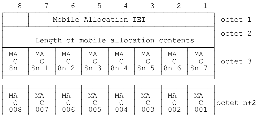
FIGURE 10.39/GSM 04.08 Mobile Allocation information element.
