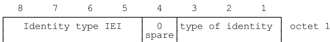
FIGURE 10.64/GSM 04.08 Identity Type information element
