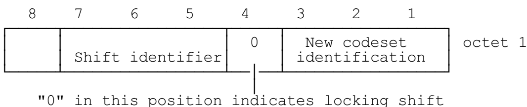
FIGURE 10.68/GSM 04.08 Locking shift element
