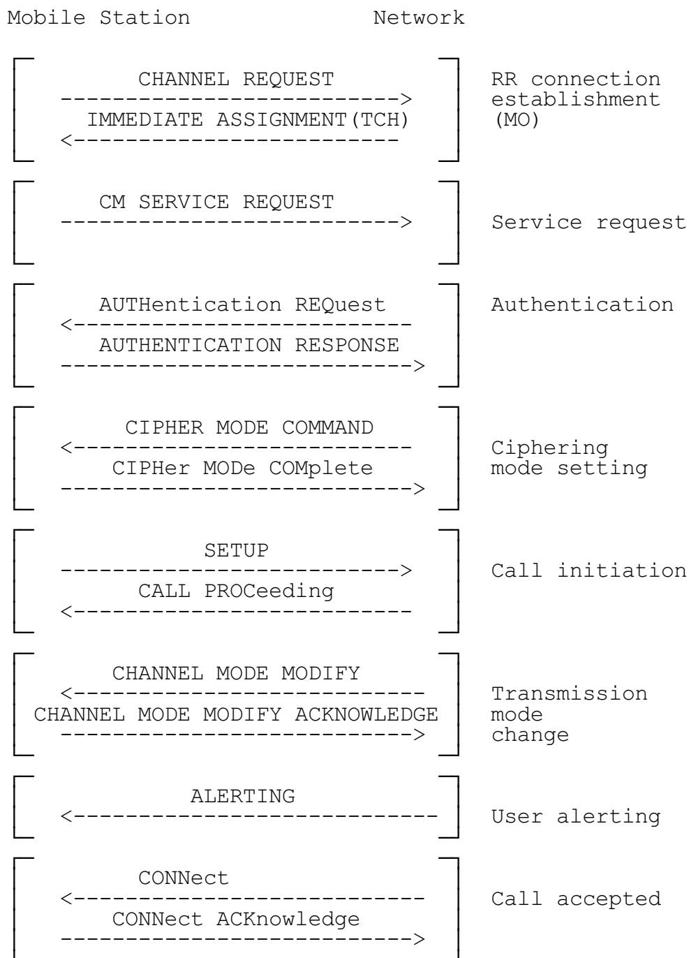
Figure 7.10c/GSM 04.08 Mobile originating call establishment with very early assignment
