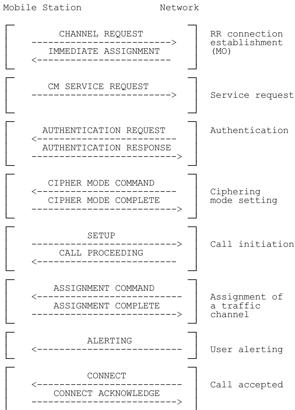
Figure 7.10a/GSM 04.08
