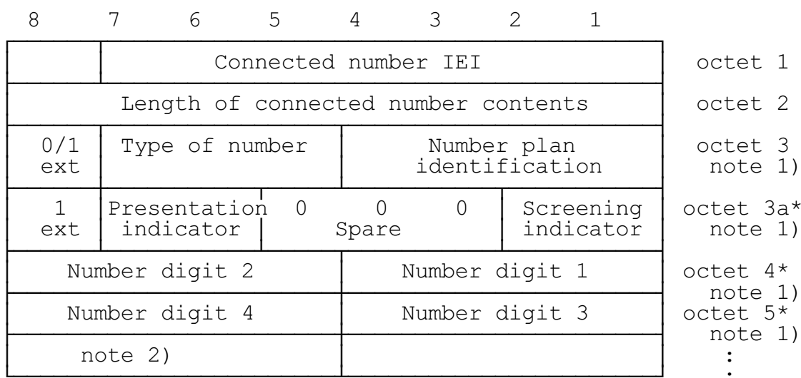
Figure 10.80/GSM 04.08
