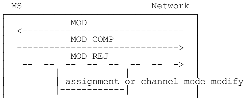
Figure 5.10b/GSM 04.08 In-call modification sequence initiated by network
