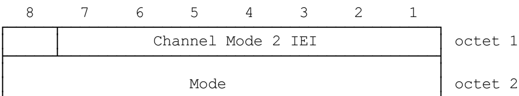
FIGURE 10.21/GSM 04.08 Channel Mode 2 information element
