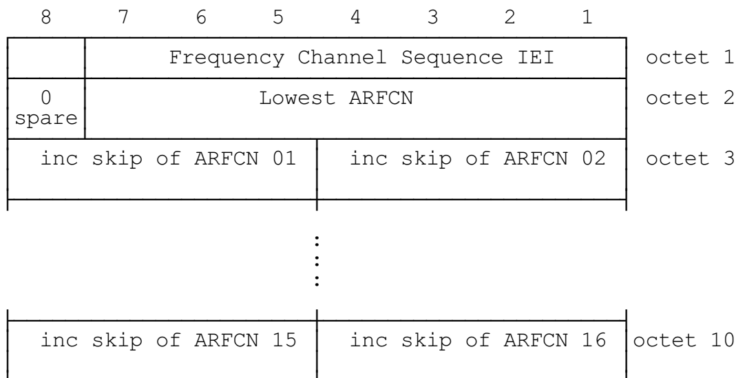
FIGURE 10.26/GSM 04.08 Frequency Channel Sequence information element
