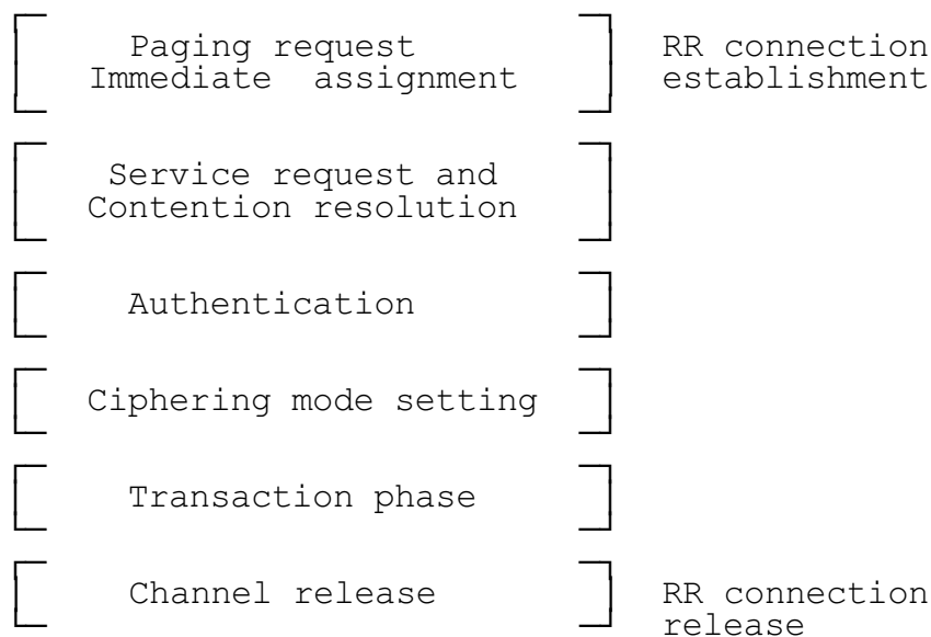
Figure 7.1/GSM 04.08 Components of structured procedures
