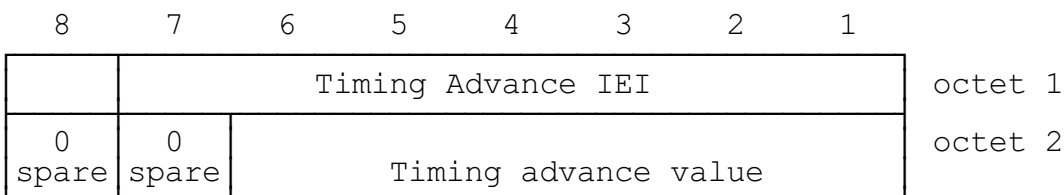
FIGURE 10.57/GSM 04.08 Timing Advance information element
