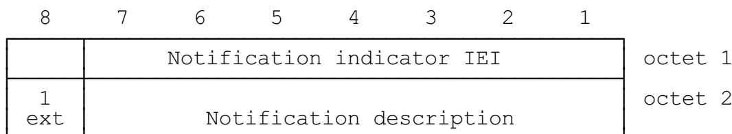
FIGURE 10.87/GSM 04.08 Notification indicator information element
