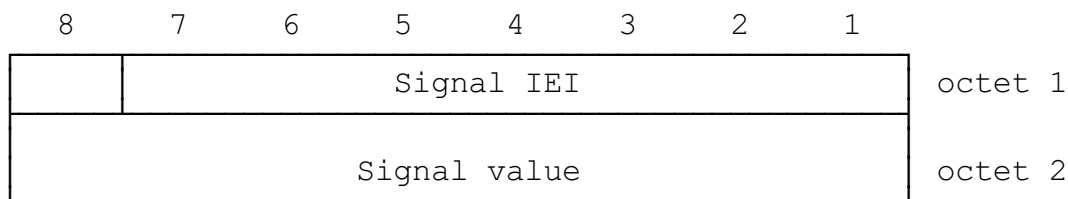
FIGURE 10.90/GSM 04.08 Signal information element
