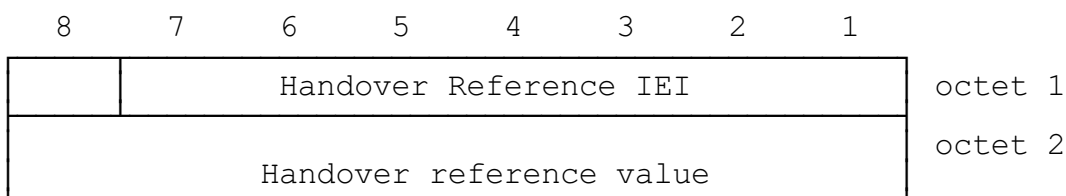
FIGURE 10.33/GSM 04.08 Handover Reference information element
