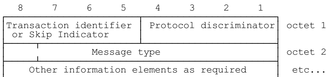
FIGURE 10.1/GSM 04.08 General message organization example
