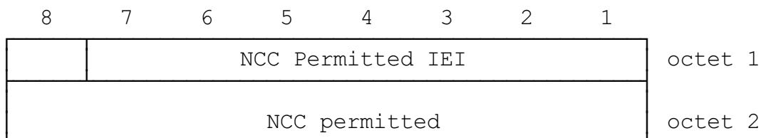
FIGURE 10.45/GSM 04.08 NCC Permitted information element
