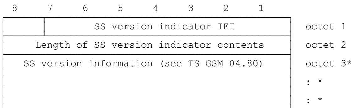
Figure 10.91/GSM 04.08
