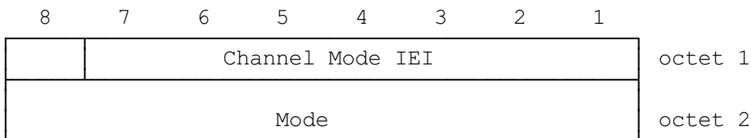
FIGURE 10.20/GSM 04.08 Channel Mode information element
