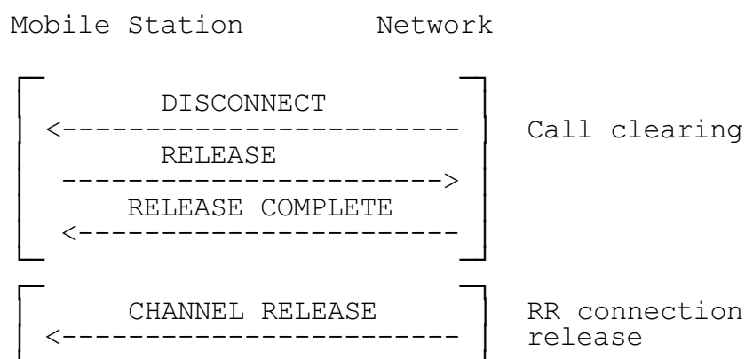
a) Call clearing initiated by the network
