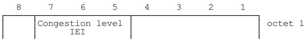
FIGURE 10.79/GSM 04.08 Congestion level information element
