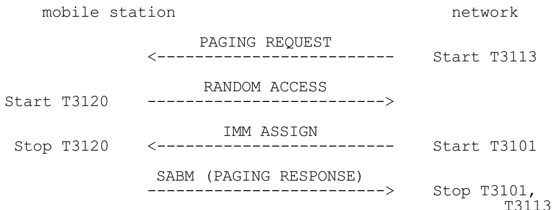
Figure 3.2/GSM 04.08 Paging sequence
