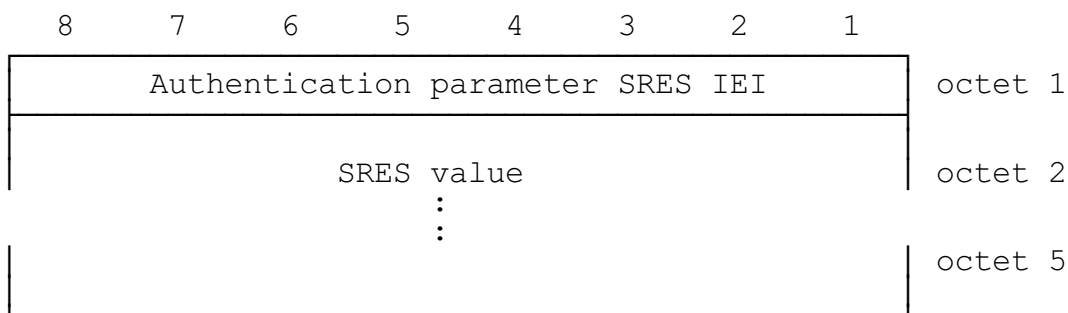
FIGURE 10.62/GSM 04.08 Authentication Parameter SRES information element
