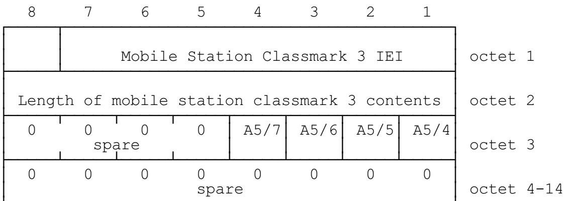
FIGURE 10.8/GSM 04.08 Mobile Station Classmark 3 information element
