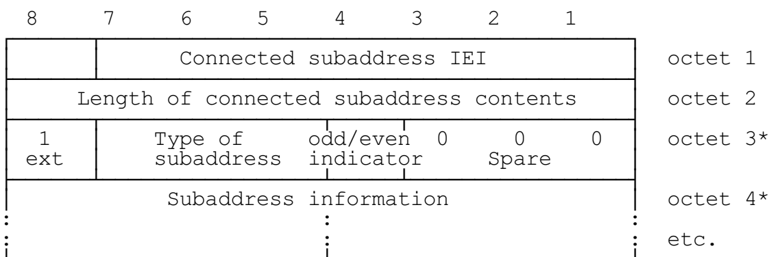
Figure 10.81/GSM 04.08
