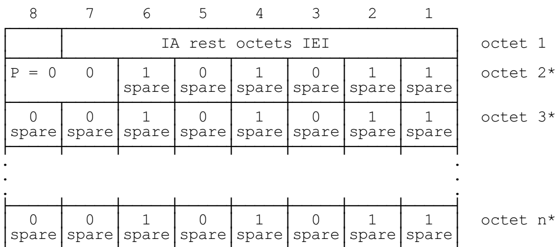
FIGURE 10.34/GSM 04.08 IA rest octets information element, P=00
