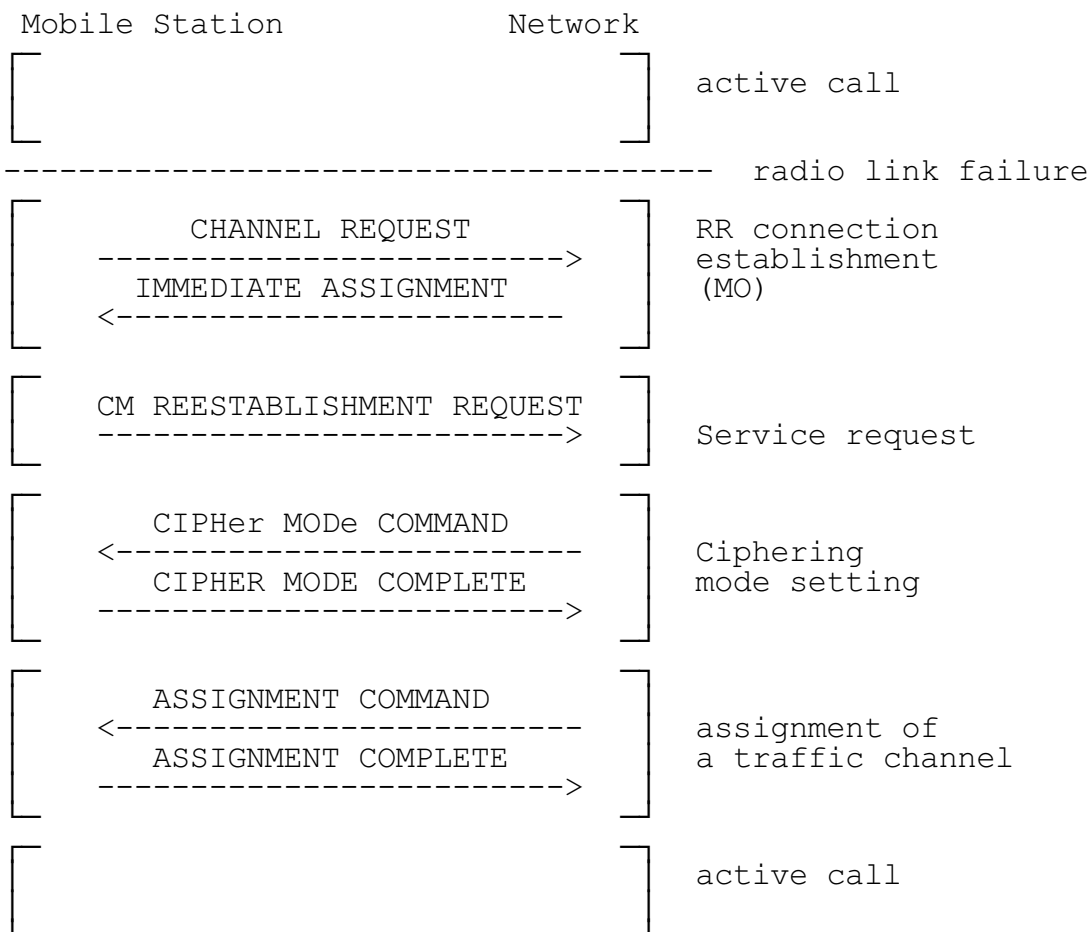
Figure 7.18/GSM 04.08 Call re-establishment
