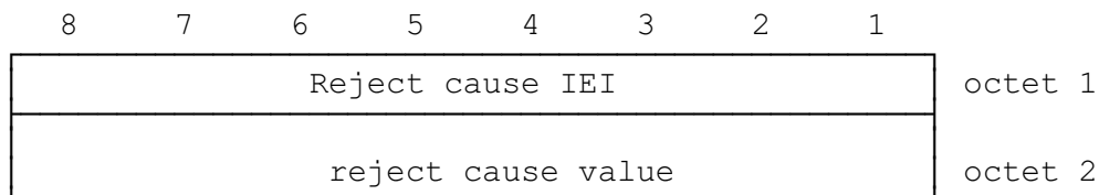
FIGURE 10.66/GSM 04.08 Reject Cause information element
