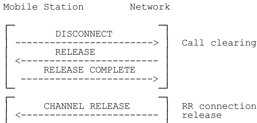
b) Call clearing initiated by the MS
