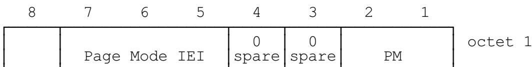
FIGURE 10.44/GSM 04.08 Page Mode information element
