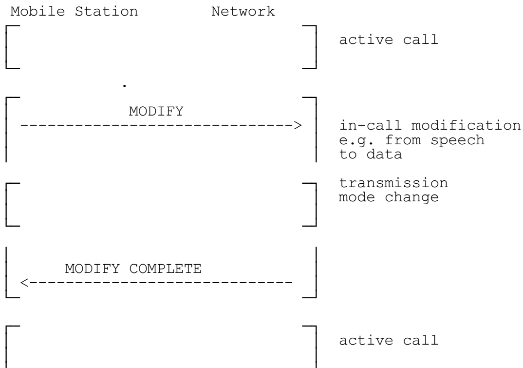
Figure 7.17/GSM 04.08 In-call modification
