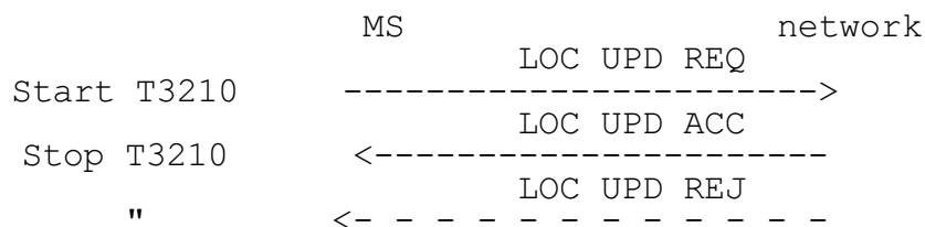
Figure 4.5/GSM 04.08 Location updating sequence
