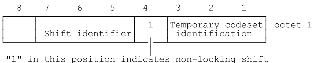
FIGURE 10.69/GSM 04.08 Non-locking shift element
