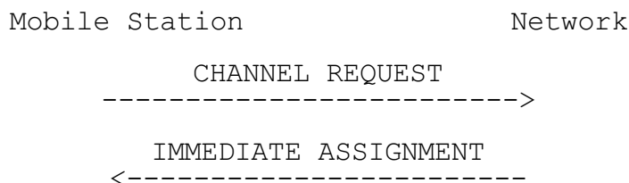
Figure 7.3/GSM 04.08 Immediate assignment
