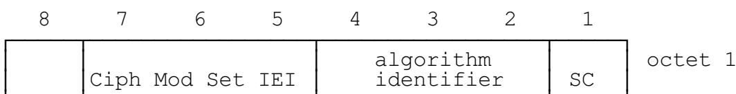
FIGURE 10.23/GSM 04.08 Cipher Mode Setting information element
