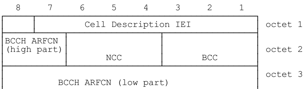
FIGURE 10.16/GSM 04.08 Cell Description information element
