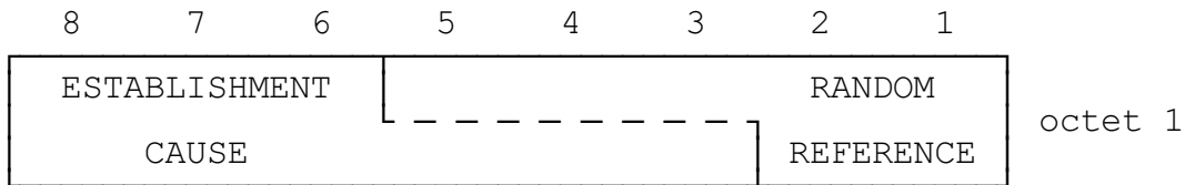
FIGURE 9.1/GSM 04.08 CHANNEL REQUEST message content
