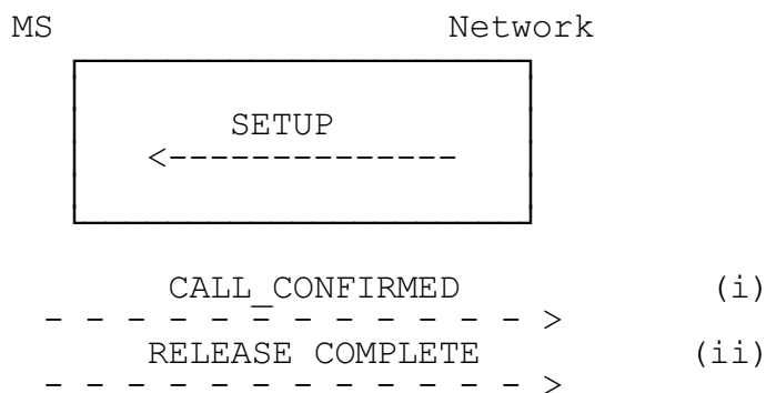
Figure 5.6/GSM 04.08 Mobile terminating call initiation and possible subsequent responses.
