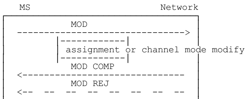
Figure 5.10a/GSM 04.08 In-call modification sequence initiated by MS
