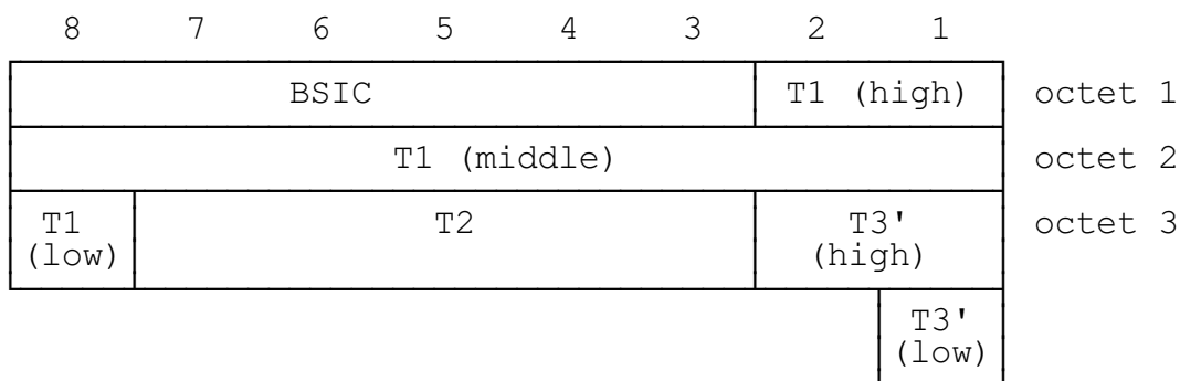
FIGURE 9.3/GSM 04.08 Frame synchronization information element
