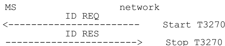
Figure 4.3/GSM 04.08 Identification sequence
