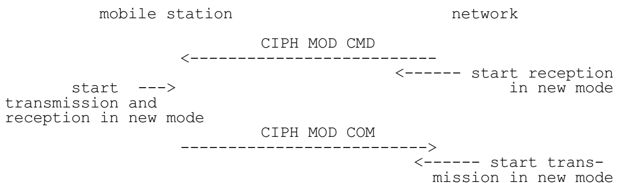
Figure 3.3/GSM 04.08 Cipherring mode setting sequence
