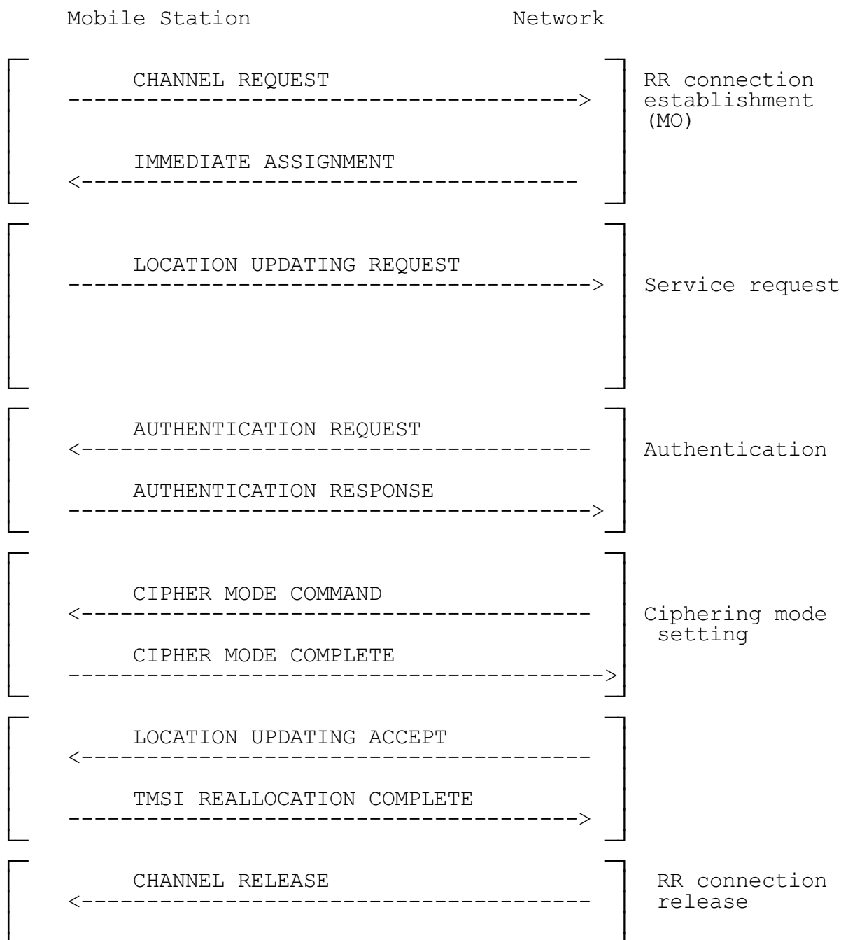
Figure 7.9/GSM 04.08 Location updating: successful case
