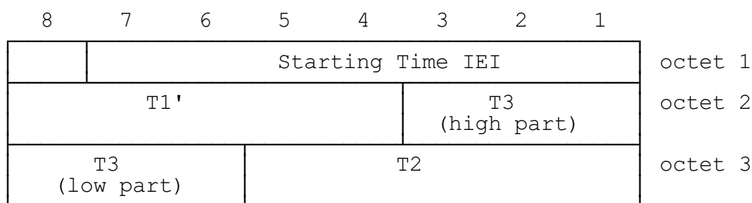
FIGURE 10.55/GSM 04.08 Starting Time information element
