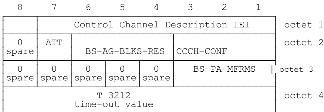
FIGURE 10.25/GSM 04.08 Control Channel Description information element
