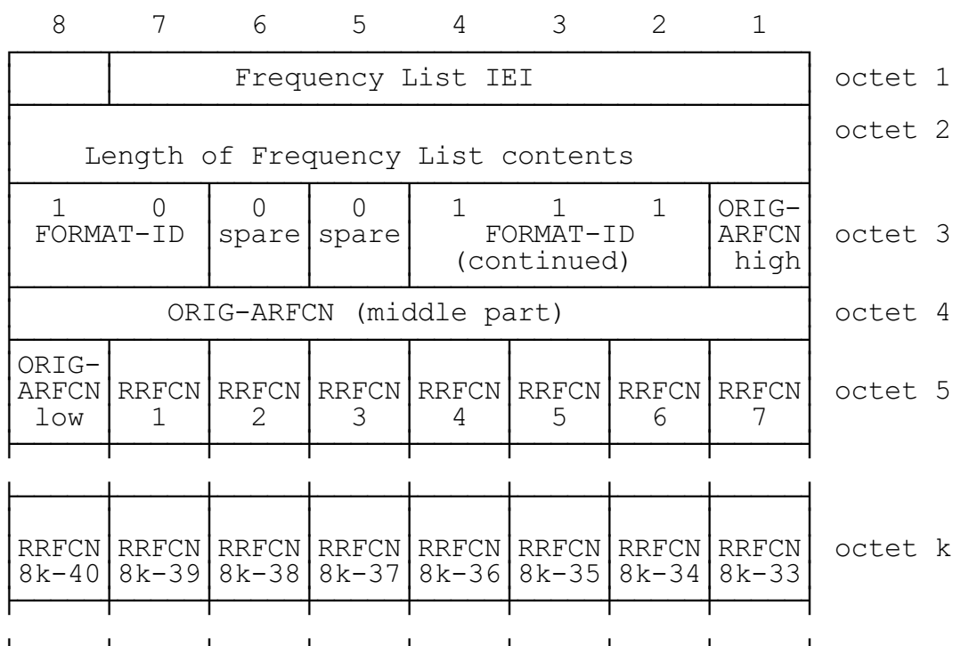
FIGURE 10.32/GSM 04.08 Frequency List information element, variable bit map format
