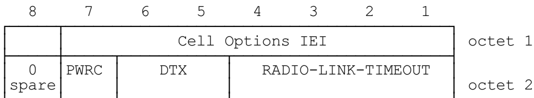
FIGURE 10.17/GSM 04.08 Cell Options information element
