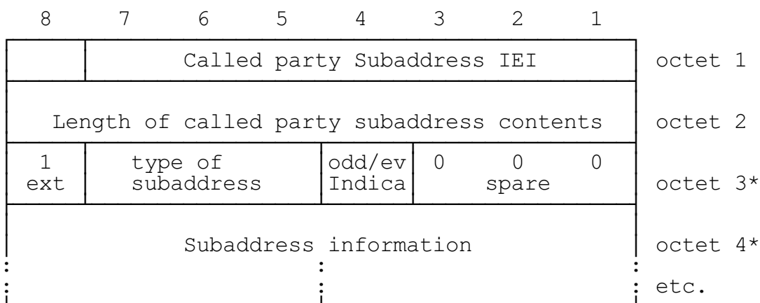
FIGURE 10.74/GSM 04.08 Called party subaddress
