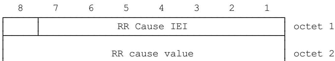
FIGURE 10.49/GSM 04.08 RR Cause information element
