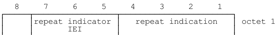
FIGURE 10.89/GSM 04.08 Repeat indicator information element
