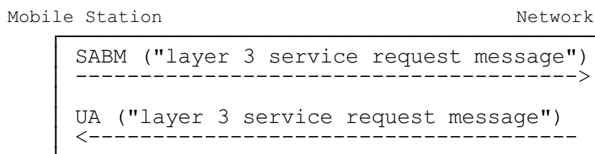
Figure 3.1/GSM 04.08 Service request and contention resolution
