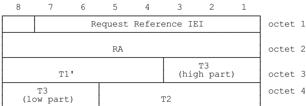
FIGURE 10.48/GSM 04.08 Request Reference information element
