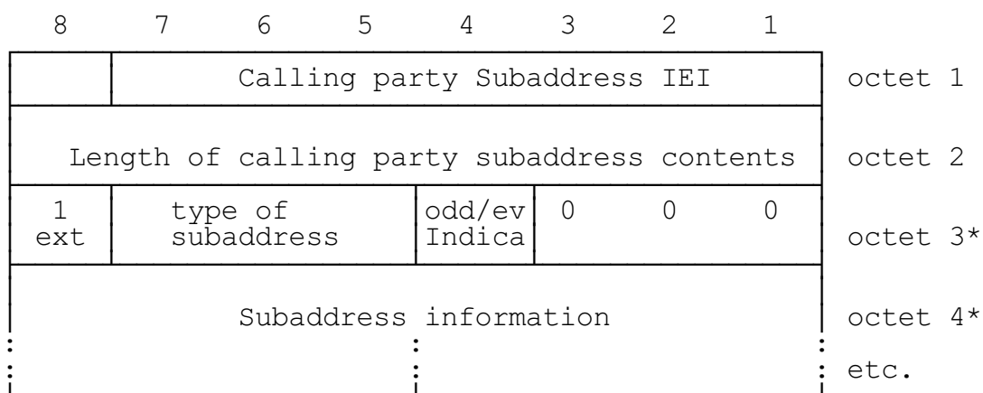
FIGURE 10.76/GSM 04.08 Calling party subaddress
