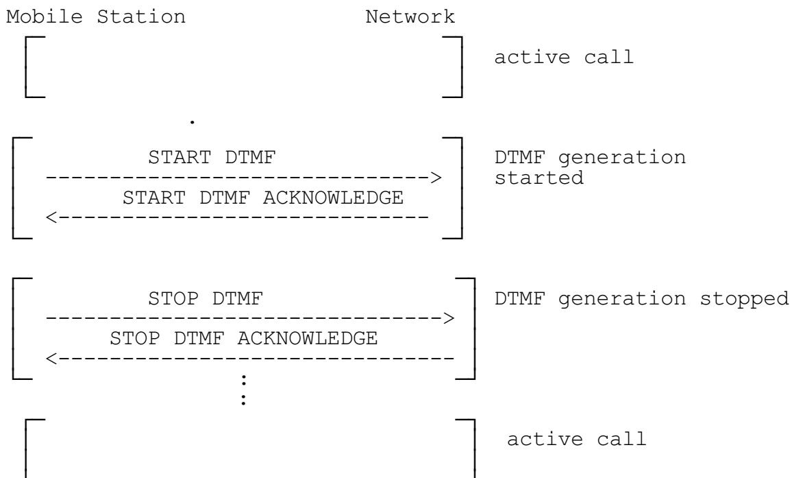
Figure 7.13/GSM 04.08 DTMF protocol control
