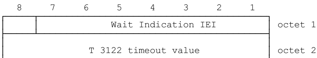
FIGURE 10.60/GSM 04.08 Wait Indication information element
