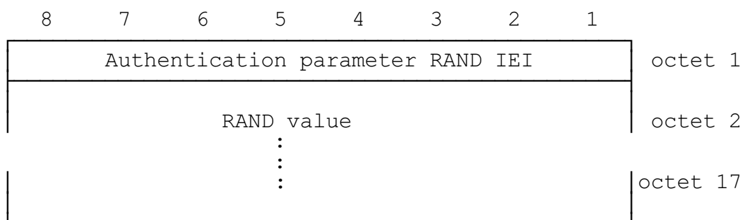
FIGURE 10.61/GSM 04.08 Authentication Parameter RAND information element
