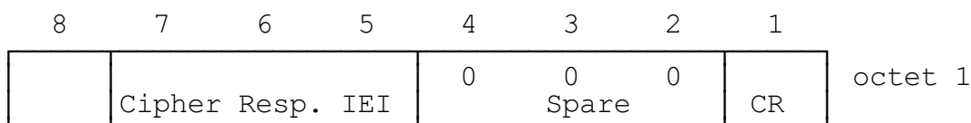
FIGURE 10.24/GSM 04.08 Cipher Response information element
