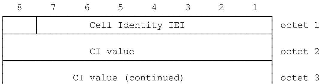
FIGURE 10.2/GSM 04.08 Cell Identity information element
