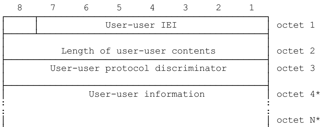
FIGURE 10.92/GSM 04.08 User-user information element
