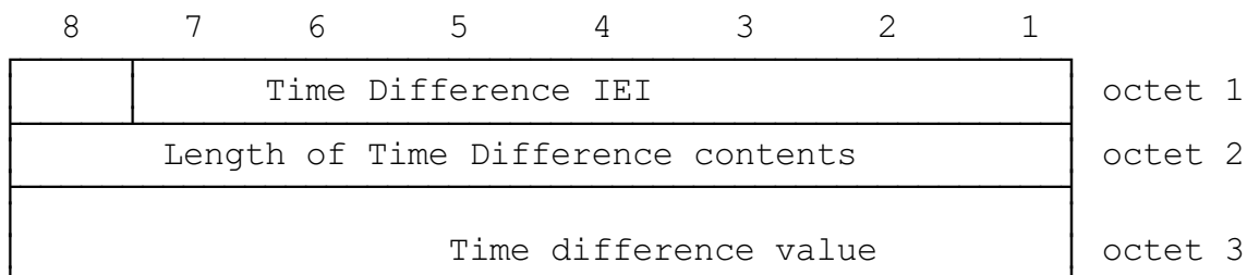
FIGURE 10.58/GSM 04.08 Time Difference information element
