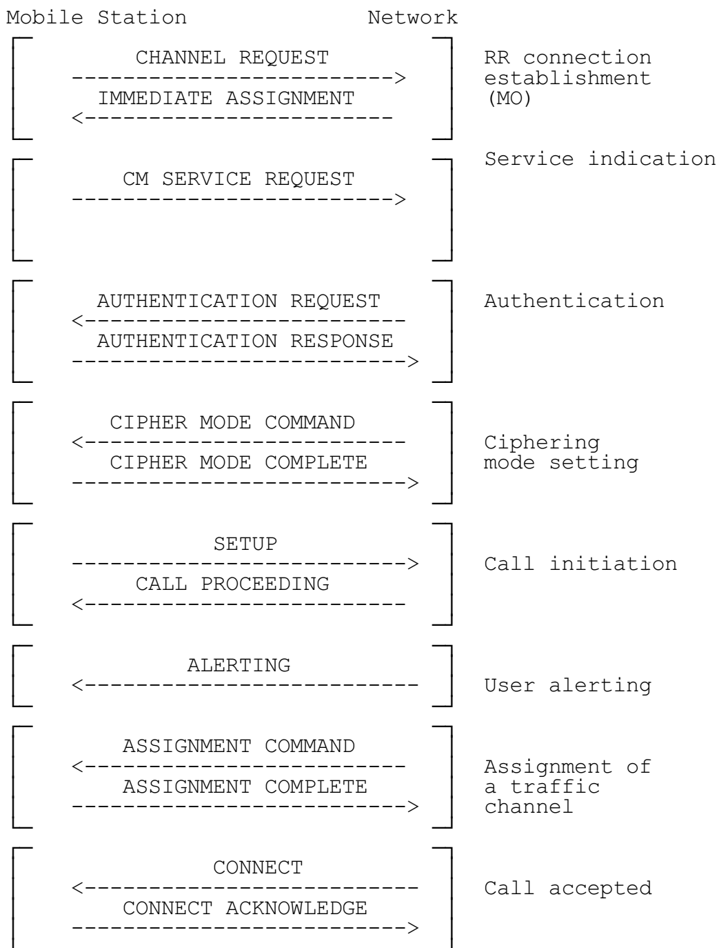
Figure 7.10b/GSM 04.08 Mobile originating call establishment with OACSU (late assignment)
