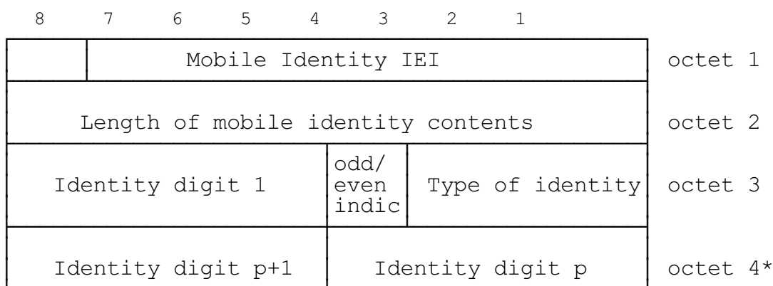
FIGURE 10.5/GSM 04.08 Mobile Identity information element
