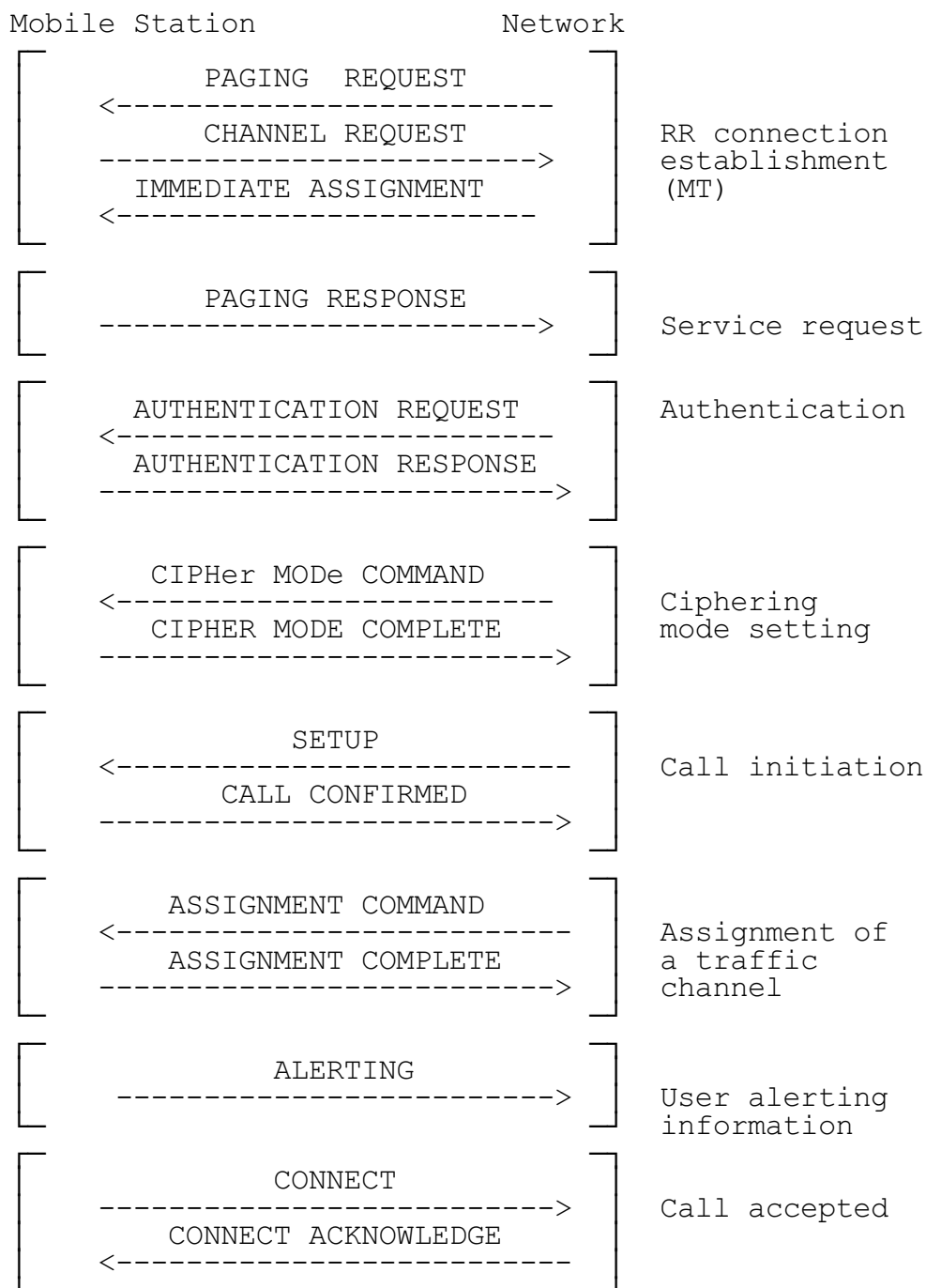
Figure 7.11a/GSM 04.08 - Mobile terminating call establishment without OACSU (early assignment)
