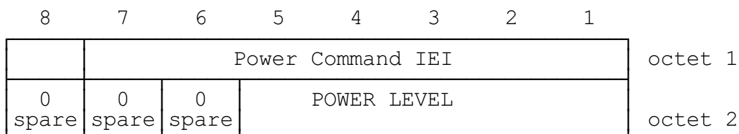
FIGURE 10.46/GSM 04.08 Power Command information element
