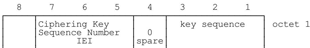
FIGURE 10.3/GSM 04.08 Cipherring Key Sequence Number information element
