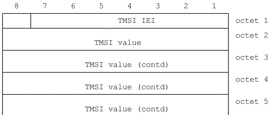
FIGURE 10.59/GSM 04.08 TMSI information element
