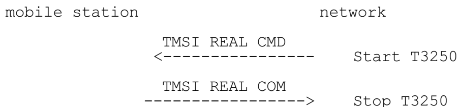
Figure 4.1/GSM 04.08 TMSI reallocation sequence
