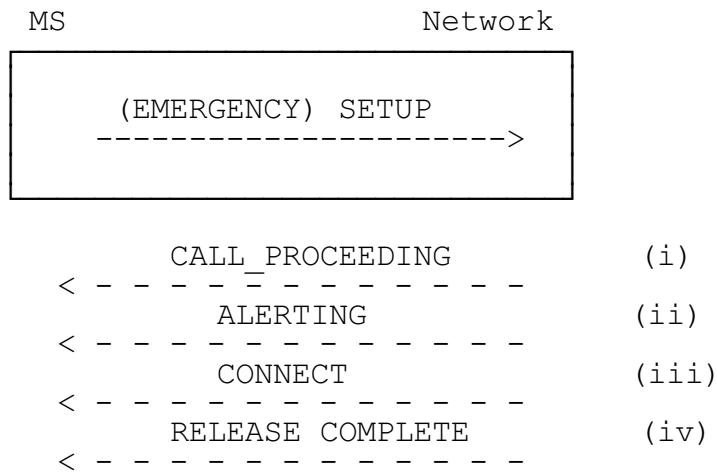
Figure 5.2/GSM 04.08 Mobile originated call initiation and possible subsequent responses.
