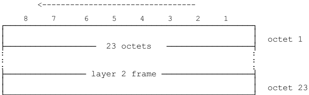
Figure 7.4: FACCH/SDCCH uplink block format
