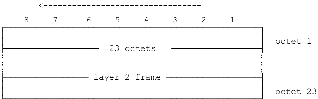
Figure 7.3: FACCH/SDCCH/BCCH/CCCH/CBCH downlink block format
