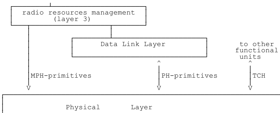
Figure 2.1: Interfaces with the Physical Layer
