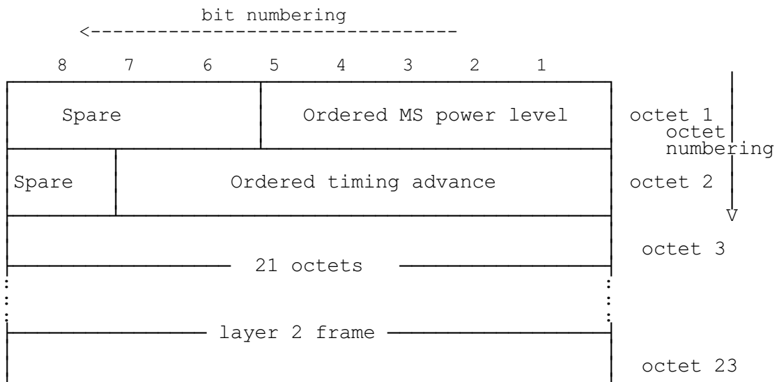
Figure 7.1: SACCH downlink block format
