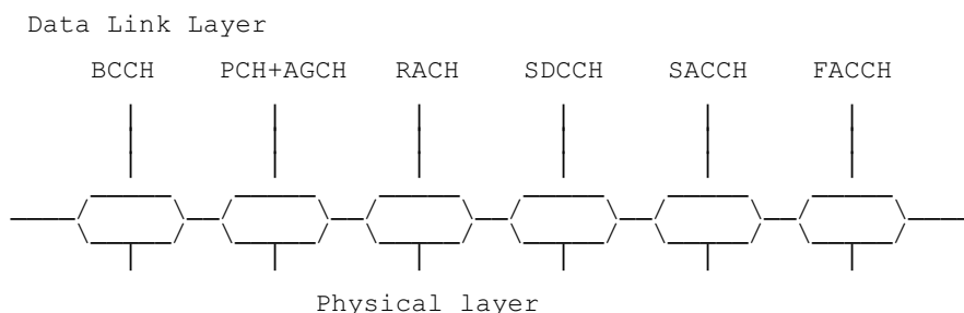
Figure 3.2: SAPs between the physical layer and the data link layer in the MS
