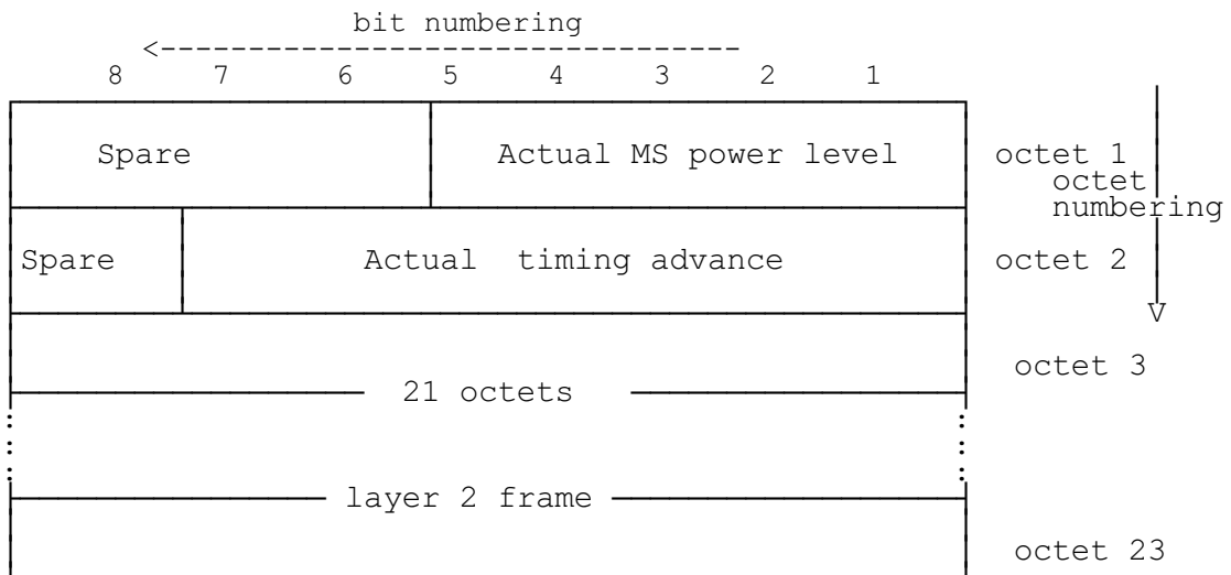
Figure 7.2: SACCH uplink block format
