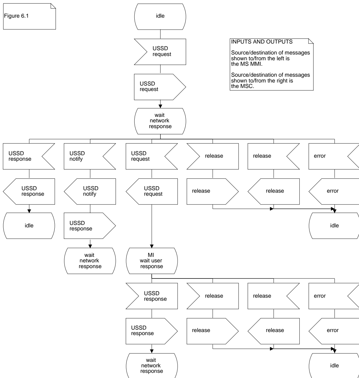
Figure 6.1: Mobile initiated USSD at MS
