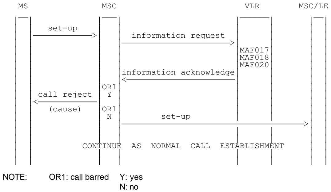
Figure 1.10: Information flow for barring of outgoing calls
