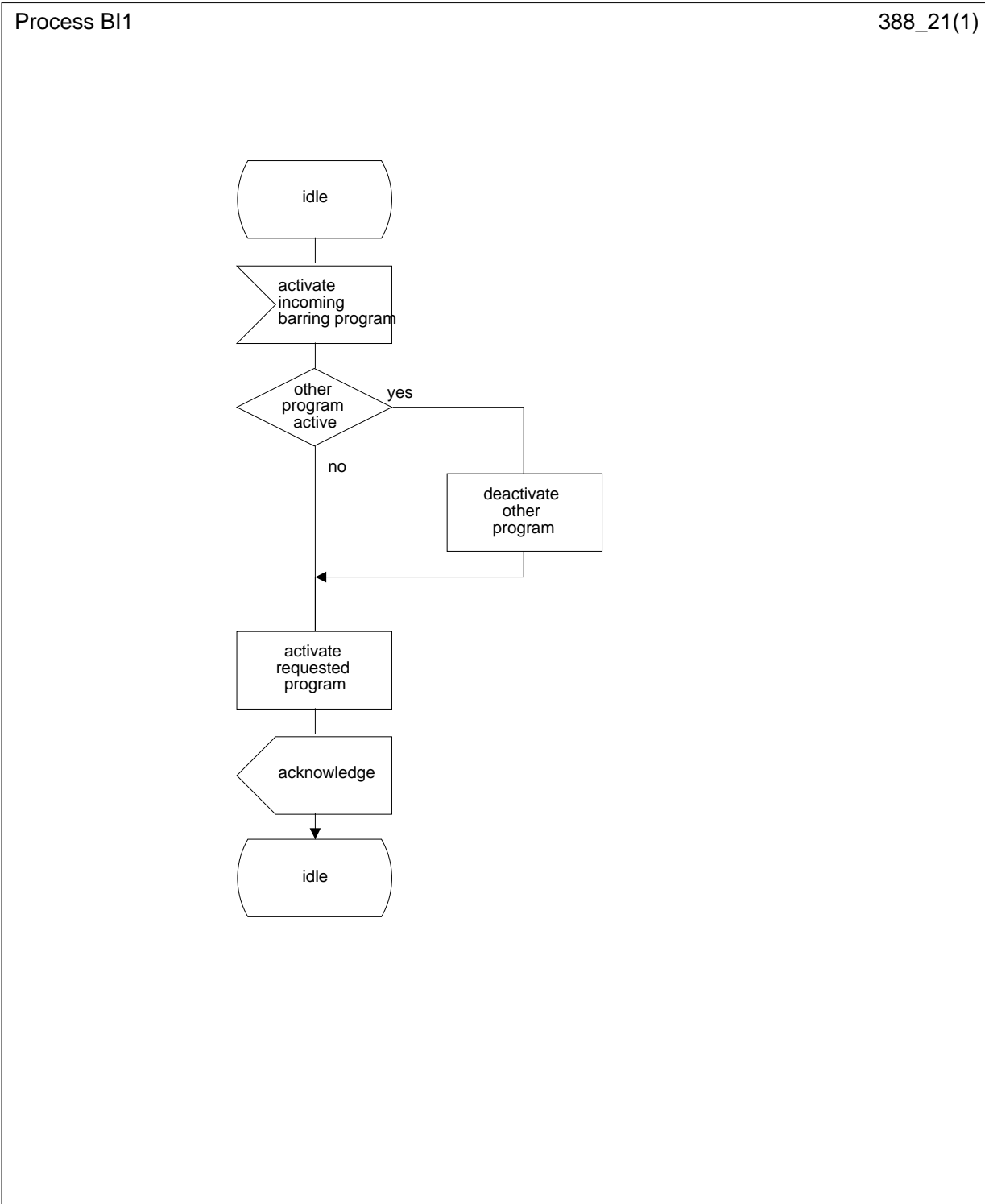
Figure 2.1: B11 Interaction between call barring programs
