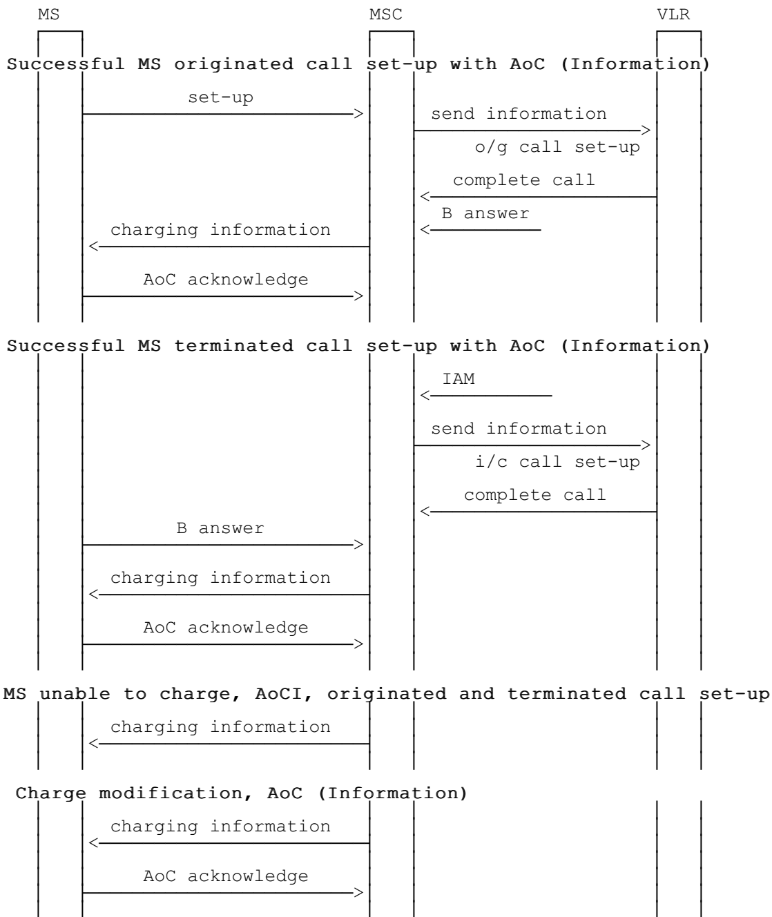
Figure 1.3: Information flow for Advice of Charge (Information)
