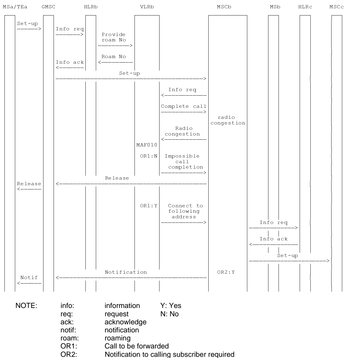
Figure 4.16: Information flow for call forwarding on mobile subscriber not reachable in case of radio congestion (to mobile station) (re-routing by VLR)
