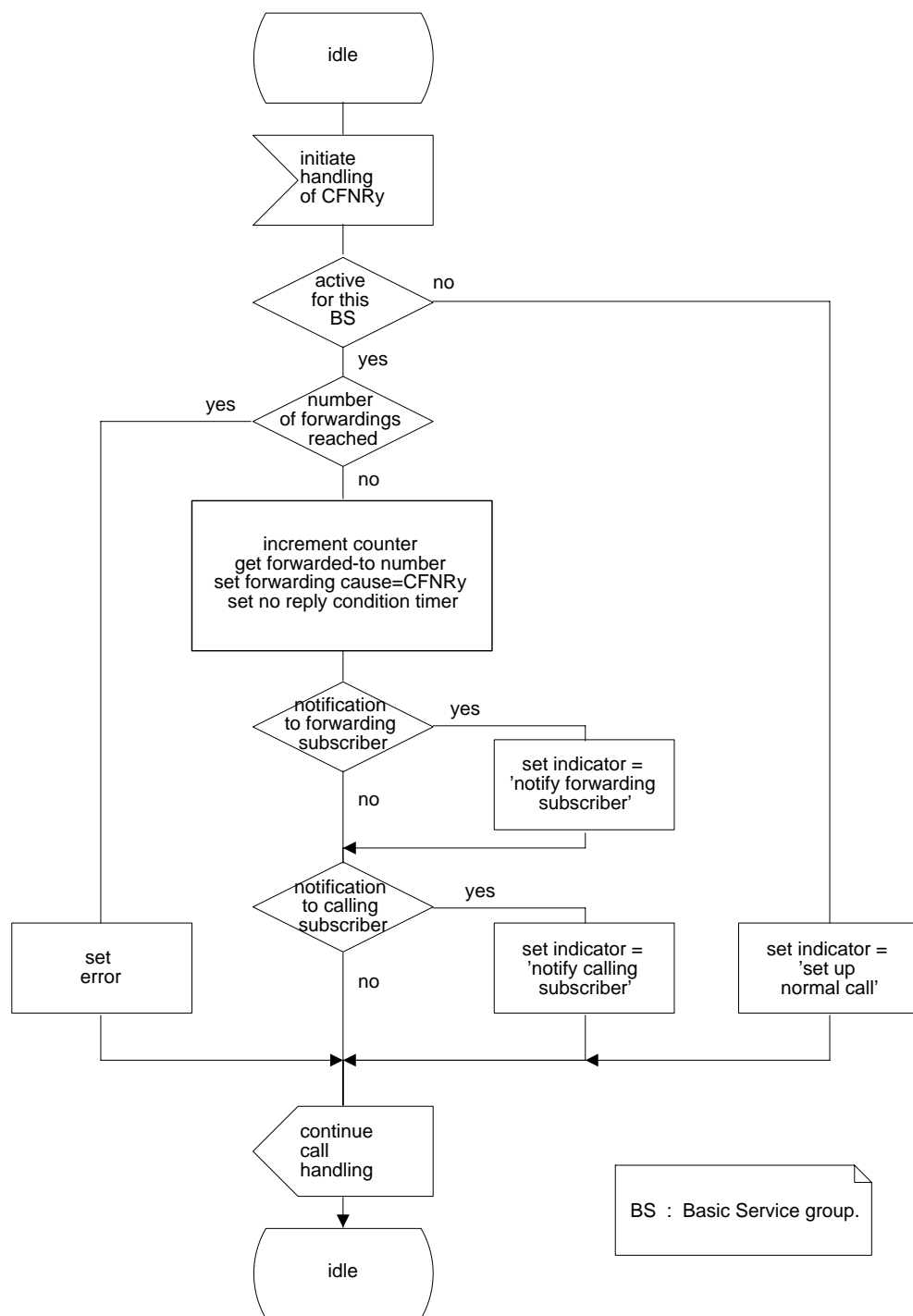
Figure 3.10: MAF008 Call forwarding on no reply authorizations examination (VLR)
