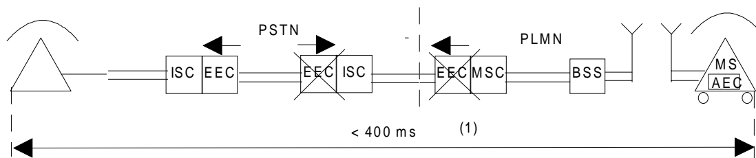
Call from PSTN to PLMN
