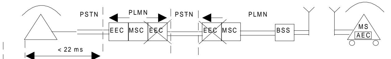
Call from PSTN to PLMN with re-route at MSC and via PSTN
