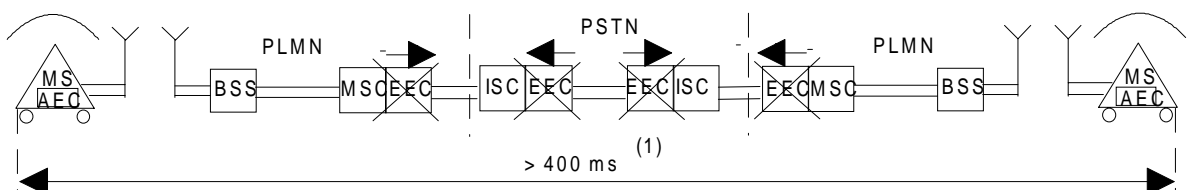
Call from PLMN to PLMN
