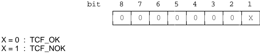
Figure A.13/03.46: Information field content of a TCF element
