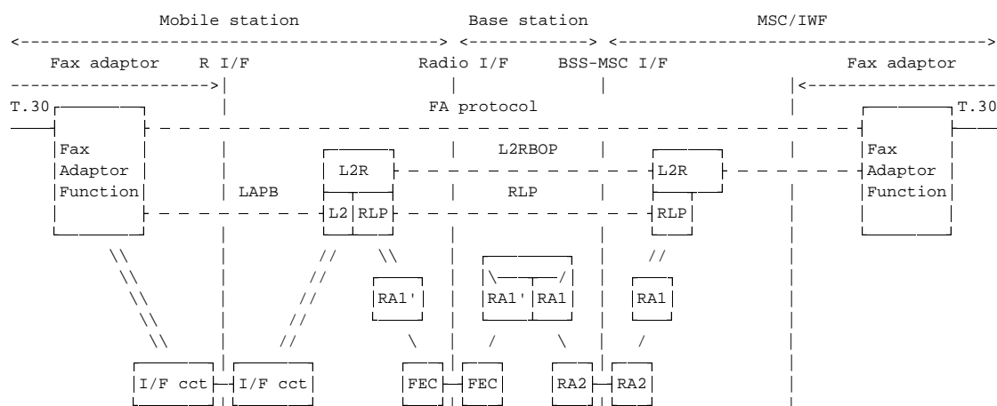
Figure 5/03.46: Protocol model for non-transparent support
