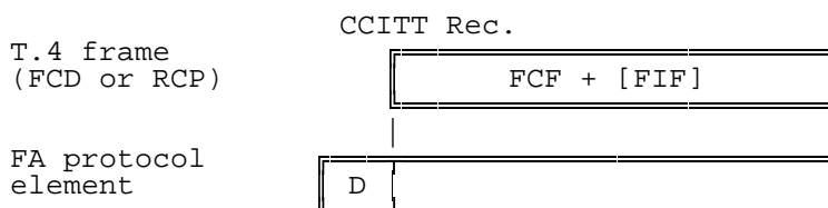
Figure A.12/03.46: Information field content of an error correction fax data element
