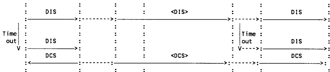
Figure II.10/03.46: Mobile terminated facsimile transmission - error recovery (example)
