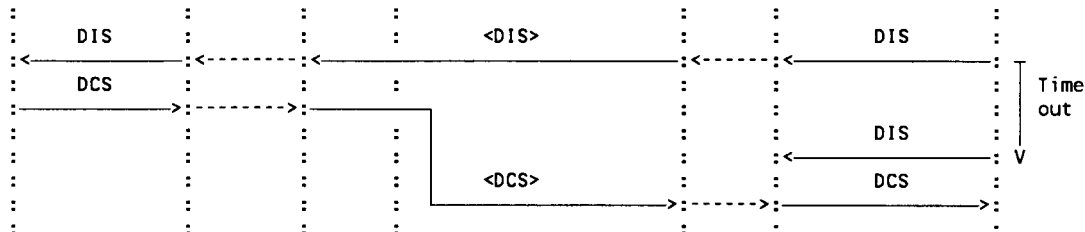
Figure II.9/03.46: Mobile originated facsimile transmission - error recovery (example)
