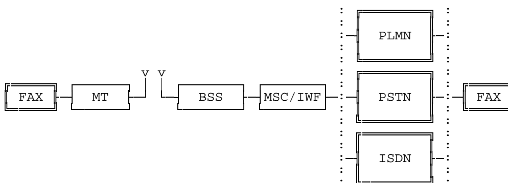
Figure 1/03.46: Network architecture
