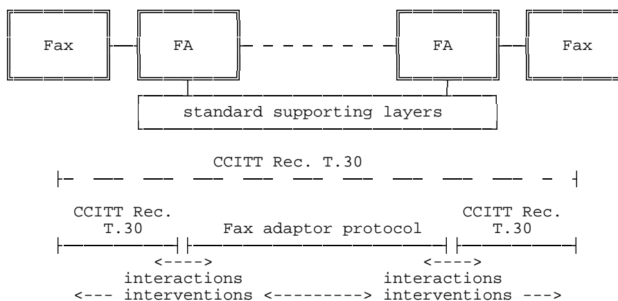
Figure 6/03.46: Communication model
