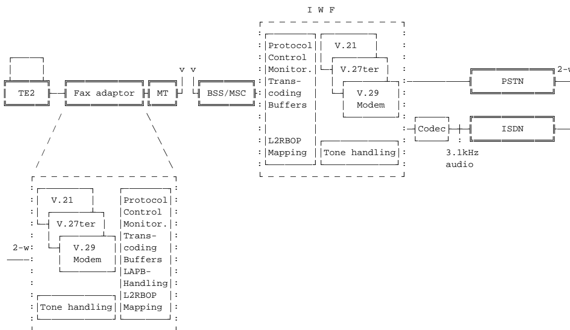
Figure 7/03.46: Network interworking
