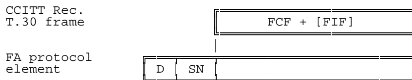
Figure A.10/03.46: Information field content of a BCS element
