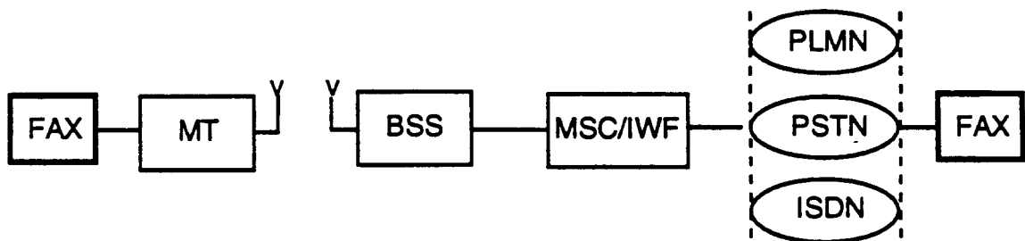
Fig. 1/03.45 Network architecture
