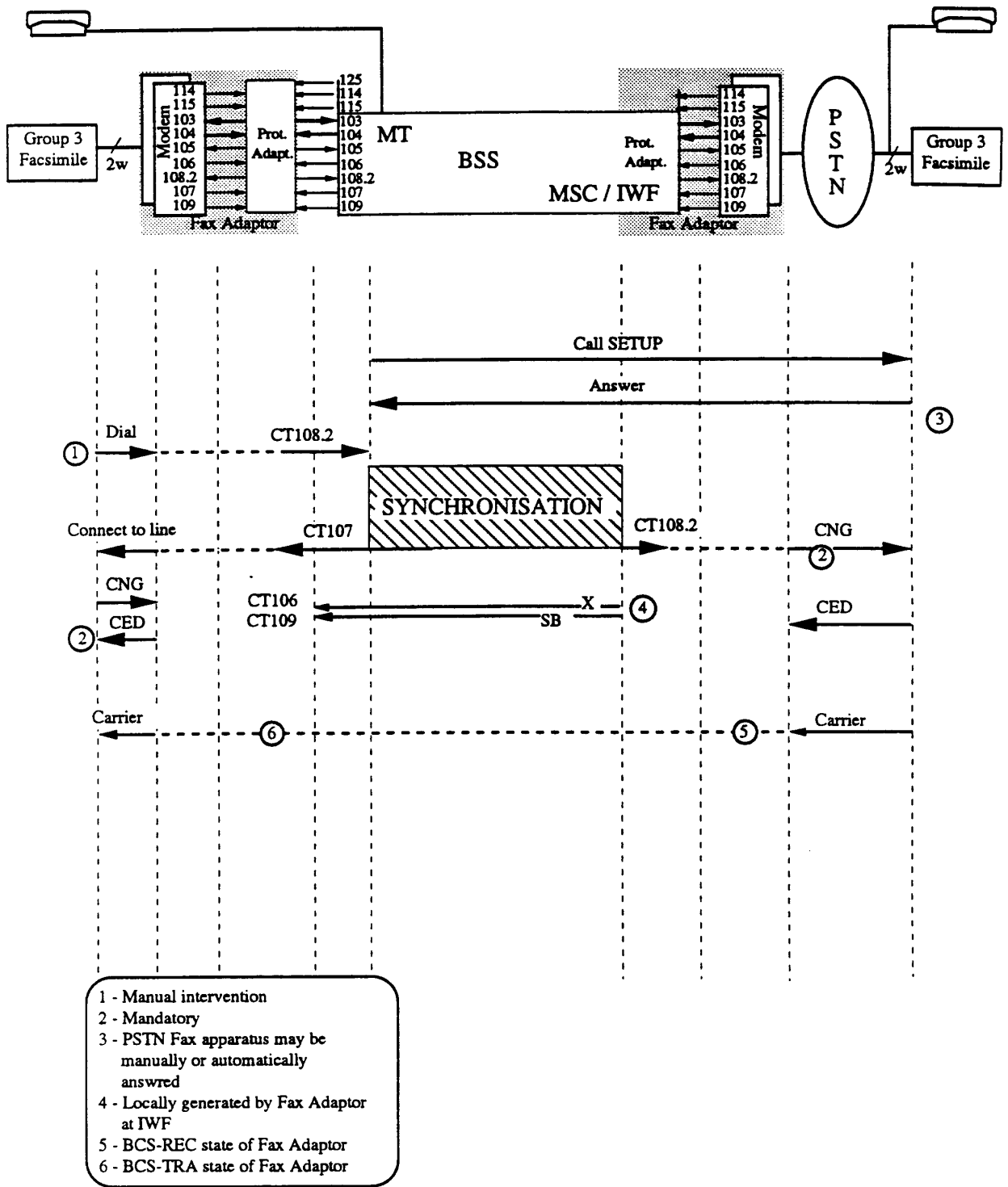
Fig. II-9/03.45 - Mobile Originated Call - Manual Calling
