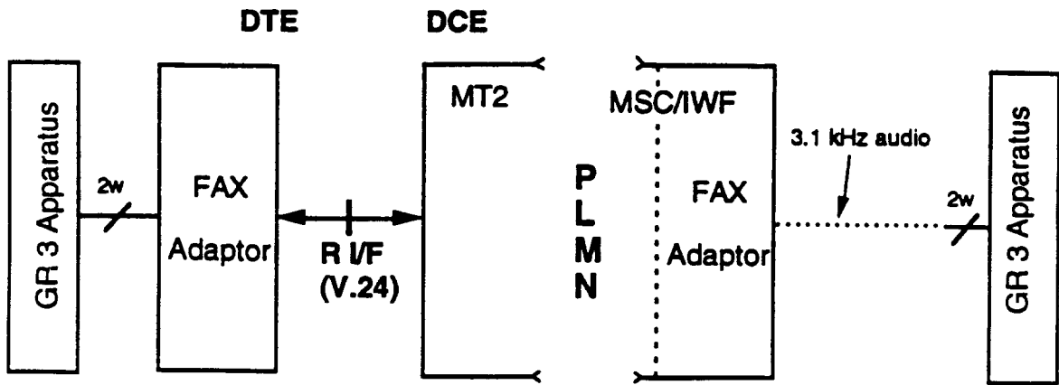
Fig.4a/03.45 Standard Teleservice connection
