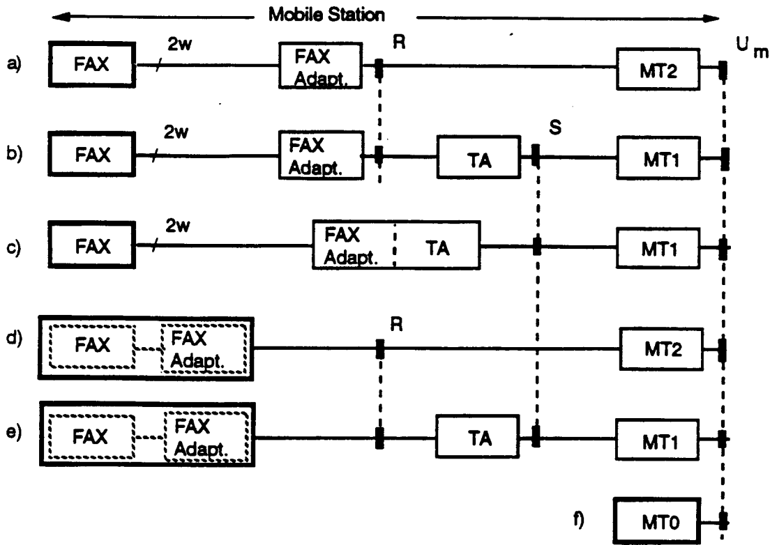
Fig. 2/03.45 Reference configurations
