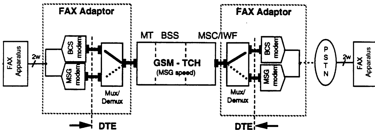
Fig.6/03.45 Fax Adaptor working principle
