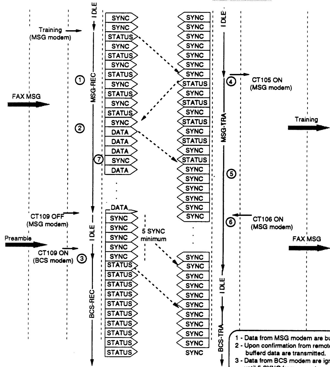
Fig. II-3/03.45 - Mobile originated facsimile transmission - MSG phase (7.2 kbit/s MSG speed)
