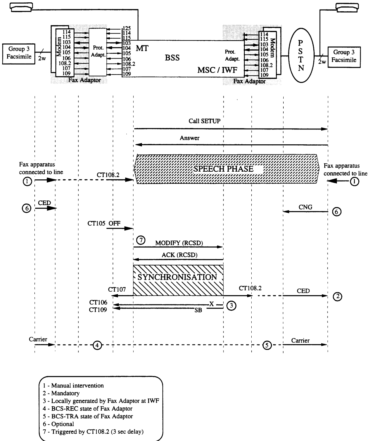
Fig. II-7b/03.45 - Mobile Originated Call - Speech then Fax (Data Call Direction is Mobile Terminated)
