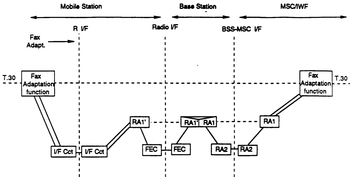
Fig. 5/03.45 Information transfer protocol model
