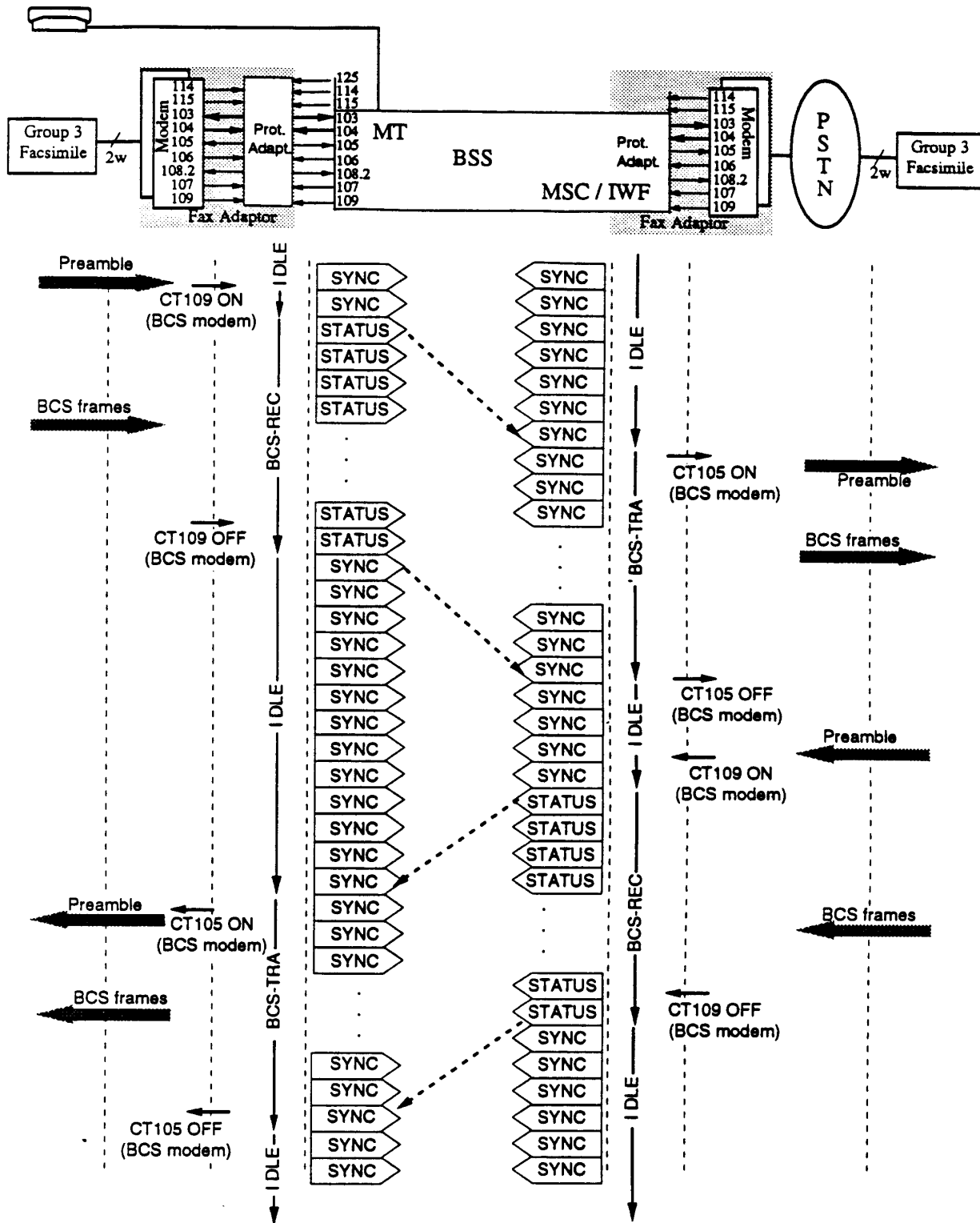
Fig. II-1/03.45 - Mobile originated facsimile transmission - Typical BCS phase (command/response)
