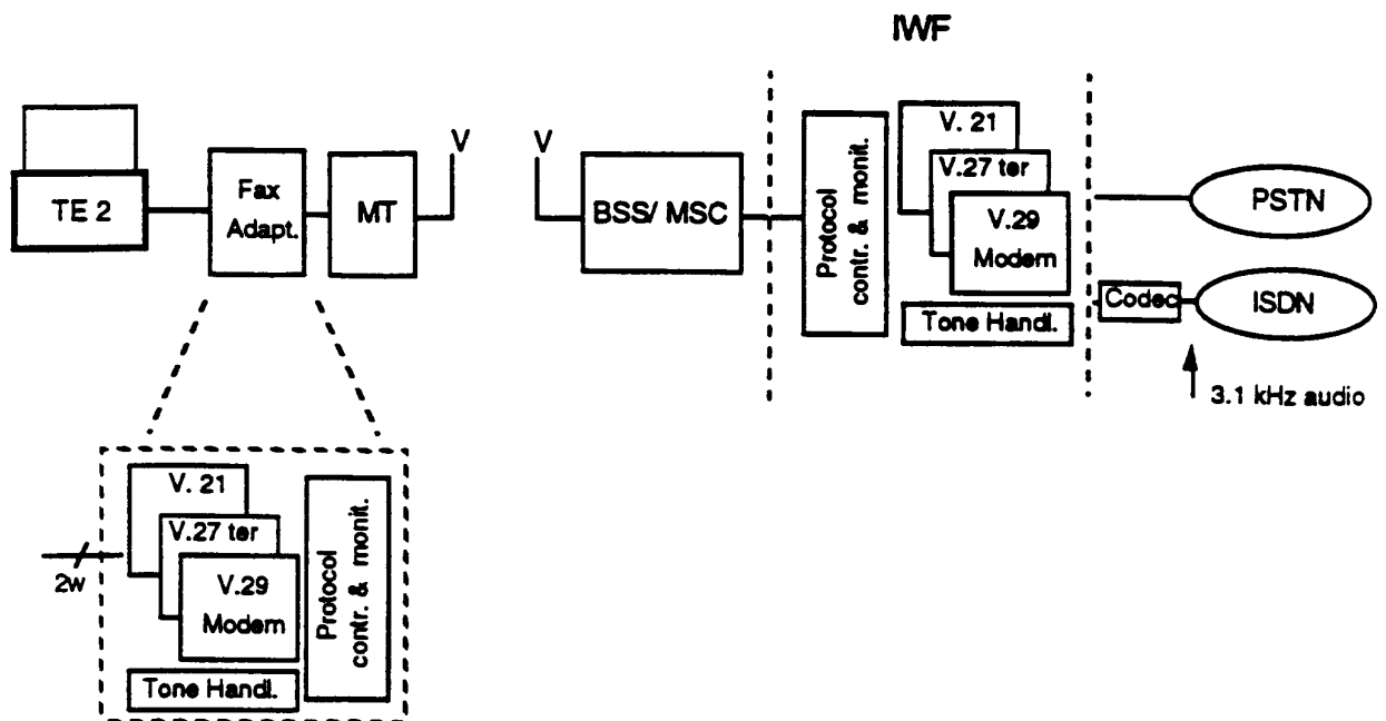
Fig.8/03.45 Network interworking
