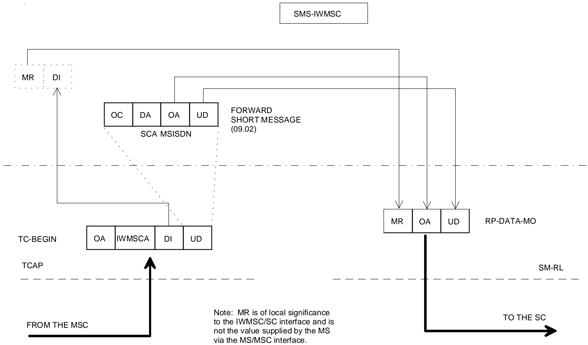
Figure 3.3: Mobile originated short message
