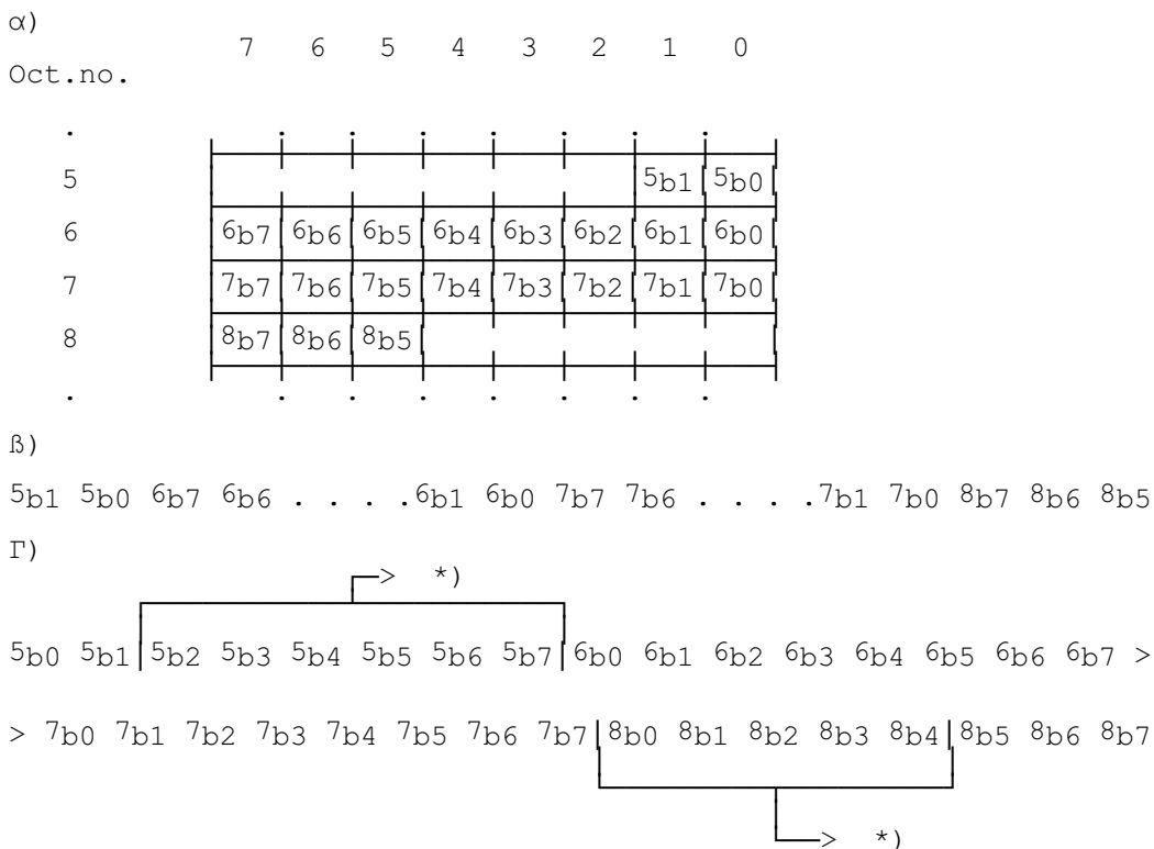
Figure 03.40/8: 21 bits from the octets 5, 6, 7, and 8 in a short message α) will represent an integer as shown in β), and will be transmitted in an order as shown in Γ)
