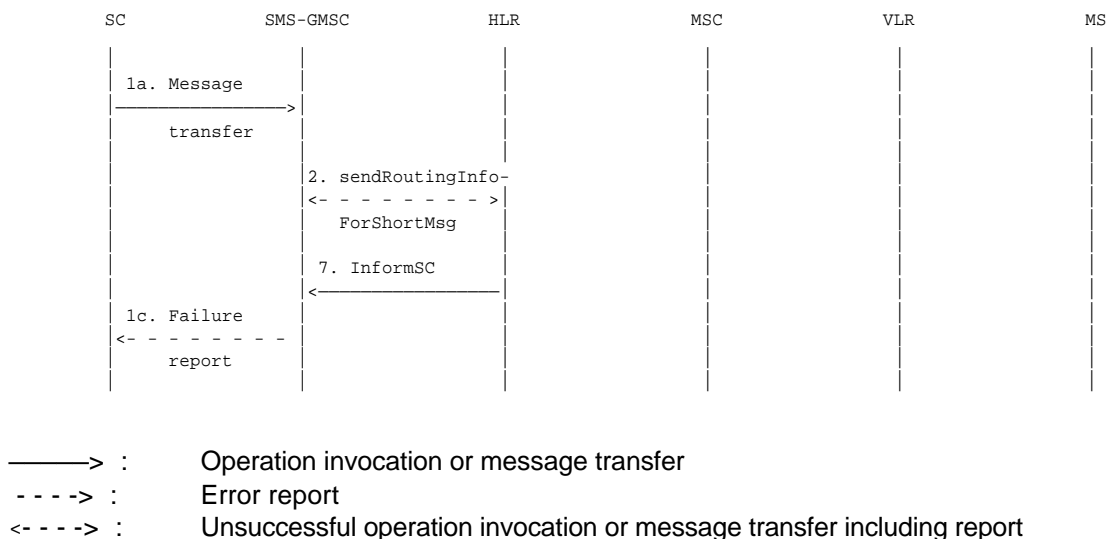
Figure 03.40/15c): Short message transfer attempt failing due to negative outcome of HLR information retrieval
