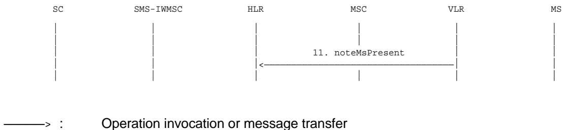
Figure 03.40/20b: The alert procedure when the MS becomes reachable, MNRF is set and MCEF is set
