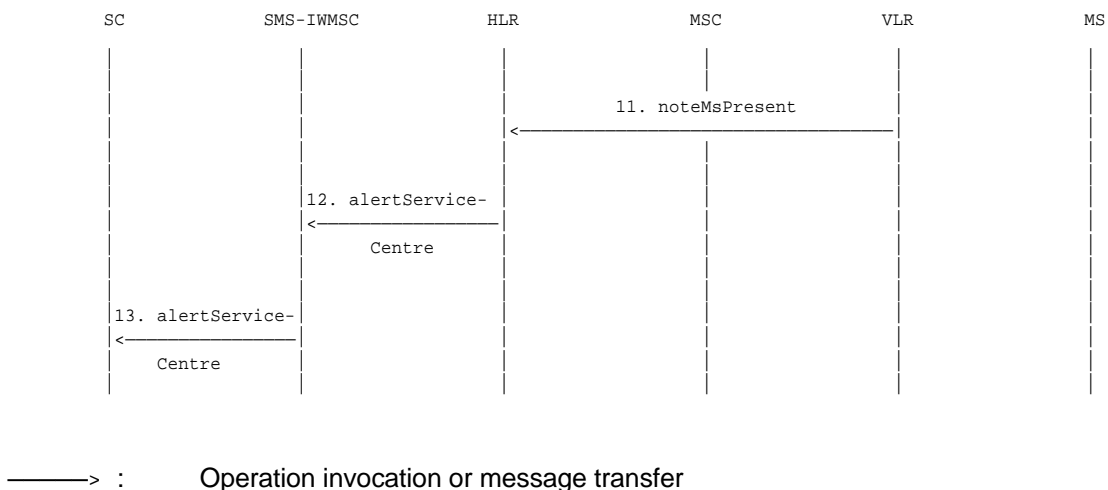
Figure 03.40/20a: The alert procedure when the MS becomes reachable, MNRF is set and MCEF is not set
