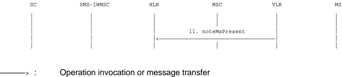
Figure 03.40/20b: The alert procedure when the MS becomes reachable, MNRF is set and MCEF is set.
