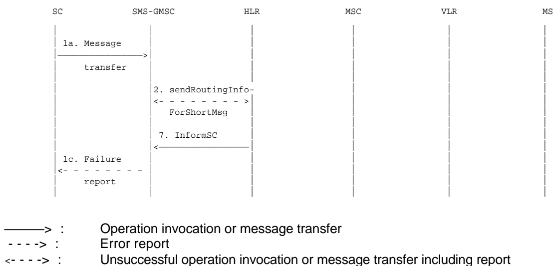
Figure 03.40/15c): Short message transfer attempt failing due to negative outcome of HLR information retrieval.
