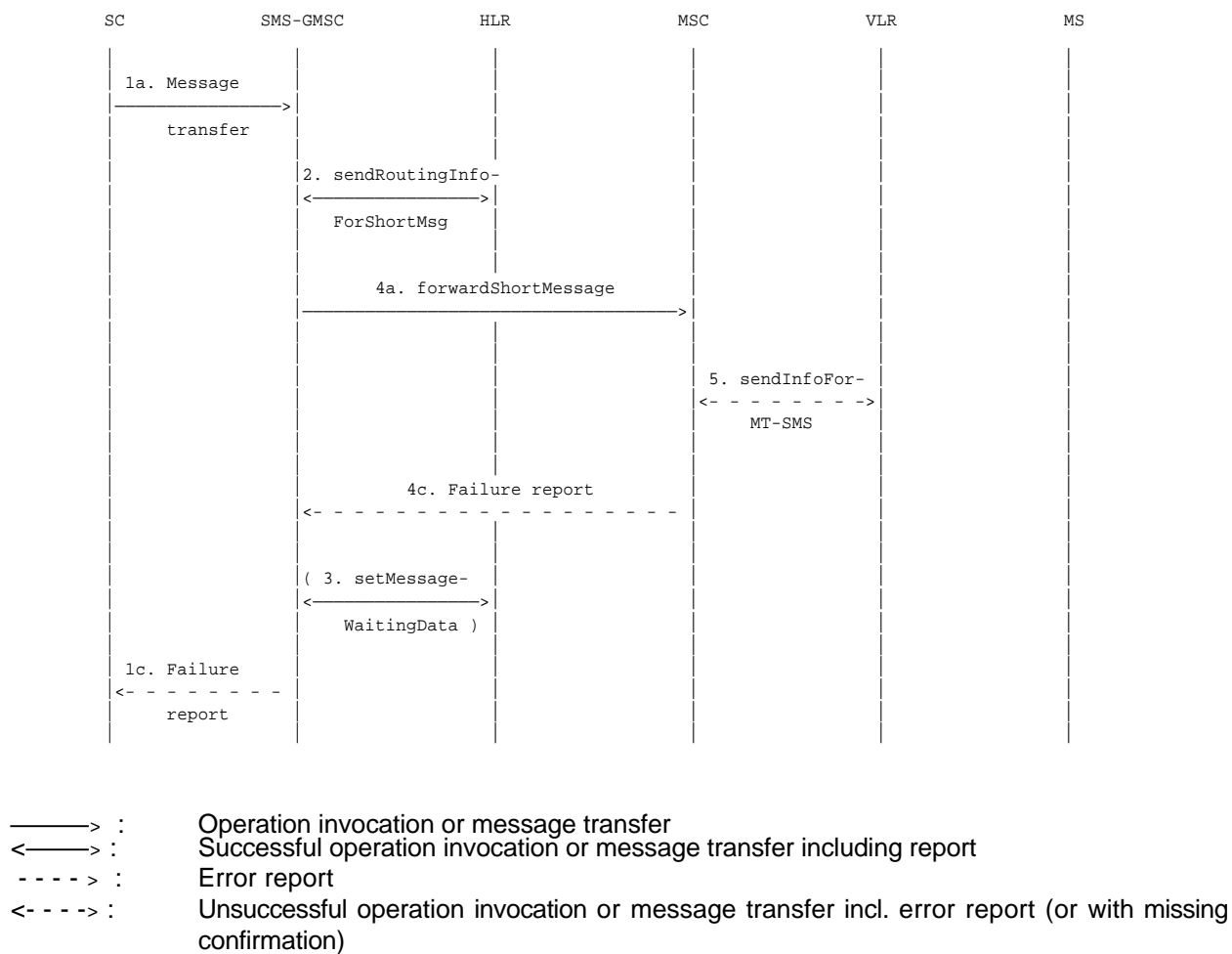
Figure 03.40/15e): Short message transfer attempt failing due to negative outcome of VLR information retrieval.
