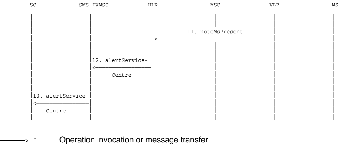
Figure 03.40/20a: The alert procedure when the MS becomes reachable, MNRF is set and MCEF is not set.
