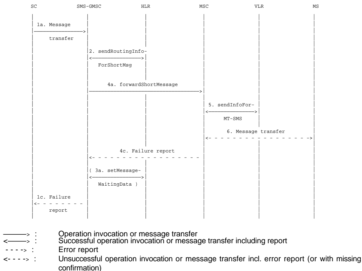
Figure 03.40/15f): Short message transfer attempt failing due to erroneous message transfer on the radio path.
