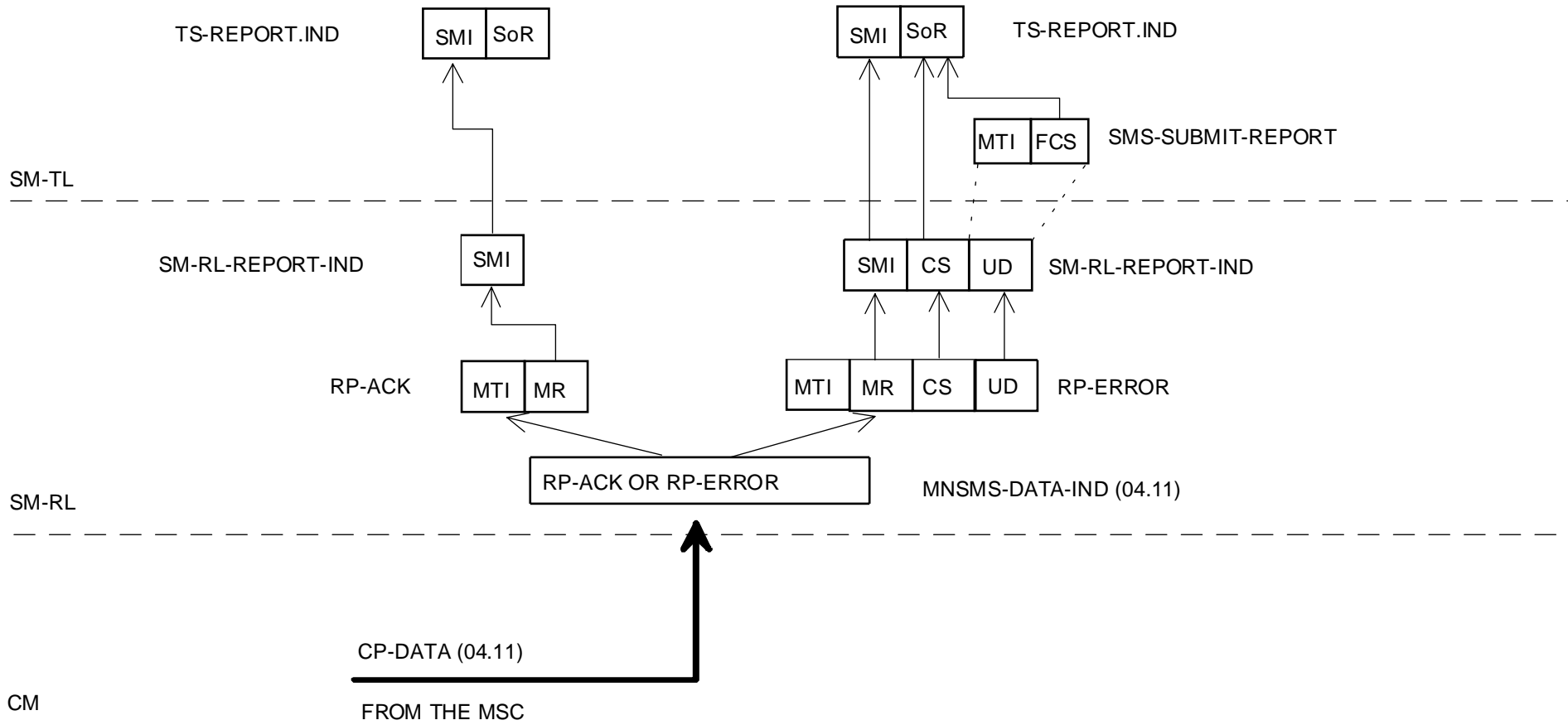
Figure 4.3: Acknowledgement in the MO case
