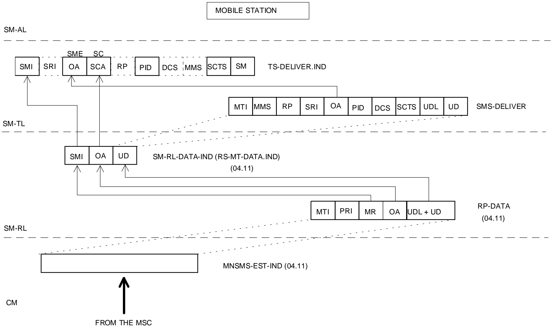
Figure 1.4: Mobile terminated short message
