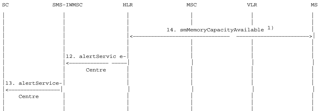
Figure 03.40/20b: The alert procedure when the MS becomes reachable, MNRF is set and MCEF is set.
