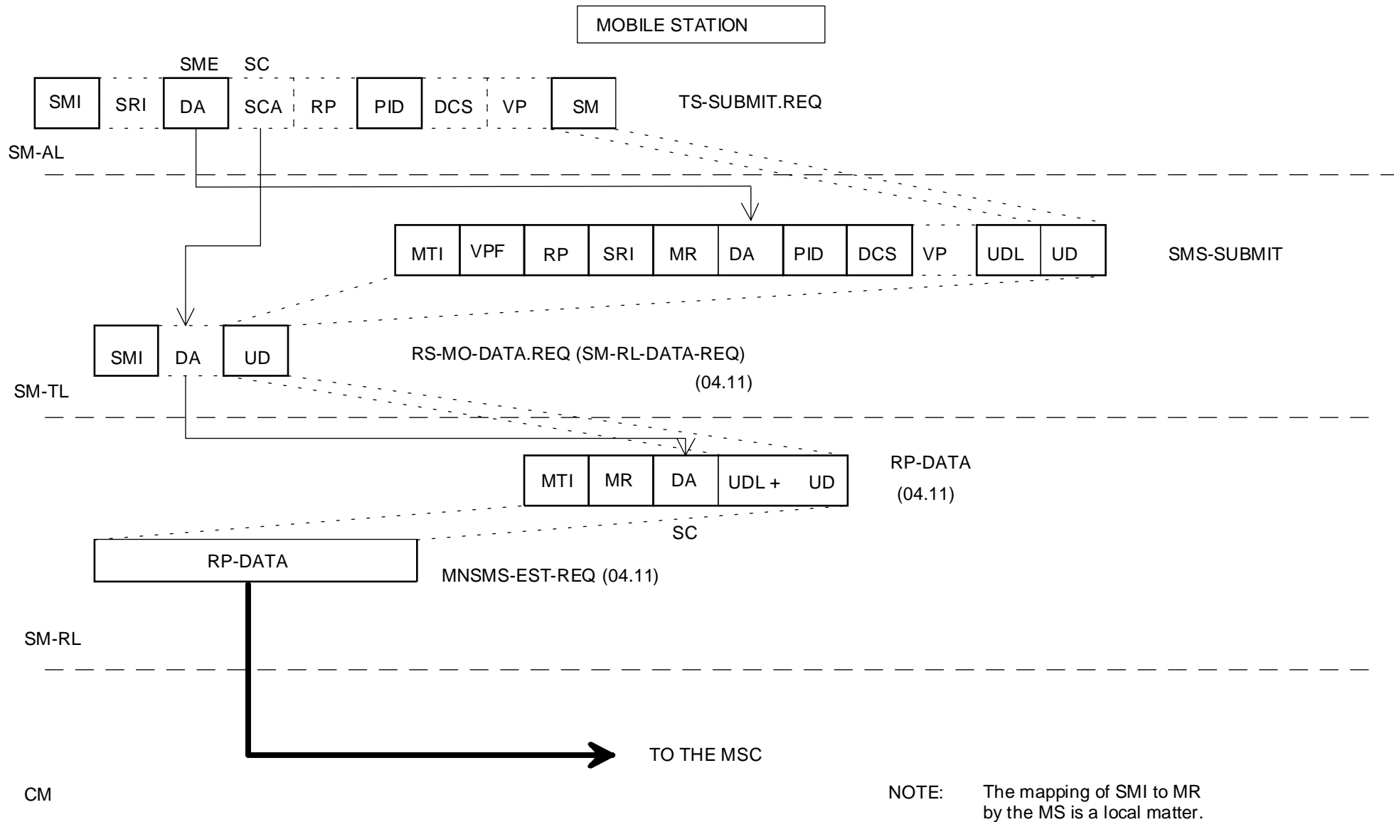
Figure 3.1: Mobile originated short message
