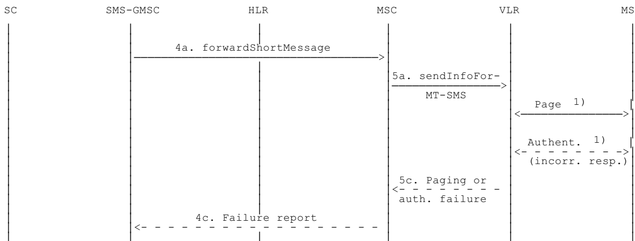
Figure 03.40/16c) 'Send information for MT SMS' procedure; erroneous case: Absent subscriber (e.g. no paging response).
