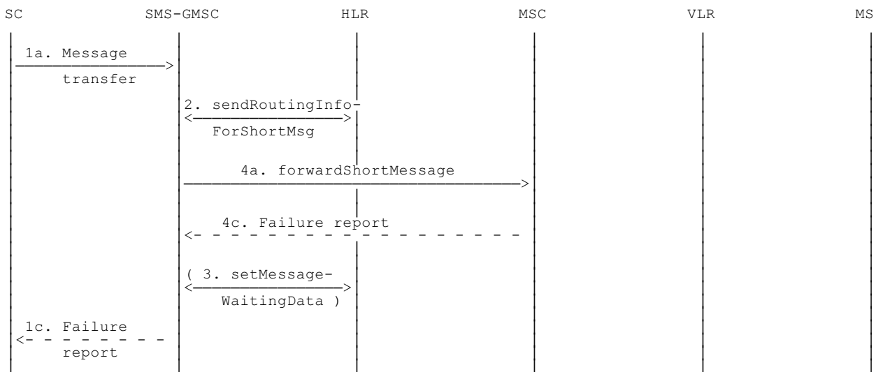
Figure 03.40/15c) Short message transfer attempt failing due to negative outcome of HLR information retrieval.
