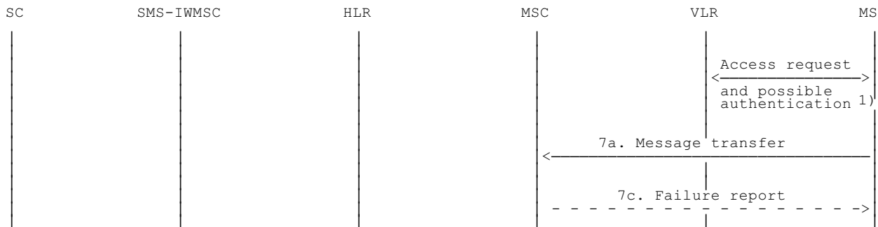
Figure 03.40/18a) Successful short message transfer attempt.
