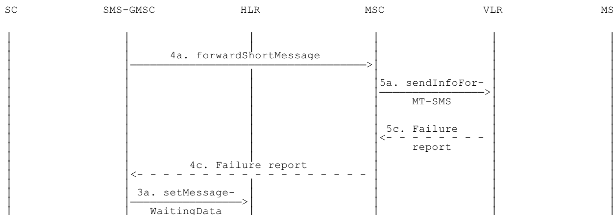
Figure 03.40/16a) 'Send information for MT SMS' procedure; error free case.
