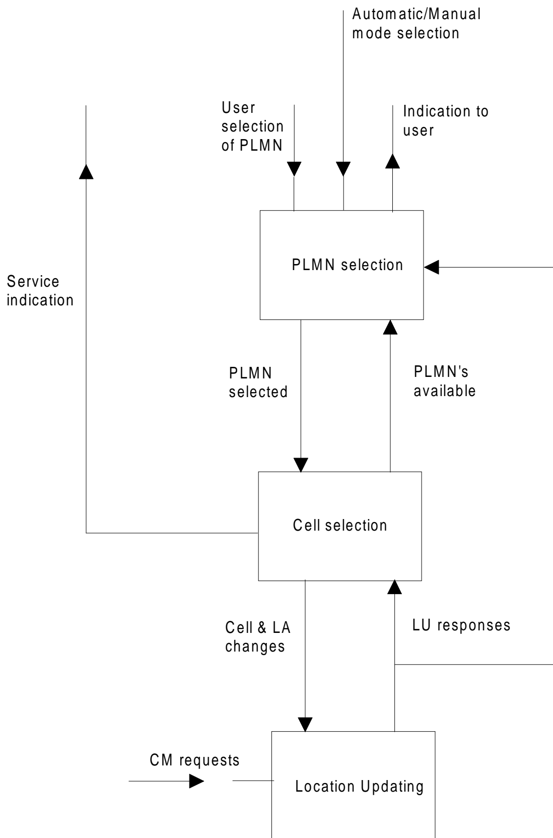
Figure 1: Overall Idle Mode process
