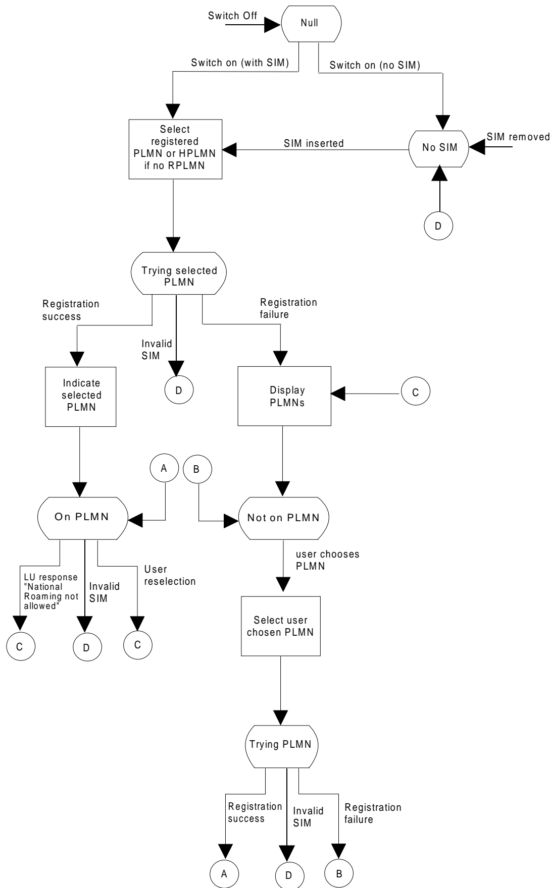
Figure 2b: PLMN Selection State diagram (manual mode)
